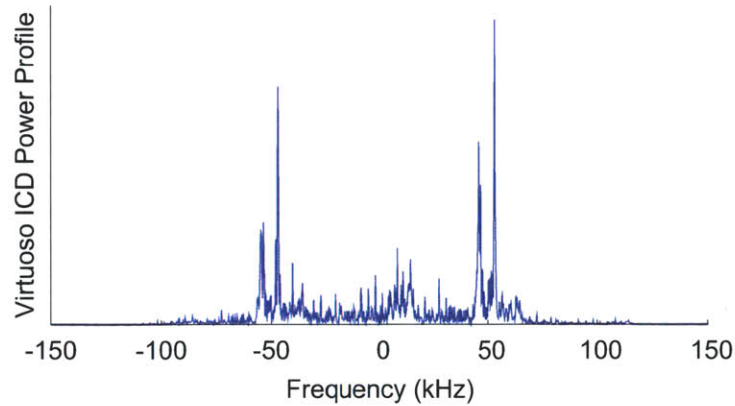
Figure 7-2: Frequency profile of IMD signal: The frequency profile of the FSK signal captured from the Virtuoso cardiac defibrillator shows that most of the energy is concentrated around \pm 50 KHz.
