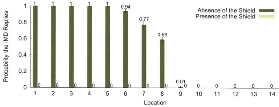
Figure 10-5: Probability the IMD transmits in reply to an active adversary: The figure shows that, in the absence of the shield, triggering an IMD to transmit and deplete its battery using off-the-shelf IMD programmer succeeds with high probability. In contrast, in the presence of the shield such attacks fail.
