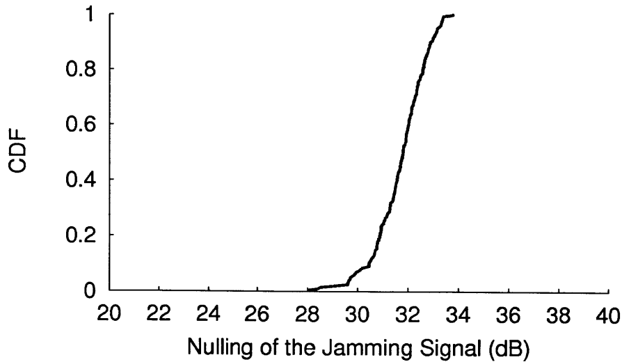
Figure 10-1: Antenna cancellation: The antidote signal reduces the jamming signal on average by 32 dB.
