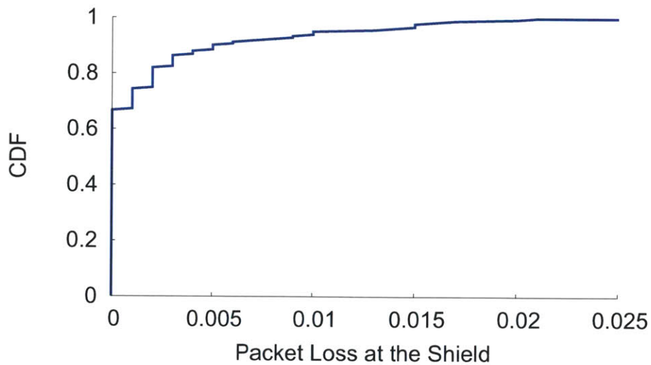
Figure 10-4: Packet Loss at the shield : When the shield is jamming, it experiences an average packet loss rate of only 0.2% when receiving the IMD’s packets. We conclude that the shield can reliably decode the IMD’s transmissions despite jamming.
