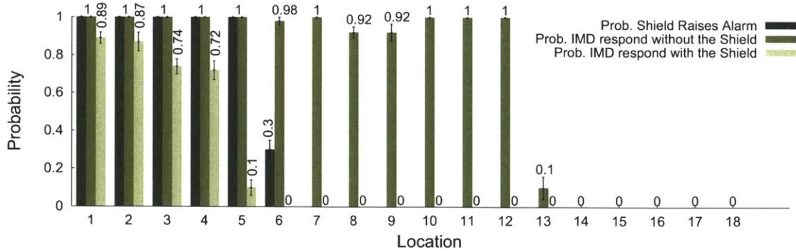
Figure 10-7: Probability the IMD changes therapy in reply to a high power active adversary: When the shield is off (absent), an adversary transmitting at 100 times the shield’s power can change the IMD’s therapy parameters even from non-line-of-sight locations up to 27 meters away. However, when the shield is on (present), the adversary is successful only from line-of-sight locations less than 5 meters away, and the shield raises an alarm.
