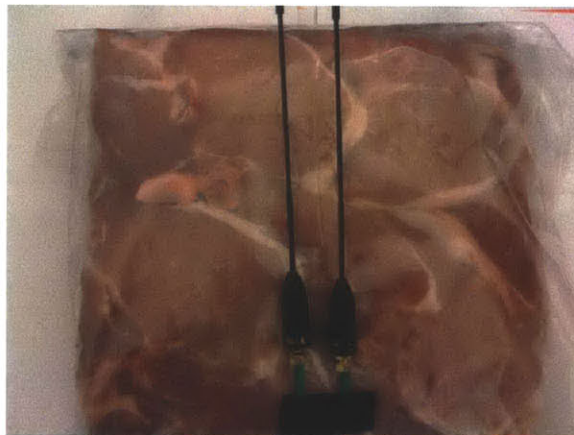
Figure 9-2: Simulating an human body environment : Each IMD is implanted beneath 1 cm of bacon, with 4 cm of 85% lean ground beef packed underneath. We placed the shield's antennas next to the IMD on the bacon's surface to simulate a necklace
