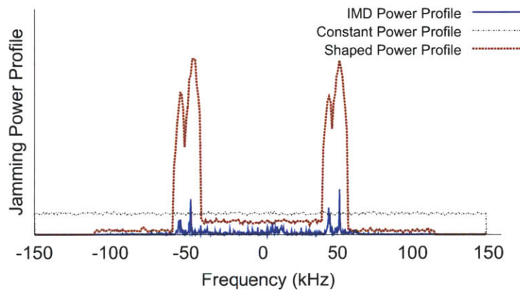
Figure 7-3: Shaping the profile of the jamming signal: The frequency profile of the jamming signal is shaped to match that of the IMD allows the shield to focus its jamming power on the frequencies that matter for decoding, as opposed to jamming across the entire 300 KHz channel. Note: The IMD's power profile in blue is scaled up for clarity.
