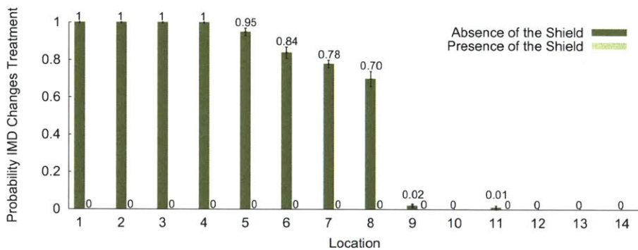
Figure 10-6: Probability the IMD changes therapy in reply to an active adversary: When the shield is off (absent), an adversary who uses an off-the-shelf IMD programmer to send unauthorized commands (in this case, to modify therapy parameters) succeeds with high probability. When the shield is on (present), it materially decreases the adversary’s ability to control the IMD.
