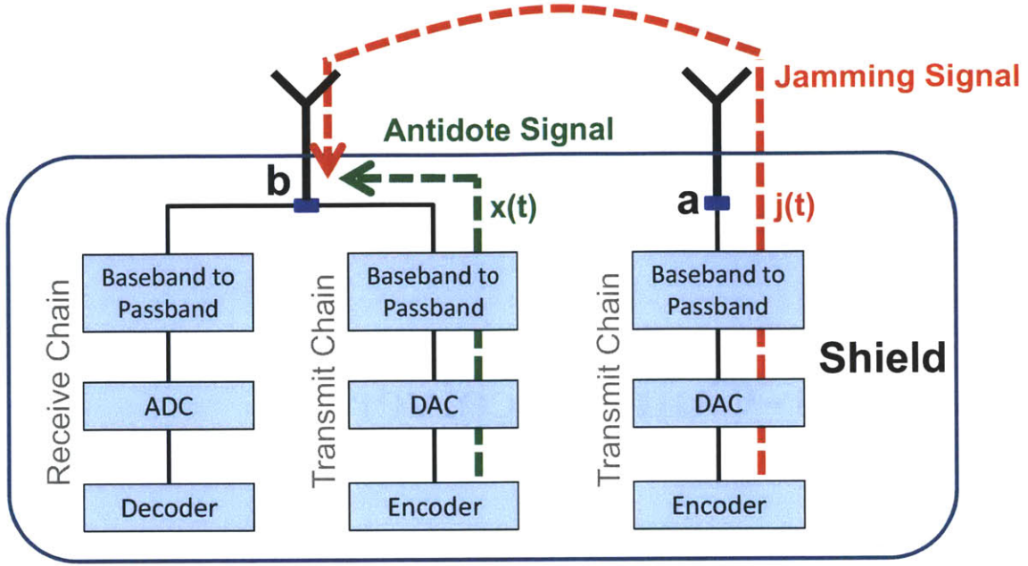
Figure 6-1: Jammer-cum-Receiver Design: The design uses 2 antennas: a jamming antenna that transmits the jamming signal and a receive antenna. The receive antenna is connected to both a transmit and receive chain. The antidote signal is transmitted from the transmit chain to cancel out the jamming signal in the receive chain.
