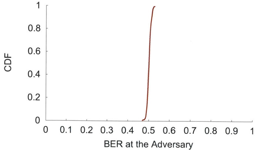
Figure 10-3: BER at the eavesdropper: CDF of an eavesdropper’s BER over all eavesdropper locations in Fig. 9-3. At all locations, the eavesdropper’s BER is nearly 50%, which makes its decoding task no more successful than random guessing. The low variance in the CDF shows that an eavesdropper’s BER is independent of its location.
