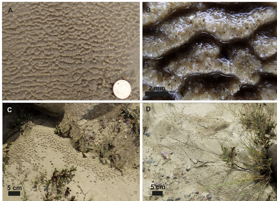
Fig. 14. Modern “Kinneyia” wrinkles in the absence of microbial mats. (a,b) “Kinneyia”-like form developing in very shallow (<2 mm) water in ponded water adjacent to a small channel on a beach at low tide. Wind is transporting sediment in arrowed direction and ridges of “Kinneyia” accrete above level of water by adhesion from water tension, retaining steep sides. Holkham, Norfolk, England. (c,d) Patches of “Kinneyia”-type form within clayey silt on the dried floor of an ephemeral stream in an endorheic basin, near Sarytobe, Kazakhstan.
