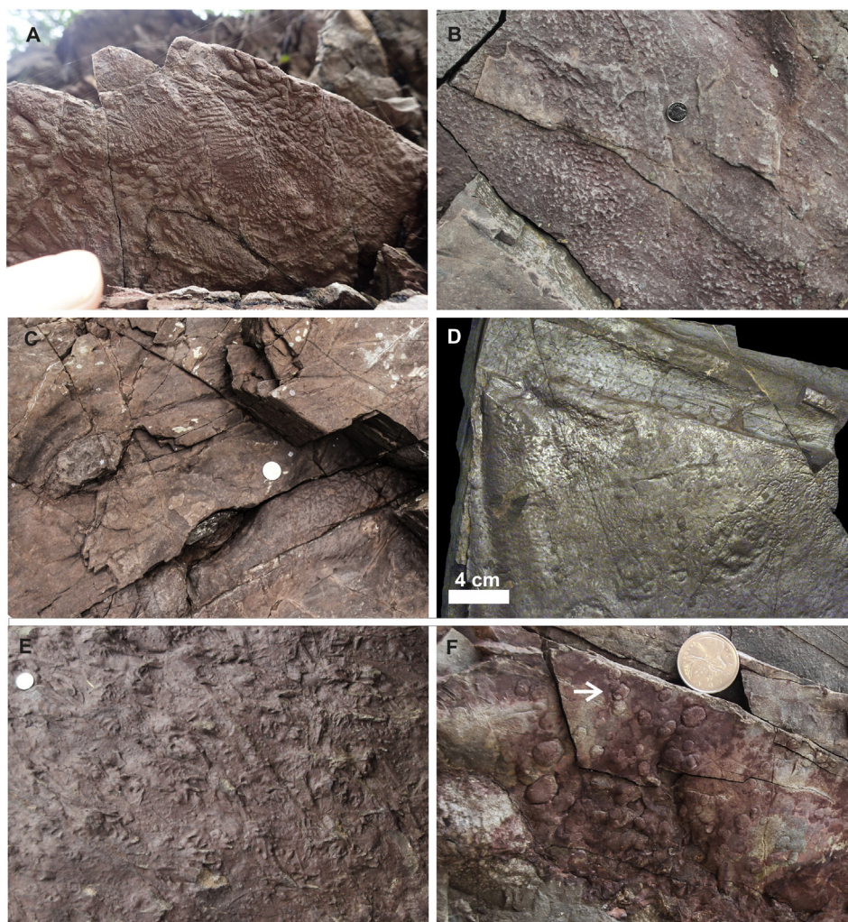
Fig. 18. Diverse sedimentary surface textures within Pennsylvanian alluvium of the Tynemouth Creek Formation, New Brunswick, Canada. (a) Oriented wrinkles on base of ephemerally channel sandstone. Category Ba. (b) Wrinkles resembling poorly preserved adhesion warts. Category Ab. Diameter of coin is 21 mm. (c) Patches of wrinkles associated with surface colonization by standing Calamites . Category ab. Diameter of coin is 24 mm. (d) Wrinkles and bubble-like structures in abandoned channel facies, associated with well-preserved Cordaites fronds. Category Ba. (e) Wrinkles and bubbles on layer associated with tetrapod tracks, but no good thin section evidence. Category ab. Diameter of coin is 24 mm. (f) Bubble like marks in positive hyporelief in abandoned channel facies that bear a strong resemblance to casts of drip marks. Category Ab. Diameter of coin is 24 mm.
