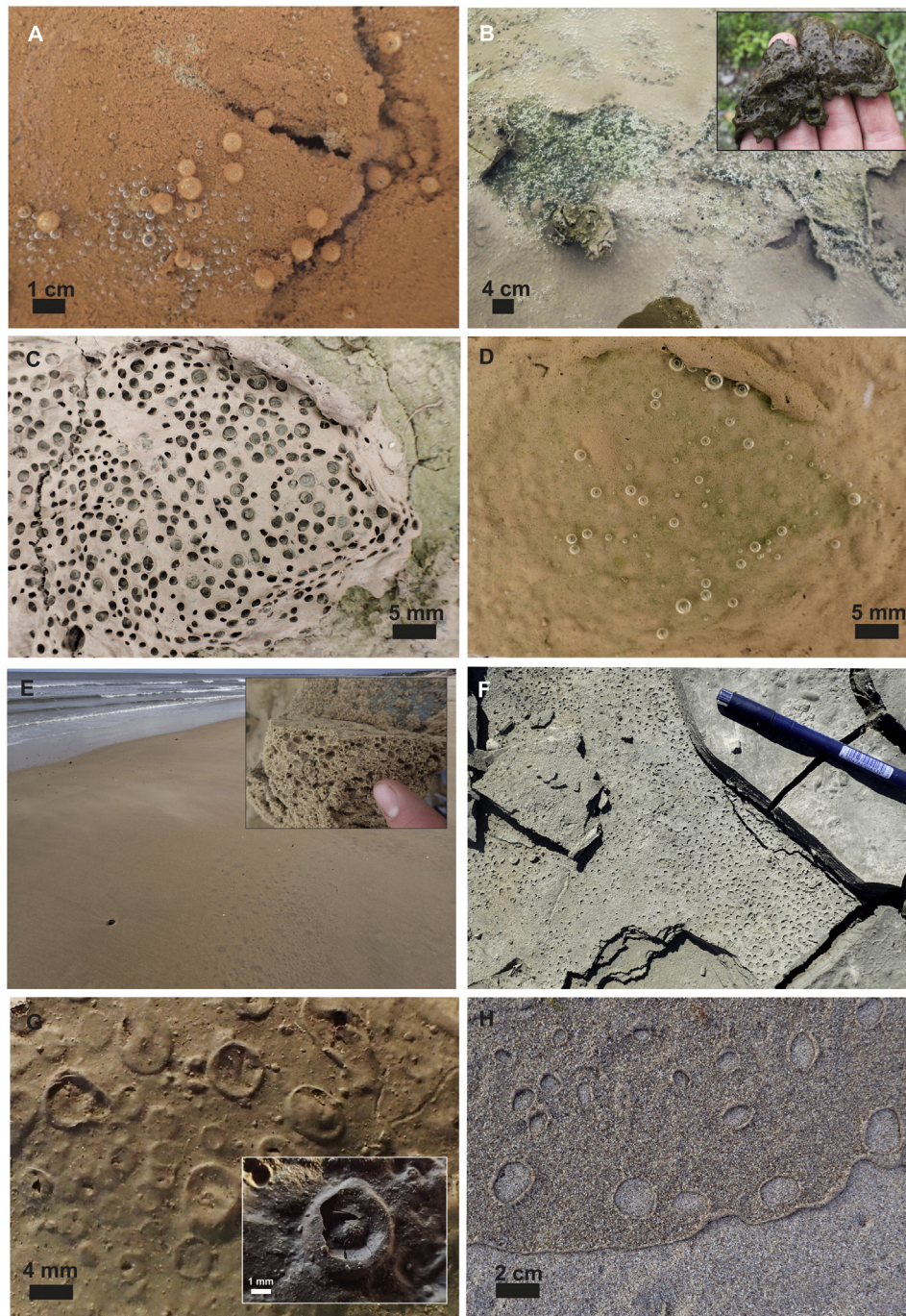
Fig. 10. Modern examples of the contribution of air and gas to the formation of sedimentary surface textures in both the presence and absence of microbial mats. (a) Respiring microbial community in a stagnant puddle on top of a coastal landslip. Larger bubbles are coated with both microbial matter and sediment grains and are arranged around a bird footprint. Hastings, Sussex, England. (b) Microbial mats developed in roadside puddle, actively respiring bubbles of oxygen that may burst inside the EPS-rich sediment, leading to prominent bubbled texture (inset). Bisk, Siberia, Russia. (c–d) Dormant microbial mat in dried freshwater puddle, showing temporary preservation of bubble texture. Second image shows same mat healed and respiring 3 days later, after heavy rain has refilled puddle but with no addition of sediment. Cape John, Nova Scotia, Canada. (e) Air escape bubbles developing near strandline on beach during falling tide, Bamburgh, Northumberland, England. Inset: subsurface structure of bubble sand developed during falling tide, Scolt Head Island, Norfolk, England. (f) Air escape bubbles formed beneath clay cap of a desiccation crack, Mont Saint-Michel Bay, Normandy, France. Length of pen is 136 mm. (g) Clay and particulate coal film on the surface of a dried puddle in a tyre rut on an access track of an opencast coal mine. As finest sediment settles out of suspension, trapped air forms bubbles in surface veneer as the puddle dries and desiccates. Although clearly abiotic, certain burst bubbles (e.g., inset) bear a resemblance to impressions previously interpreted as fossils (e.g., Intrites punctatus (sensu McLroy et al., 2005) from Ediacaran strata). Bachat, Siberia, Russia. (h) Patterns formed by swash on a beach where swashing water was laden with sediment. Sediment was transported by the film of water but not within the air bubbles that were trapped in the swash by the breaking wave, resulting in an adhesive sediment veneer with characteristic holes reflecting bubble locations. Texture was formed at high tide and persisted on the beach for a full tidal cycle. Sandwood Bay, Sutherland, Scotland.
