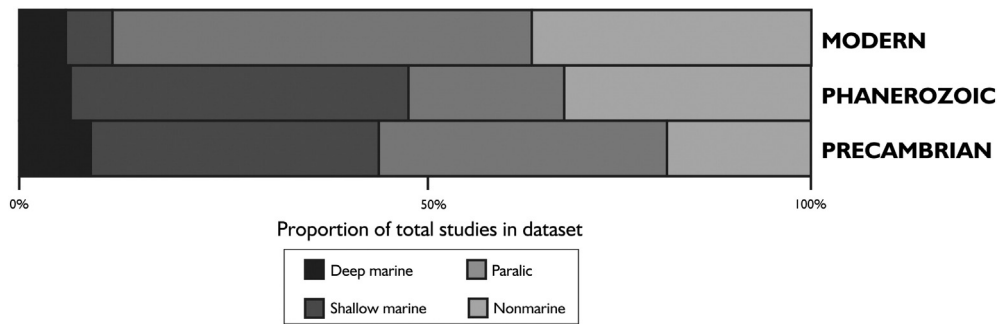
Fig. 4. Environmental distribution of recorded MISS (as a proportion of total studies) for the Precambrian, Phanerozoic and Recent.
