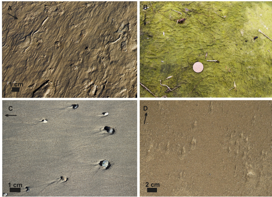
Fig. 12. Sedimentary surface textures arising from flow and shear in modern sediments: arrows indicate flow direction. (a) Transverse wrinkling of top of supratidal mat resulting from wind. Meighen Island, Nunavut, Canada. (b) Wrinkling in intertidal algal mat resulting from draining of tide from margins of salt marsh. Alnmouth, Northumberland, England. Diameter of coin is 23 mm. (c) Cusped forms developing in the lee of shell material during ebb tide. Ostend, Belgium. (d) Setulfs developing through wind erosion (and associated with adhesion ripples in Fig. 7). Holkham, Norfolk, England.
