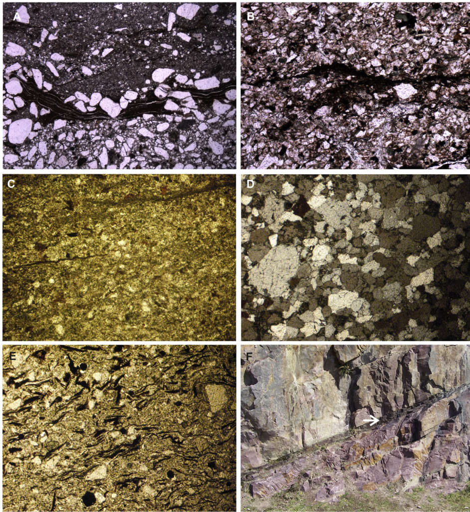
Fig. 16. Thin section images of suspected MISS. (a) Thick organic layers draped over mounds of large quartz grains with twisted and recumbent pieces, implying original cohesion, and sand grains apparently imbedded within the organic layer. Mississippian Horton Bluff Formation, Blue Beach, Nova Scotia, Canada (see Fig. 1c for larger scale structure). Field of view = 2.5 mm. (b) Dark organic lenses splitting and fraying, but not exhibiting lateral continuity. Pennsylvanian Tynemouth Creek Formation, New Brunswick, Canada (see Fig. 18e). Field of view = 2.5 mm. (c) Thin section of Arumberia, cut perpendicular to bedding, with thin wisps of organic material. Cambro-Ordovician Port Lazo Formation, Brittany, France (Fig. 1t). Field of view = 3.1 mm. (d) Thin section of “Kinneyia” wrinkles, cut perpendicular to bedding, exhibiting no evidence for organic material. Silurian Tumblagooda Formation, Western Australia (Fig. 1x). Field of view = 3.1 mm. (e-f) Thin section with abundant organic microbial mat fragments that comes from mudstone horizon in 16f, where there is a total absence of sedimentary surface texture or any other macroscopic features that would suggest a microbial presence. Cambro-Ordovician Frehel Formation (correlative with Port Lazo Formation in 16d), Brittany, France.
