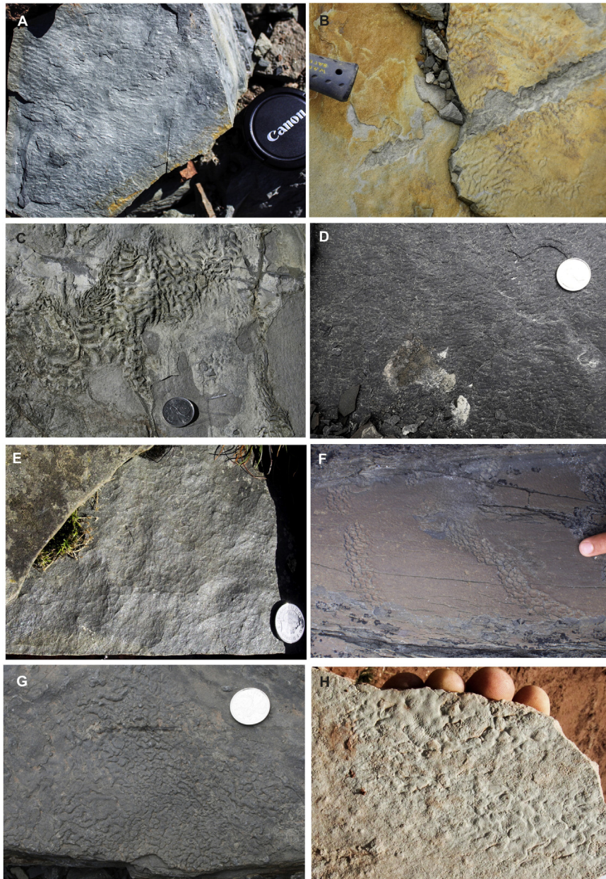
Fig. 1. Examples of sedimentary surface textures in the rock record. (a) Transverse wrinkles on the base of a mudstone bed. Siluro-Devonian coastal alluvial plain facies, Clam Bank Formation, Clam Bank Cove, Newfoundland, Canada. Diameter of camera lens cap is 58 mm. (b) Patch of curving transverse wrinkles on top of a siltstone bed. Late Devonian back-barrier and sabkha facies, Evieux Formation, Hoyoux, Belgium. Width of hammer shaft is 35 mm. (c) Recumbently oriented wrinkles on a mudstone bedding plane. Mississippian tidal facies, Horton Bluff Formation, Blue Beach, Nova Scotia, Canada. Diameter of coin is 24 mm. (d) Transverse wrinkles within fine-grained sandstones deposited on a storm-dominated shelf. Silurian (Llandovery) Ross Brook Formation, Arisaig, Nova Scotia, Canada. Diameter of coin is 24 mm. (e) Reticulate markings on top of siltstone. Neoproterozoic lacustrine facies of the Diabaig Formation, Badenscallie, Scotland. Diameter of coin is 25 mm. (f) Trains of reticulate ridges on top of siltstone. Ediacaran deep-marine facies of the Trepassey Formation, Mistaken Point Ecological Reserve, Newfoundland, Canada. (g) Overlapping transverse ridges and mounds on top of very fine sandstone bed. Pennsylvanian alluvial facies, Tynemouth Creek Formation, St. Martin's, New Brunswick, Canada. Diameter of coin is 24 mm. (h) Cusperate inverted mounds on base of siltstone, overprinted with very fine transverse wrinkles. Early Triassic playa lake facies, Aylesbeare Mudstone Formation, Chiselbury Bay, Devon, England. (i) Aristophycus branching structure in convex relief on top of coarse sandstone bed. Cambro-Ordovician braided fluvial channel facies, Frehel Formation, Erquy, Brittany, France. Length of pen is 136 mm. (j) Convex blister structures and reticulate mineralization on top of mudstone. Early Permian alluvial facies, Kildare Capes Formation, Prince Edward Island, Canada. Diameter of coin is 24 mm. (k) Bubble-like texture on upper surface of sandstone bed. Early Permian alluvial facies, Kildare Capes Formation, Prince Edward Island, Canada. Diameter of coin is 24 mm. (l) Craters of different dimensions, attributable to raindrop impact impressions, on upper surface with desiccation cracks. Middle Devonian alluvial facies of the Catskill Formation, New York, United States. Diameter of coin is 24 mm. (m) Spindle-shaped "synaeresis" cracks cross-cutting top of Rosselia trace fossil. Early Triassic shallow-marine facies, Newport Formation, Royal National Park, New South Wales, Australia. Diameter of coin is 29 mm. (n) "Synaeresis" cracks in association with a variety of small infaunal burrows, preserved on the base of a fine sandstone bed. Late Mississippian tidal facies, Alston Formation, Howick, Northumberland, England. (o) Sinuose branching sand crack within sandstone wave-ripple trough, possibly a poorly-developed instance of Manhuriophycus. Late Mississippian deltaic facies, Alston Formation, Taythes Gill, Cumbria, England. Diameter of coin is 27 mm. (p) Setulfs in convex relief on top of fine-grained sandstone. Silurian coastal alluvial facies, Tumblagooda Sandstone, Kalbarri, Western Australia. Diameter of coin is 24 mm. (q) Palimpsested millimetre-scale ripples oblique to main ripple crests, plus looping grazing trails. Early Mississippian tidal facies of the Horton Bluff Formation, Blue Beach, Nova Scotia, Canada. Length of pen is 136 mm. (r) Ornamented ripples on the base of a sandstone. Ediacaran emergent coastal facies of the Bonney Sandstone, Flinders Ranges, South Australia. (s) Cusperate forms on top of very fine grained sandstone. Early Pennsylvanian alluvial facies of the Tynemouth Creek Formation, New Brunswick, Canada. (t) Arumberia fabric. Cambro-Ordovician tidal facies of the Port Lazo Formation, Brehec, Brittany, France. Diameter of coin is 23 mm. (u) Pitted texture associated with Arumberia fabric. Cambro-Ordovician tidal facies of the Port Lazo Formation, Brehec, Brittany, France. Diameter of coin is 23 mm. (v) Patches of "Kinneyia"-like wrinkles and repichnial trails on bedding surface in shelfal Cambrian strata. Rozel Shale and Sandstone, Normandy, France. Diameter of coin is 22 mm. (w) "Kinneyia" texture on top of fine-grained sandstone bed. Middle Ordovician shallow-marine facies of the Stairway Sandstone Formation, Amadeus Basin, Northern Territory, Australia. (x) "Kinneyia" texture on top of fine-grained sandstone bed. Silurian coastal alluvial facies, Tumblagooda Sandstone, Kalbarri, Western Australia. Diameter of coin is 24 mm.
