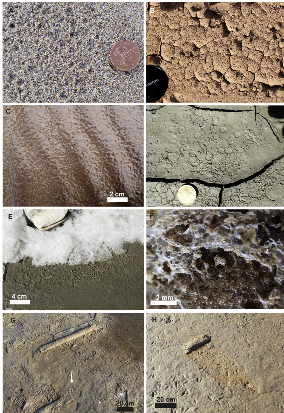
Fig. 11. Impression and sedimentary surface textures in modern sediments. (a) Fresh raindrop impressions in damp beach sand, resulting in clusters of craters separated by shared crater margins. Bamburgh, Northumberland, England. Diameter of coin is 26 mm. (b) Discrete raindrop impressions preserved in desiccated mud on floor of ephemeral stream. Boom Canyon, Kyrgyzstan. Diameter of camera lens cap is 62 mm. (c) Rain impact microtopography (R.I.M.) developed on wet sand on top of intertidal ripples immediately after heavy rain shower — note how R.I.M. blankets ripples on all sides. Bay of Fundy, Five Islands, Nova Scotia, Canada. (d) Drip impressions (and invertebrate trails) formed 2 m below a bridge from coalesced drops of water — note flattened discoidal shape and larger size than rain drop imprints. Mont Saint-Michel Bay, Normandy, France. Diameter of coin is 23 mm. (e) Wrinkle-like impressions in sand resulting from frozen beach foam. Clam Harbour, Nova Scotia, Canada. (f) Close-up of patch of organic-rich foam on tidal flat — although individual sediment grains are entrained in foam, there is little imparting of texture to the underlying sediment. Stiffkey Marshes, Norfolk, England. (g–h) Human and bird footprints on a supratidal algal mat in the High Arctic. Wind has created roll-up structures in algal mat, leaving patches of bare sediment. Where footprints are marked in bare sediment (black arrow) definition is greater than where they rest on mat (white arrow). However, mats appear to increase preservation potential of partial footprints (h). Meighen Island, Nunavut, Canada.
