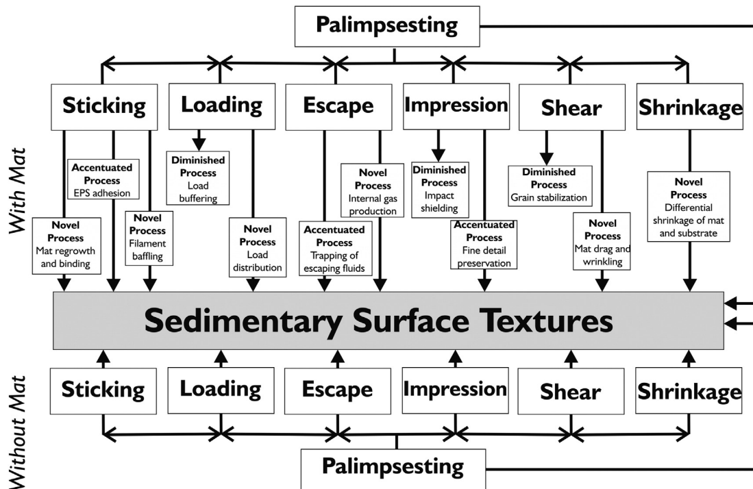
Fig. 5. Pathways involved in the creation of sedimentary surface textures, both in the presence and absence of MISS. The presence of a microbial mat may promote accentuated formation of a texture that would form on a naked substrate, diminish the formation of a texture, or result in a novel texture that could not form in the absence of a mat. Each of the illustrated pathways may be expected to result in a discrete texture for a given set of constants (e.g., grain-size, rate and intensity of process). Spatial and temporal variability in nature means that the diversity of potential textures is far greater than implied in this figure. In occurrences that are not actively forming, only the sedimentary surface texture itself is immediately presented, so determining the pathways involved in its formation requires inductive reasoning.
