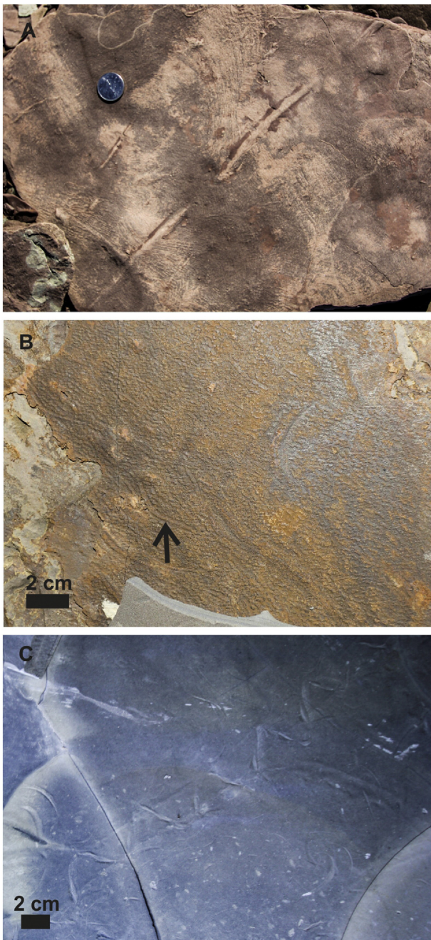
Fig. 19. Circumstantial evidence of former mats preserved as impressions due to interaction with other structures. (a) Drag mark on bedding surface, seen to distort transverse wrinkles. Result of object (likely woody debris, in context) dragging through cohesive veneer on top of sedimentary substrate. Alluvial facies of the Pennsylvanian Boss Point Formation, Little River, Nova Scotia, Canada. Diameter of coin is 24 mm. (b,c) Fish trails ( Undichna ) with different preservation depending on substrate. In (b), trails have levee margins, interpreted as indicative of fish fins dragging in ‘sludge’ of suspected microbial mat (also iron-rich and exhibiting millimetre-scale ripples and wrinkles). In (c), where the turbidite sandstone surface exhibits no sedimentary surface textures, the trails are preserved as sharp scratches without levees. Pennsylvanian Bude Formation, Cornwall, England.
