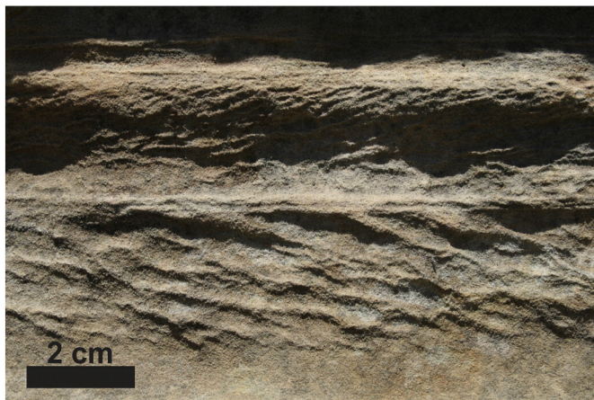
Fig. 7. Preservation potential of adhesion ripples illustrated by accretionary adhesion ripple cross-lamination in the Cambrian Wonewoc Formation, Wisconsin Dells, Wisconsin, United States. For surface expression, see Dott et al. (1986) ; their Fig. 2).
