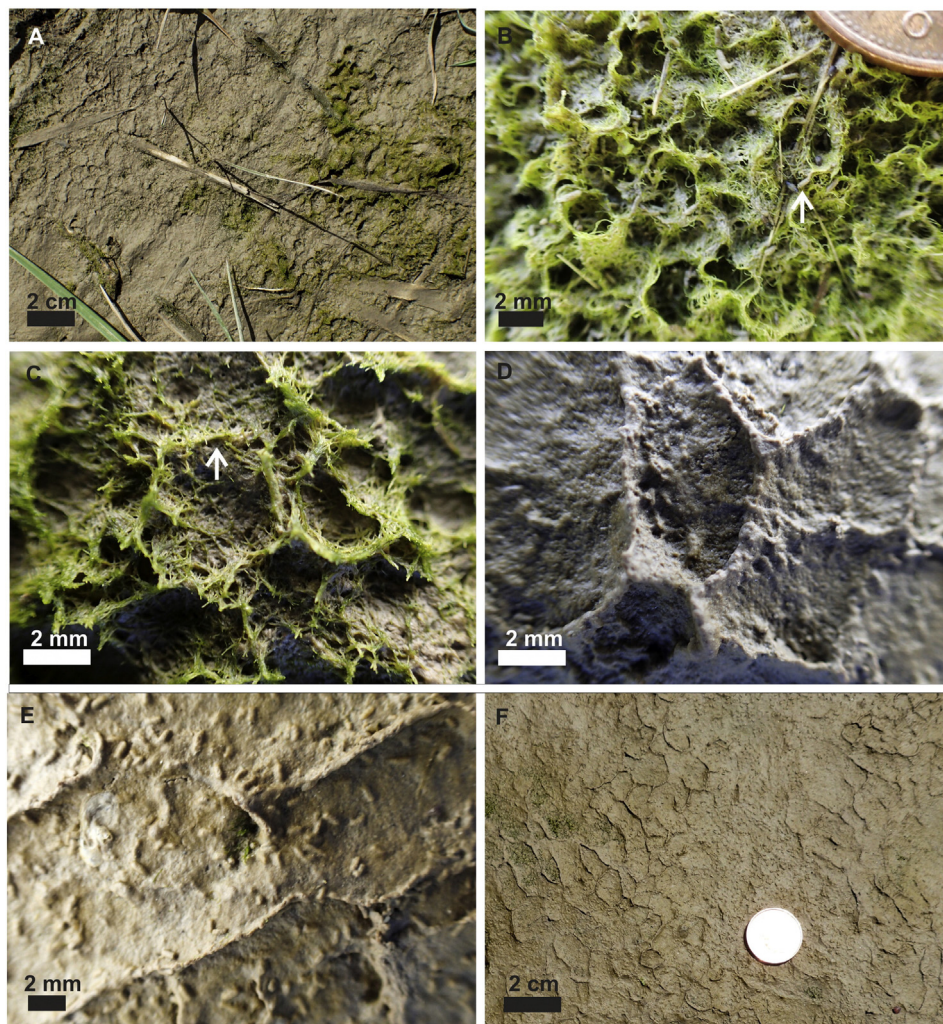
Fig. 8. Sedimentary surface textures formed by adhesion, accretion and baffling in modern sediments where microbial and algal mats are present. Examples from the tidal reaches of the River Rother, Sussex, England, at low tide. (a) Patches of filamentous algae on muddy tidal deposit. Filaments have become tangled into a reticulate pattern that is present both on the algal mats and the bare sediment. (b) Close-up image of tangling of algal filaments. Resultant 'nests' have the capacity to trap other objects, such as suspected egg case (arrowed). (c) Trapping of mud leads to collapse flattening of certain septate ridges of the reticulate structure, leading to an effective enlargement of each of the individual nests within the structure. (d) Eventual encasement of entire structure by mud, preserving only the most pronounced reticulate septae with a correspondingly larger dimension than the reticulate patterns in the algal mat itself. (e) Close-up of preserved ridges, plus mud-coated detritus (suspected egg cases as in b) trapped between them. (f) Resultant texture on now bare sediment, acting as a locus for immediate colonization by other microbial elements (to the left of the image).
