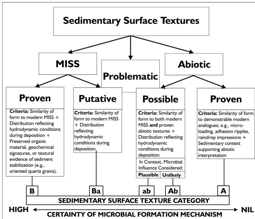
Fig. 17. Proposed umbrella classification of Sedimentary Surface Textures, incorporating true MISS as well as problematic and abiotic textures, and the shorthand approach for initial field classification.
