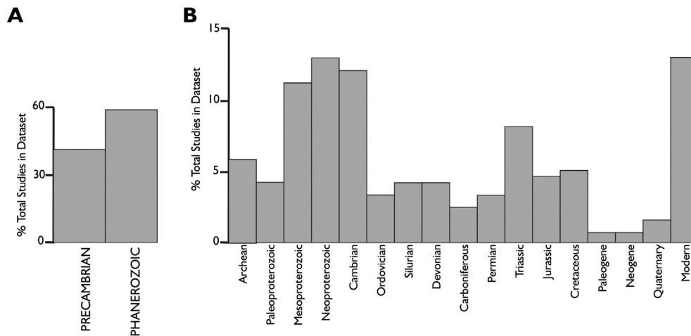
Fig. 2. Distribution of reported MISS in the global stratigraphic record, from studies listed in Table 1. (a) Proportion of MISS recorded in the Precambrian and Phanerozoic. (b) Proportional distribution by Eon (for Archean), Era (for later Precambrian) and Period (for Phanerozoic). Note that, where given age crossed two periods (e.g., Silurian–Devonian), a 0.5 value was given to each period.
