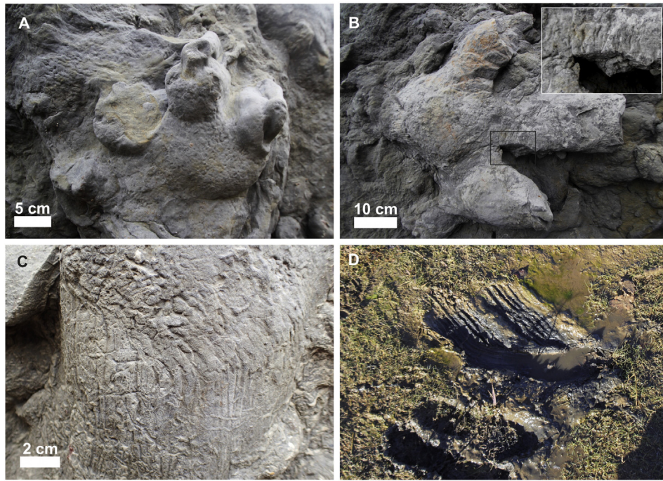
Fig. 20. Sedimentary surface textures associated with dinosaur footprints, Early Cretaceous Ashdown Formation, Fairlight Cove, Sussex, England. (a) Well-preserved iguanadont footprint with claw mark and wrinkles preserved on both base of footprint and outside of footprint. (b) Iguanadont footprint with heel slip marks and skin impressions around toe joints (inset). (c) Heel slip marks on iguanadont footprint with same dimensions as diamond shaped sedimentary surface texture internal to foot: possible skin impression. (d) Analogue for heel slip impression made by ornamental hiking boot soles on modern salt marsh, Stiffkey, Norfolk, England.
