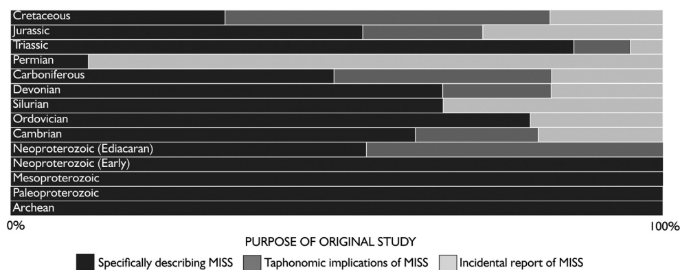
Fig. 3. Purpose of studies describing MISS for each interval, shown as a proportion of total studies (each individual reference in Table 1 considered as a discrete datapoint). Purpose divided into (a) studies where the description and interpretation of the presence of MISS was the main focus of the paper, (b) studies where the taphonomic importance of MISS was the main focus, and (c) where the presence of MISS was noted incidentally, as one sedimentary feature amongst many others.
