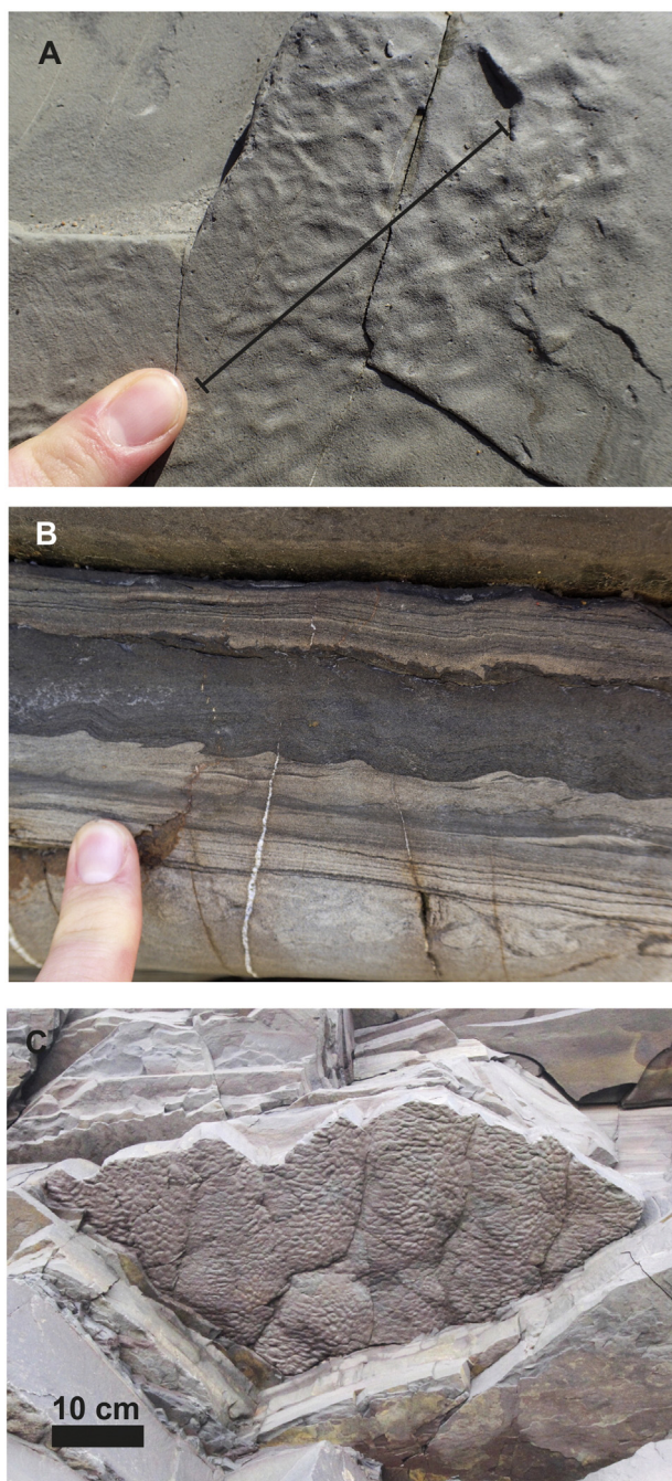
Fig. 9. Examples of wrinkles arising from loading in the Early Pennsylvanian Bude Formation, Cornwall, England. (a) Epirelief wrinkles with no discernible orientation on top of fine sandstone turbidite bed. (b) Cross-sectional view of loading in the same facies. Dimensions of load structures initially appear in excess of the wrinkle marks, but if the section were cut along the line shown in a, this would not be the case. (c) Hyporelief counterpart to load induced wrinkles on the base of an overlying bed, showing capacity for formation of inverted wrinkles on underlying beds.
