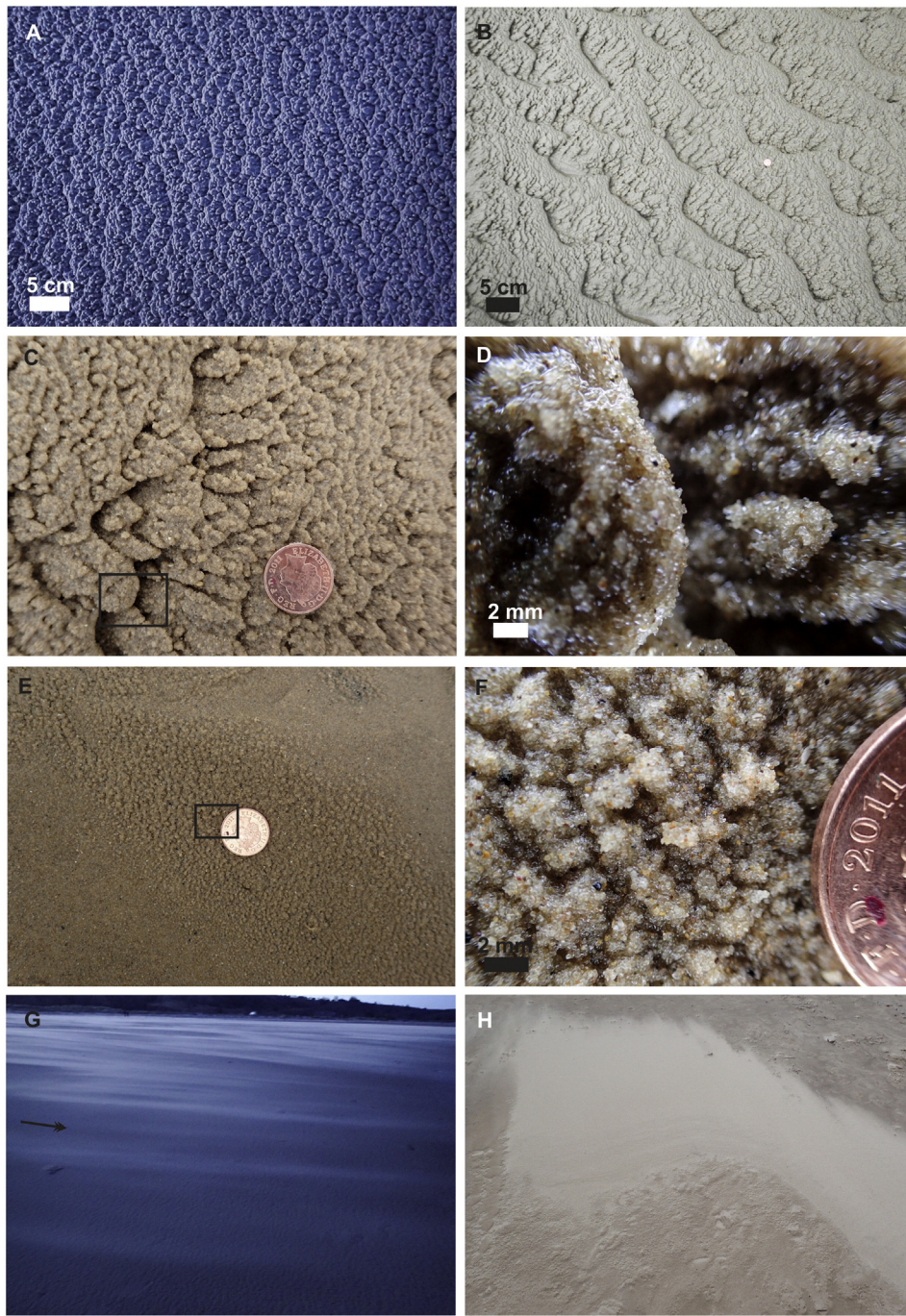
Fig. 6. Sedimentary surface textures formed by adhesion, accretion and baffling in modern sediments where microbial mats are absent. (a) Adhesion ripples with steep stoss sides (wind moving from left of image). Actively forming on wet beach sands below the high tide line during ebb tide, Alnmouth, Northumberland, England. (b) Flat topped adhesion ripples with adhesion ladder ripples forming in troughs. Actively forming in strong wind conditions as soon as water of tidal prism retreated during ebb tide, Het Zwin, Belgium. (c–d) Close-up images of stoss side of actively accreting adhesion ripples, showing extent of water tension in pores of sand and the initial adherence of wind-blown sand grains prior to their being subsumed by water tension. Actively forming on wet beach sands below the high tide at turn of ebb to flood tide, Holkham, Norfolk, England. Diameter of coin is 20 mm. (e–f) Close-up images of actively accreting adhesion warts at same locality, warts forming preferentially over ripples as they accrete on an inclined side of a drainage channel, sheltered from the wind. Diameter of coin is 20 mm. (g) Active formation of adhesion ripples as sheets of aeolian sand blow over wet beach (in direction of arrow). Movement by saltation is hindered as a proportion of grains become accumulated into stoss sides of adhesion ripples. Alnmouth, Northumberland, England. (h) Instantaneous preservation of adhesion warts. Adhesion warts formed during start of ebb tide when sand was wet. Continued drying of sand, coupled with drop in wind intensity, means that small low amplitude dune patches of dry sand now migrate slowly over previously formed adhesion warts (and footprints), offering an initial pathway towards preservation. Bamburgh, Northumberland, England. Field of view is c. 1 metre.
