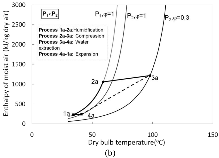
Figure 16: Varied pressure cycle. (a) Schematic diagram; (b) Psychrometric representation: humidification (1-2) followed by compression (2-3), subsequent dehumidification (3-4) and finally expansion (4-1).
