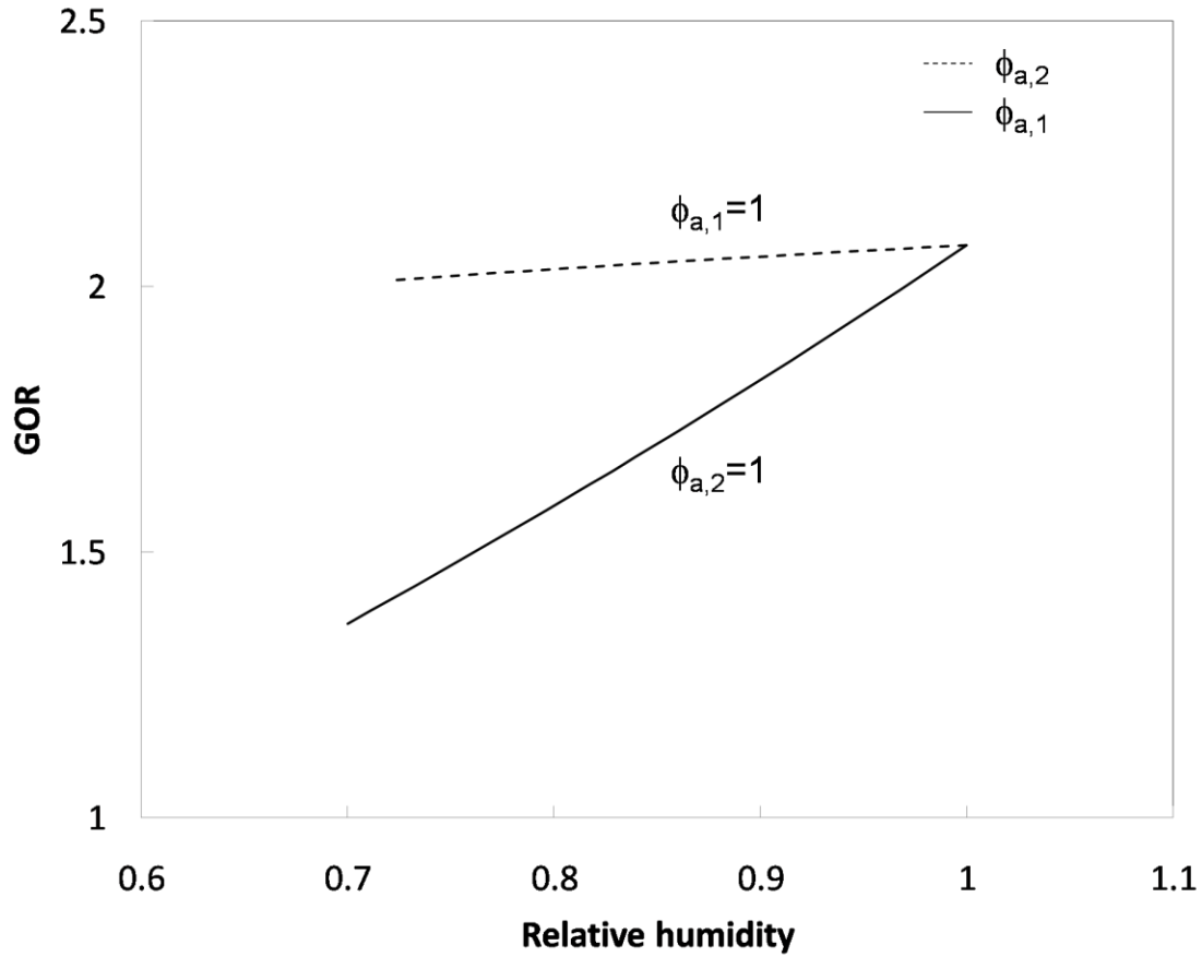
Figure 3: Effect of humidifier and dehumidifier inlet air relative humidity on water-heated CAOW cycle performance. \dot{m}_w = 0.5 kg/s; \dot{m}_{da} = 0.1 kg/s; T_{w,2} = 80^\circ\text{C} ; T_{w,0} = 35^\circ\text{C} ; \varepsilon_h = \varepsilon_d = 90\% .
