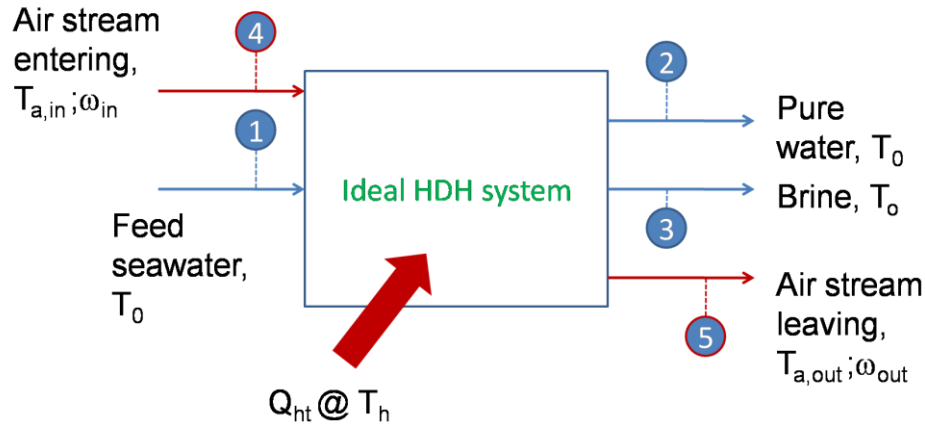
Figure 19: Schematic diagram for calculating Carnot GOR of HDH
