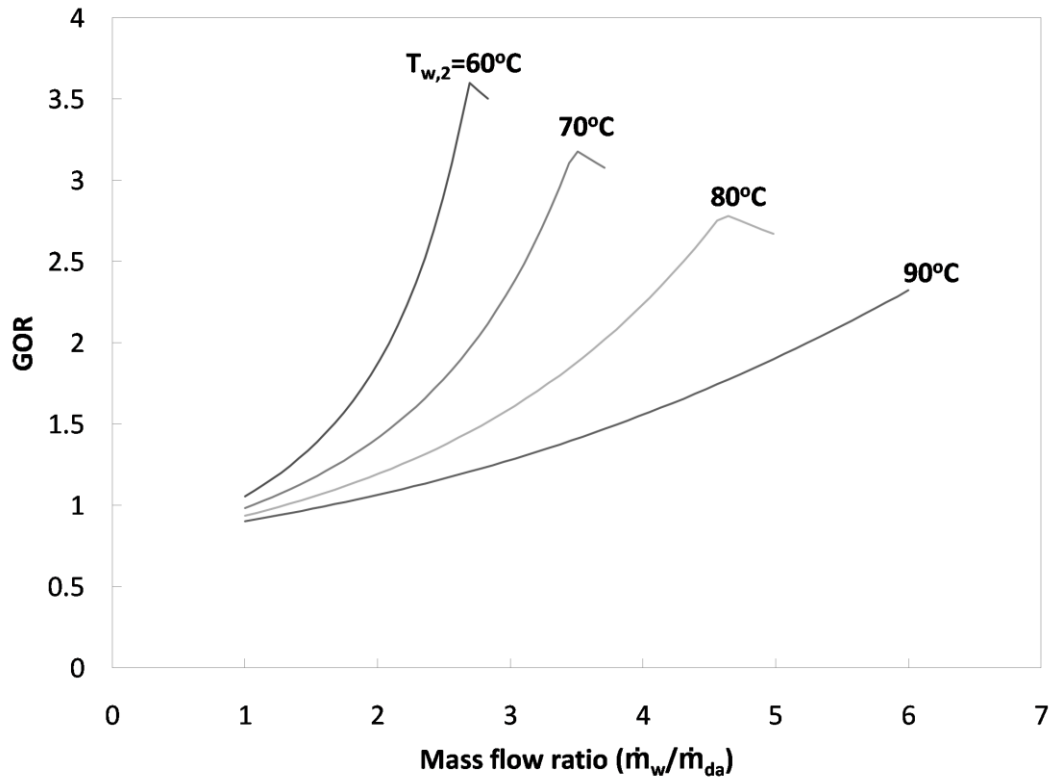
Figure 5: Effect of top temperature, T_{w,2} , on water-heated CAOW cycle performance. T_{w,0} = 35^\circ\text{C} ; \varepsilon_h = \varepsilon_d = 92\% .
