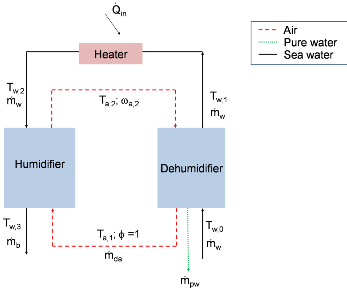
Figure 1: Water-heated CAOW HDH cycle
