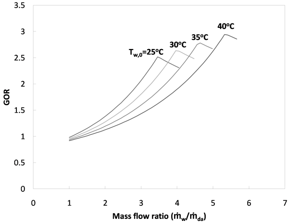
Figure 7: Effect of bottom temperature, T_{w,0} on water-heated CAOW cycle performance.
