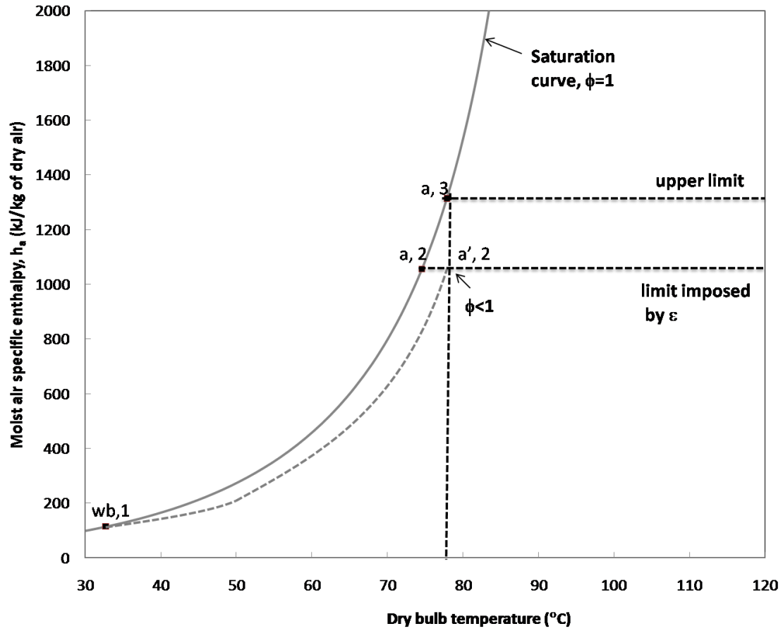
Figure 2: Psychrometric chart showing possible humidification paths and exit states; counter flow is assumed; T_{wb,1} = 31.6^{\circ}\text{C} ; T_{a,3} = T_{w,2} = 77.9^{\circ}\text{C} .
