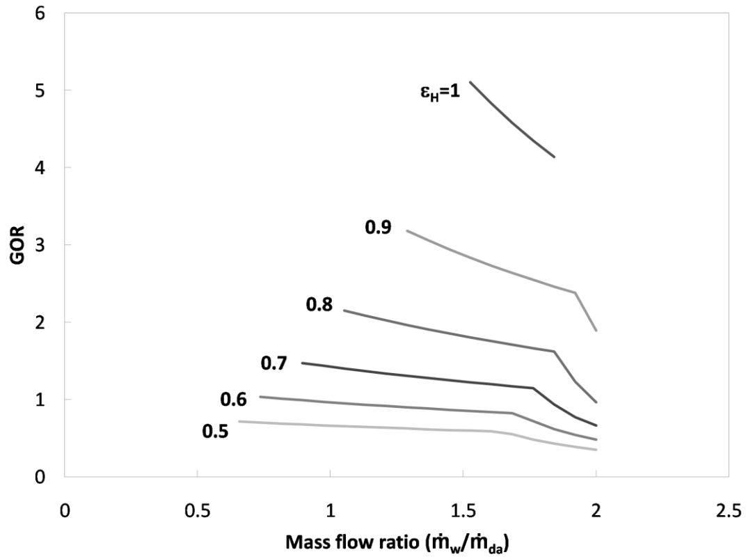
Figure 12: Effect of humidifier effectiveness on CAOW modified air-heated cycle performance T_{a,3} = 80^\circ\text{C} ; T_{w,0} = 30^\circ\text{C} ; \epsilon_d = 90\% .
