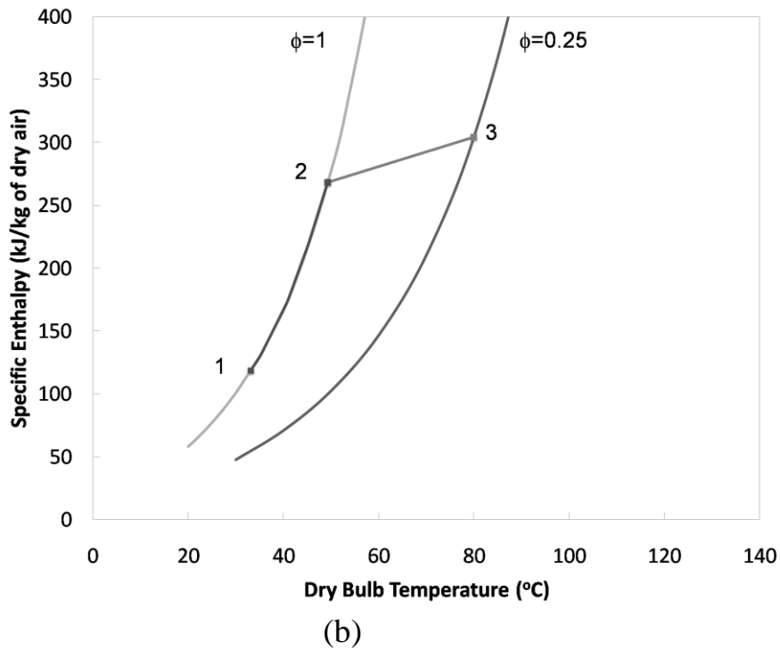
Figure 11: Modified air-heated cycle. (a) Schematic diagram; (b) Psychrometric representation: humidification (1-2) followed by heating (2-3) and subsequent dehumidification (3-1).
