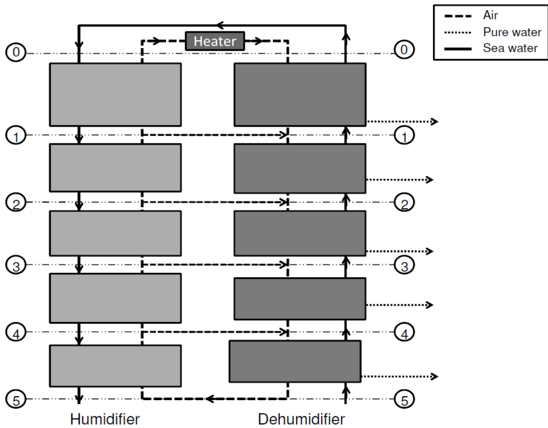
Figure 14: Multi-extraction CAOW modified air-heated cycle.
