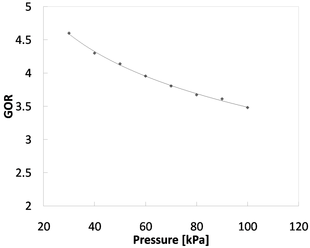
Figure 15: Effect of system pressure on performance of CAOW modified air-heated cycle; T_{a,3} = 67^{\circ}\text{C} ; T_{w,0} = 30^{\circ}\text{C} ; \varepsilon_h = \varepsilon_d = 90\% .
