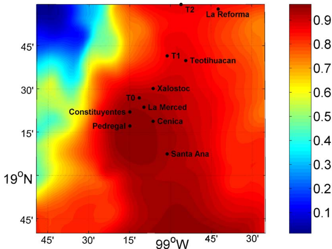
Fig. 8. Predicted episode average ground-level fractional contribution of anthropogenic V-SOA to PM_{10} total V-SOA during 13–16 April 2003.
