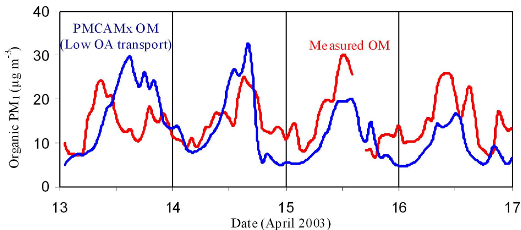
Fig. 13. Comparison of model predictions in the low boundary conditions case with hourly measurements for total PM 1 organic mass concentration taken during the MCMA campaign in 13–16 April 2003 at CENICA.
