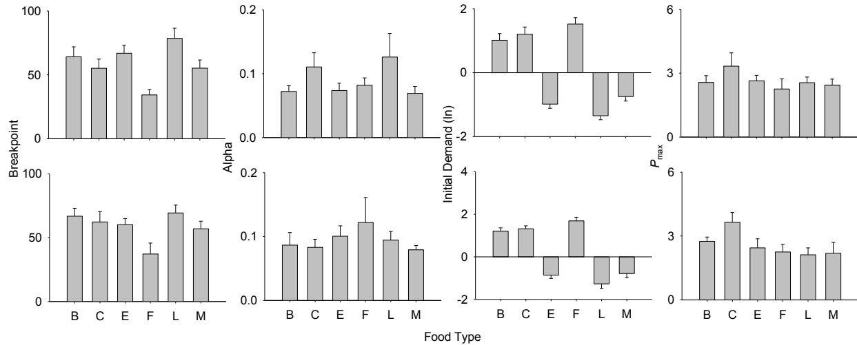
Figure 1. Estimates of alpha, initial demand ( \ln ), P_{\max} and break point (averaged across all sessions for all possums) plotted as a function of food available under the PR schedule (top panel), and plotted as a function of food available under the FR schedule (bottom panel) across possums. The standard error bars are the standard error of the mean. (B=Berries, C=Chicken, E=Egg, F=Foliage, L=Locust, and M=Mushroom).
