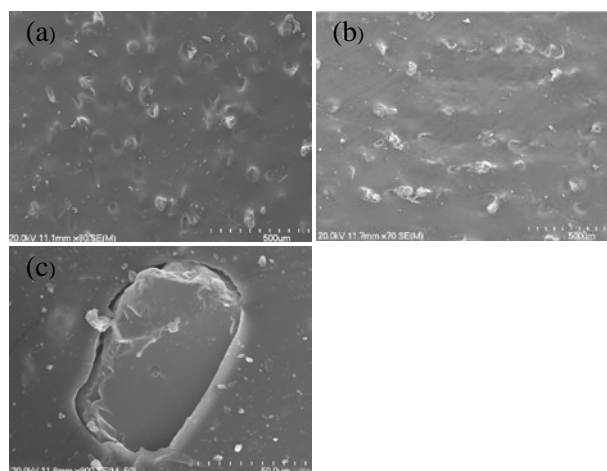
Figure 1 SEM images of MREs (a) curing in the absence of a magnetic field, (b) curing in the presence magnetic field and (c) interphase of iron sand-natural rubber matrix
