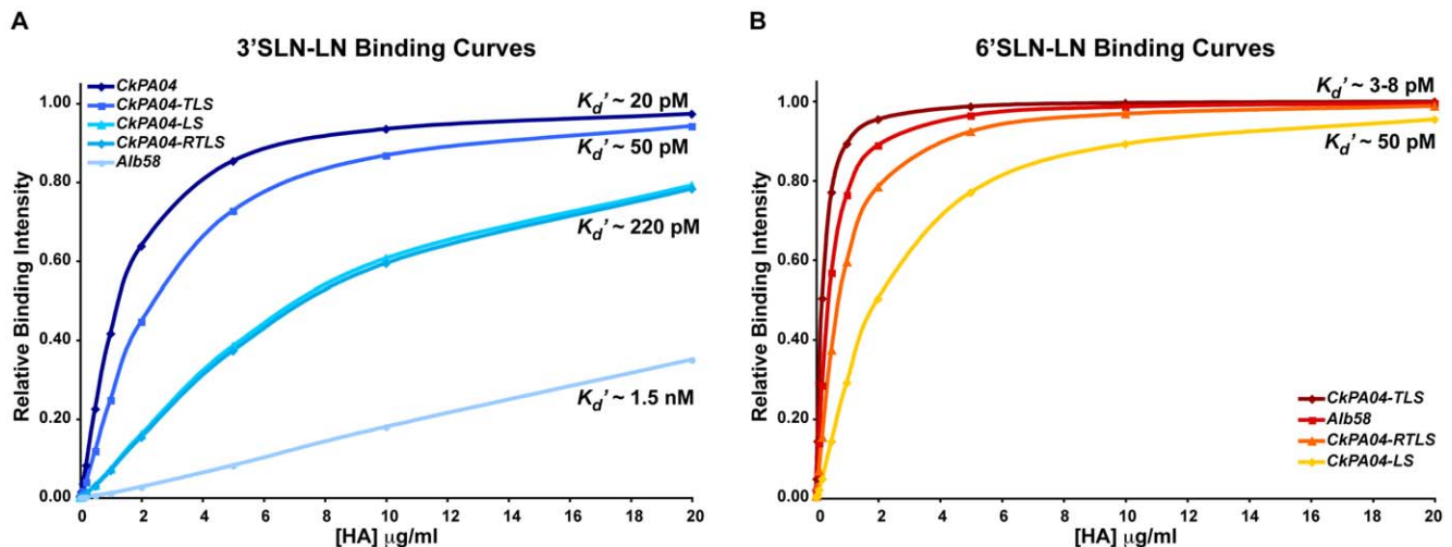
Figure 6. Glycan receptor-binding affinities of the mutant forms of CkPA04 HA. A , shows the theoretical binding curves (with the apparent binding constant K_d' ) that depict the differences in the binding affinity of the WT and mutant H2N2 HAs to the representative avian receptor (3'SLN-LN). B , shows the theoretical binding curves that depict the differences in the binding affinity of the WT and mutant H2N2 HAs to the representative human receptor (6'SLN-LN). The range of K_d' values (3–8 pM) is shown for CkPA04-TLS , Alb58 and CkPA04-RTLS that is contrasted with the K_d' value of CkPA04-LS . The binding curves were generated by fitting to the Hill equation (see Methods) and plotting the theoretically calculated fractional saturation ( y -axis) against HA concentration ( x -axis). The n value for all the binding events is around 1.3. doi:10.1371/journal.pone.0013768.g006
