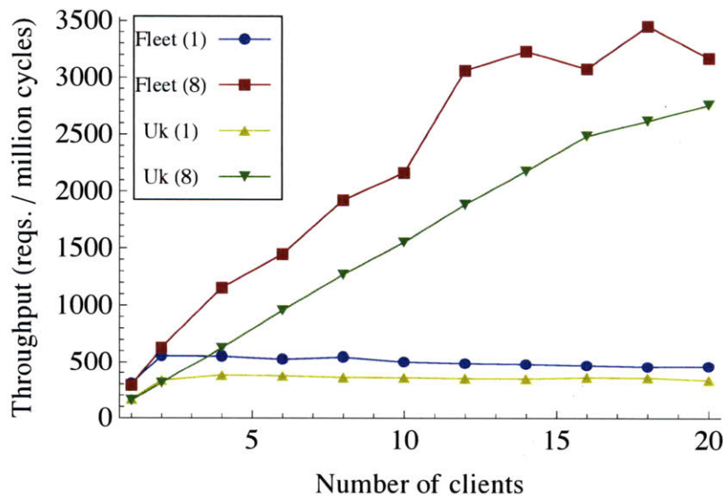
Figure 6-4: Messaging performance comparing the name service fleet design and the prior microkernel naming design. Results are shown for round-trips of small messages, with one and eight servers servicing requests. Legend indicates the design and number of servers ( e.g. , “Uk (8)” is microkernel with 8 servers). Results demonstrate significantly improved messaging performance in the name service fleet design.
