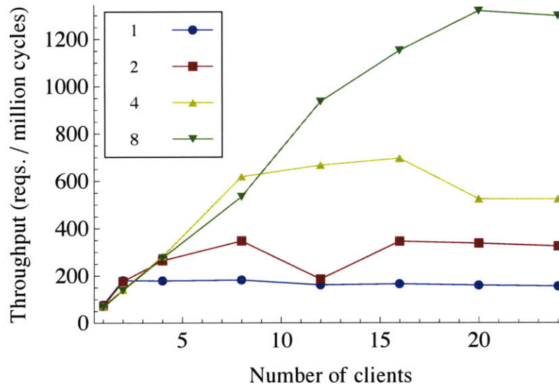
Figure 6-1: Lookup performance in the name service fleet. Legend indicates size of name service fleet. Performance scales well with number of clients until fleet saturates. Peak service rate scales well with fleet size.
