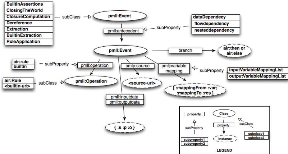
Figure 8: AIR Justification Ontology: All concepts defined without a prefix are in the airj namespace
