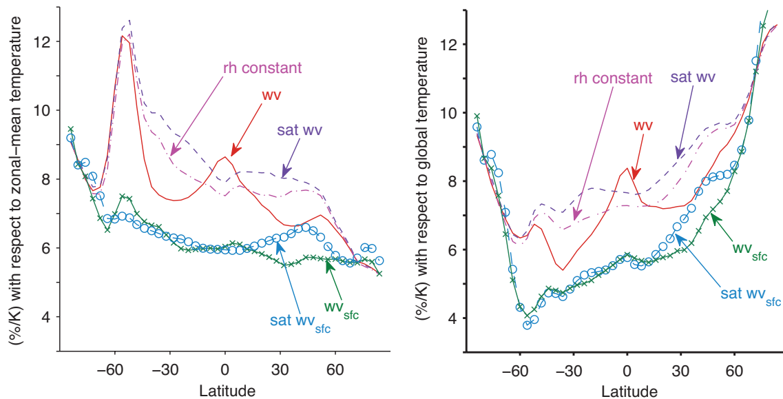
Figure 1. Rates of change ( \%/K ) of column water vapor (red solid), column water vapor with an invariant distribution of relative humidity (pink dashed-dotted), saturation column water vapor (purple dashed), surface specific humidity (green line and crosses), and surface saturation specific humidity (blue line and circles). Rates of change are with respect to zonal-mean surface air temperature (left panel) and global-mean surface air temperature (right panel). The values shown are multi-model means of estimates of the differential rates of change based on equation (2) and differences between 1980-1999 and 2080-2099.
