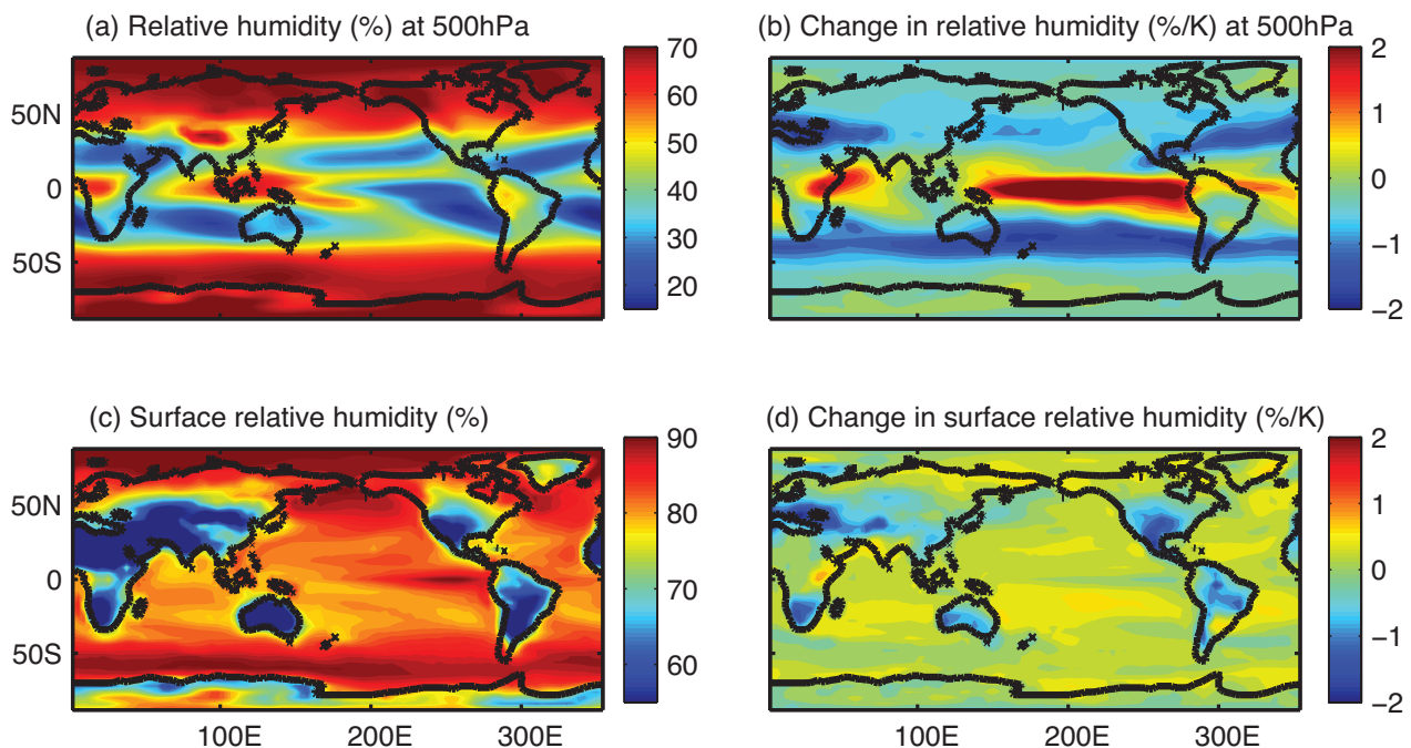
Figure 2. Mean relative humidity (%) for the period 1980-1999 and its rates of change (%/K) under climate change at 500hPa (a,b) and at the surface (c,d). The rates of change are based on absolute rather than fractional changes in relative humidity (same time periods as in figure 1), are calculated with respect to global-mean surface air temperature, and are not modified using equation (2). Multi-model means are shown in all cases.
