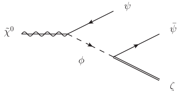
FIG. 6: If F_1 \gg F_2 and the SSM gaugino masses arise from sector 1 alone, then a bino-like LOSEP can decay into \zeta and two standard model fermions \psi\bar{\psi} through an off-shell scalar \phi , which is the superpartner of \psi . For m_{\tilde{\chi}^0}^2 \ll m_\phi^2 and \tilde{m}_1^2 \ll \tilde{m}_2^2 , the branching fraction into each \psi\bar{\psi} is entirely determined by the hypercharge of this field.
