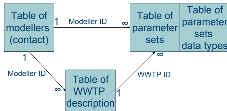
Figure 3-1. Database structure
