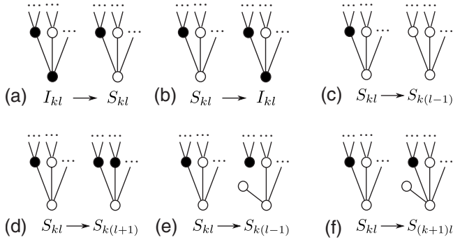
FIG. 1. Schematic illustration of the events described in the text which result in changing a node from one compartment to another. Susceptible nodes are represented by open symbols ( \circ ) and infectious nodes by filled symbols ( \bullet ).
