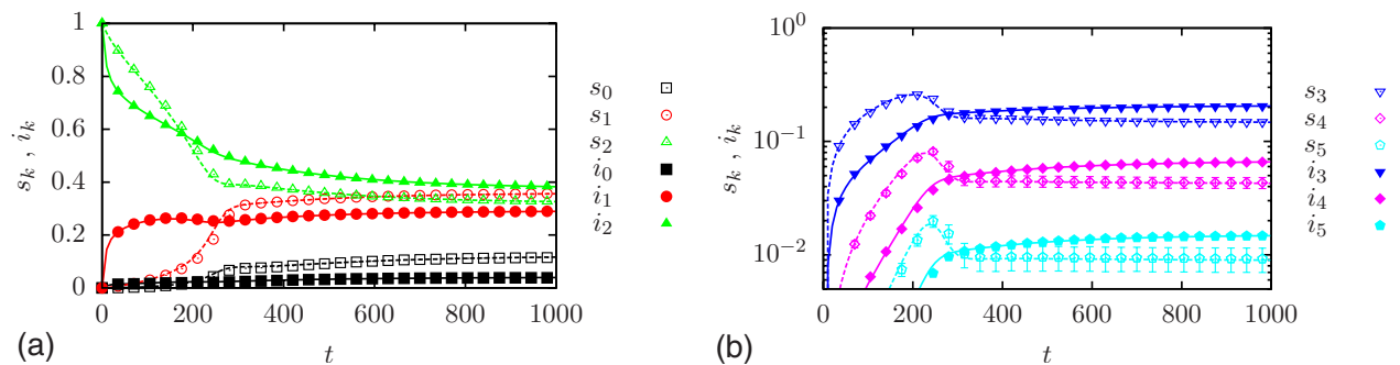
FIG. 3. (Color online) Degree probability s_k and i_k for susceptible (open symbols, dashed lines) and infectious (filled symbols, solid lines) individuals against time t on an adaptive network with a DR initial degree distribution ( k_0 = 2 ). The parameters of the system are \alpha = 0.005 , \beta = 0.06 , \gamma = 0.02 , and \epsilon = 0.1 , as in Fig. 2(a). Points and error bars (if larger than marker size) correspond to the mean and standard deviation computed over 10 000 Monte Carlo simulations; curves are the predictions of our analytical approach. (a) Low-degree nodes ( k = 0, 1 , and 2). (b) High-degree nodes ( k = 3, 4 , and 5).
