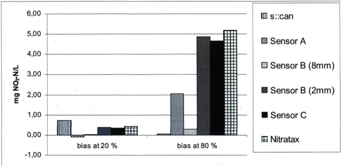
Figure 18: Comparison of bias
