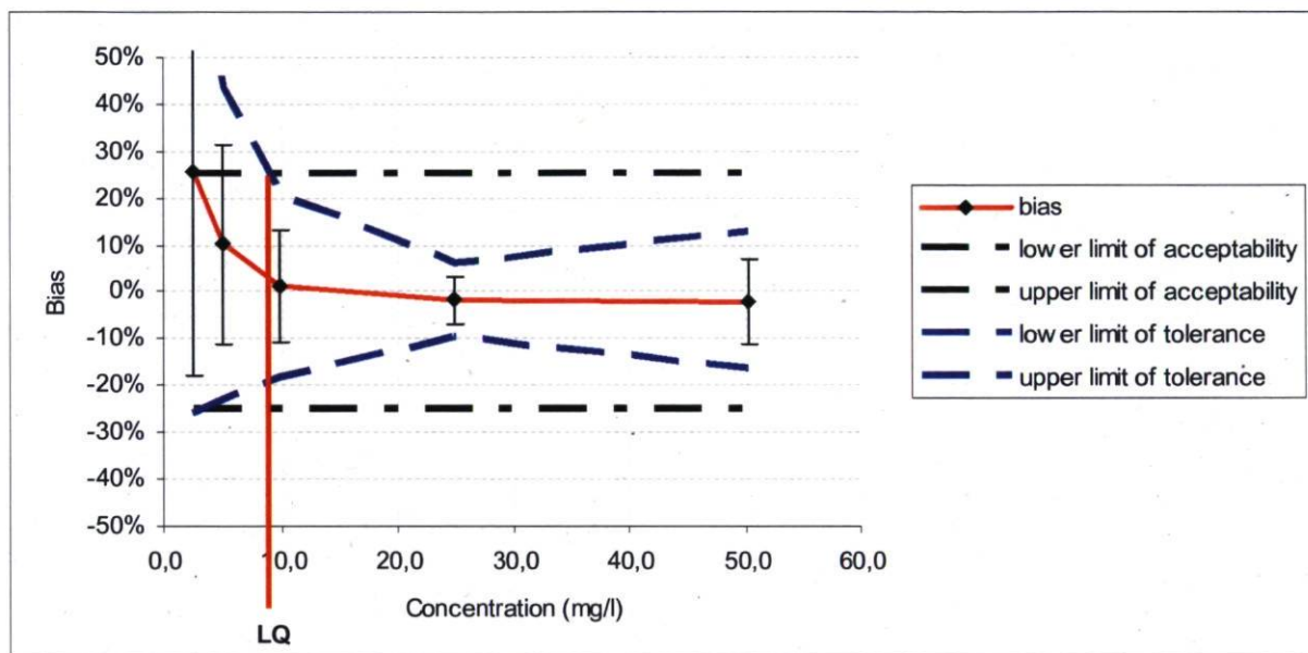
Figure 8: Accuracy profile (Hauduc, 2007)
