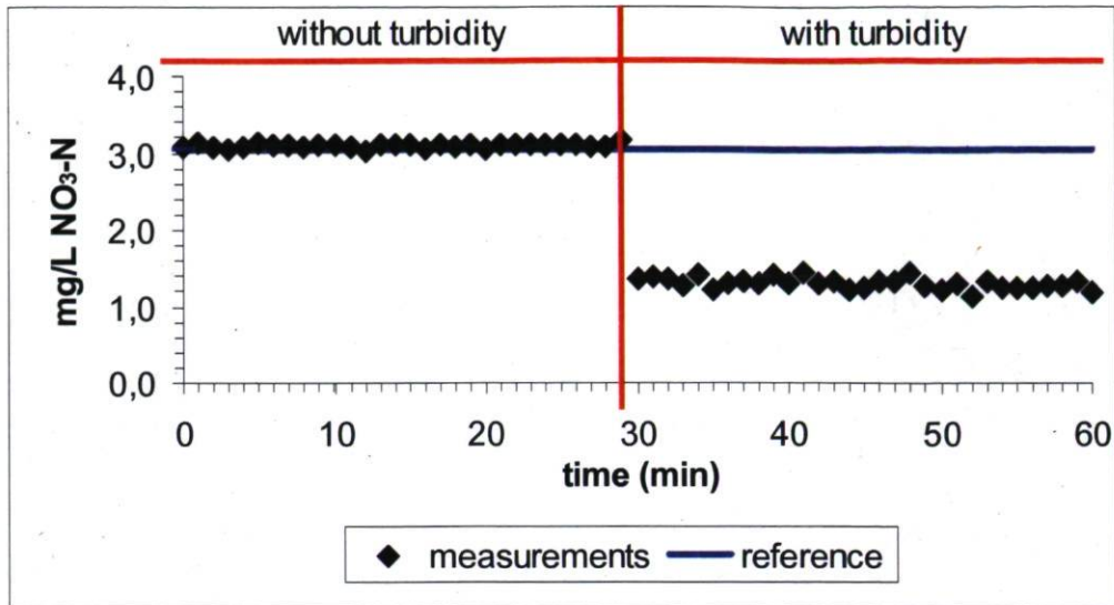
Figure 30: Effects of turbidity on nitrate measurements with the Spectro::lyser™ (3 mg/L NO 3 -N and 10 FNU)
