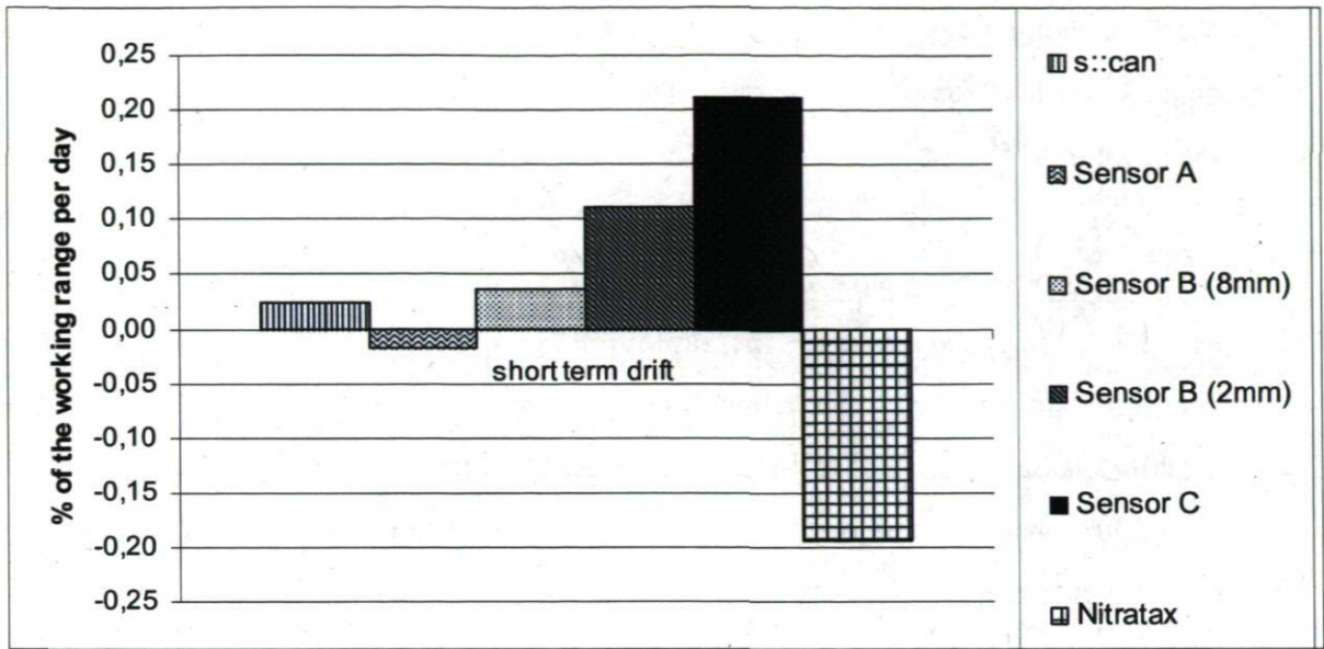
Figure 19: Comparison of short term drift
