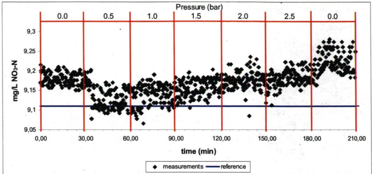
Figure 23: Nitrate concentration vs time for different air pressures applied to the Nitratax for a solution at approximately 10 mg \text{NO}_3\text{-N/L}
