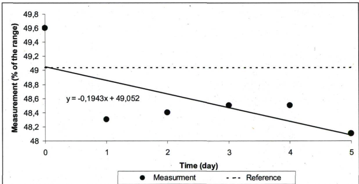
Figure 20: Measurement vs time for Nitratex
