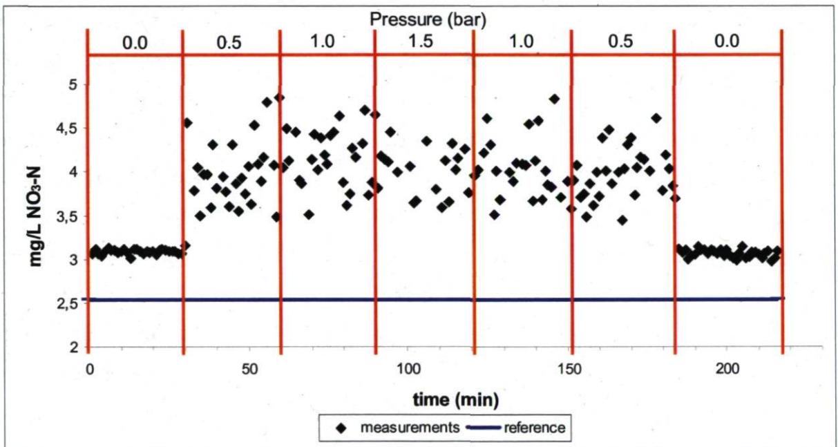
Figure 22: Nitrate concentration vs time for different air pressures applied to the Spectro::lyser tm for a solution at 3 mg NO 3 -N/L
