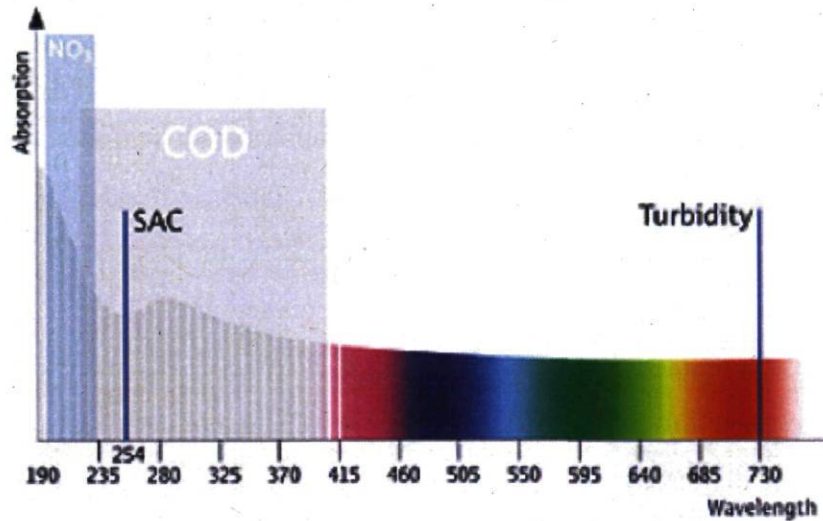
Figure 2: UV spectra and components absorption (Wedgewood Analytical, 2006)
