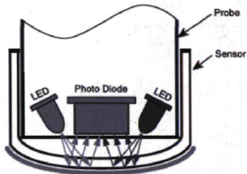
Figure 4: Luminescence dissolved oxygen probe 6 (source : Hach, 2005)
