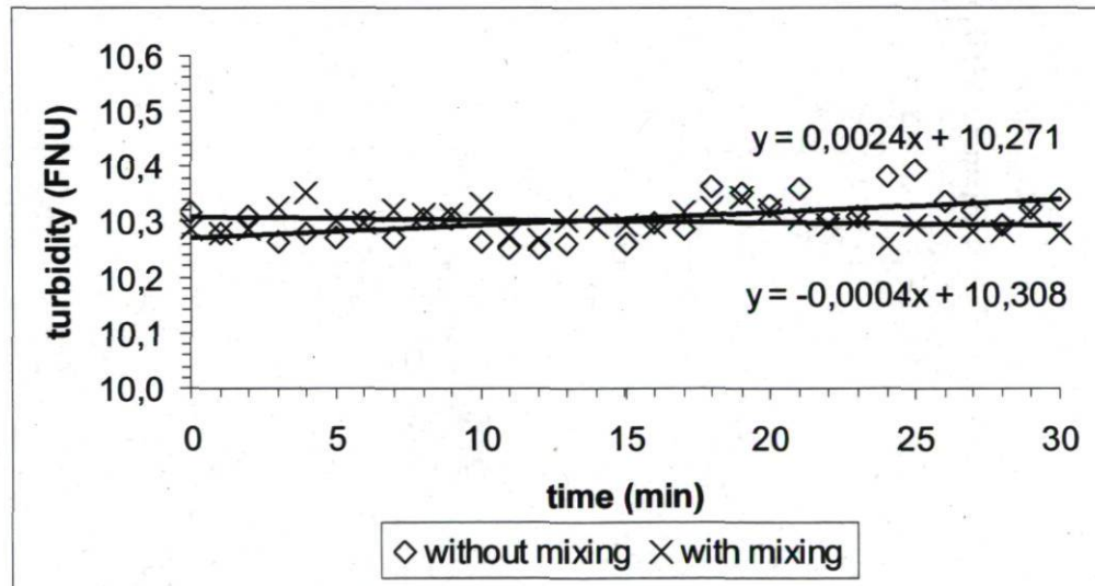
Figure 27: AMCO Clear® stability (with and without mixing) for a concentration of 50 FNU (non-diluted)
