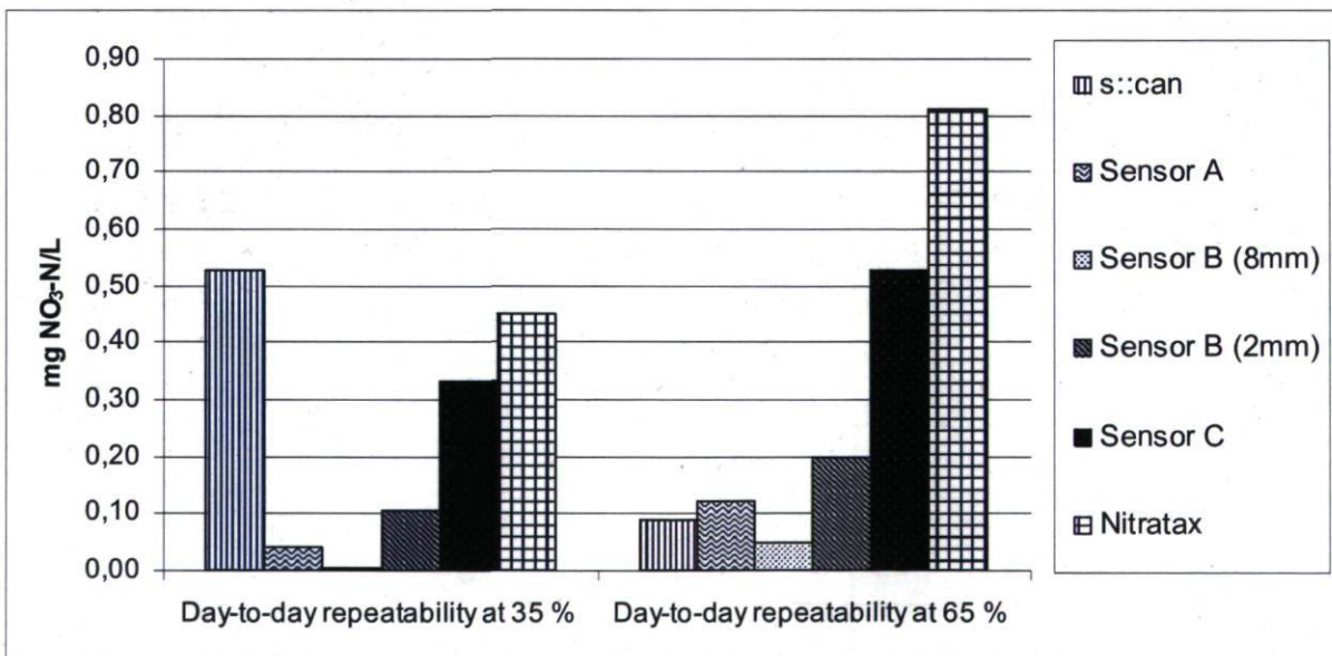
Figure 15: Comparison of day-to-day repeatability
