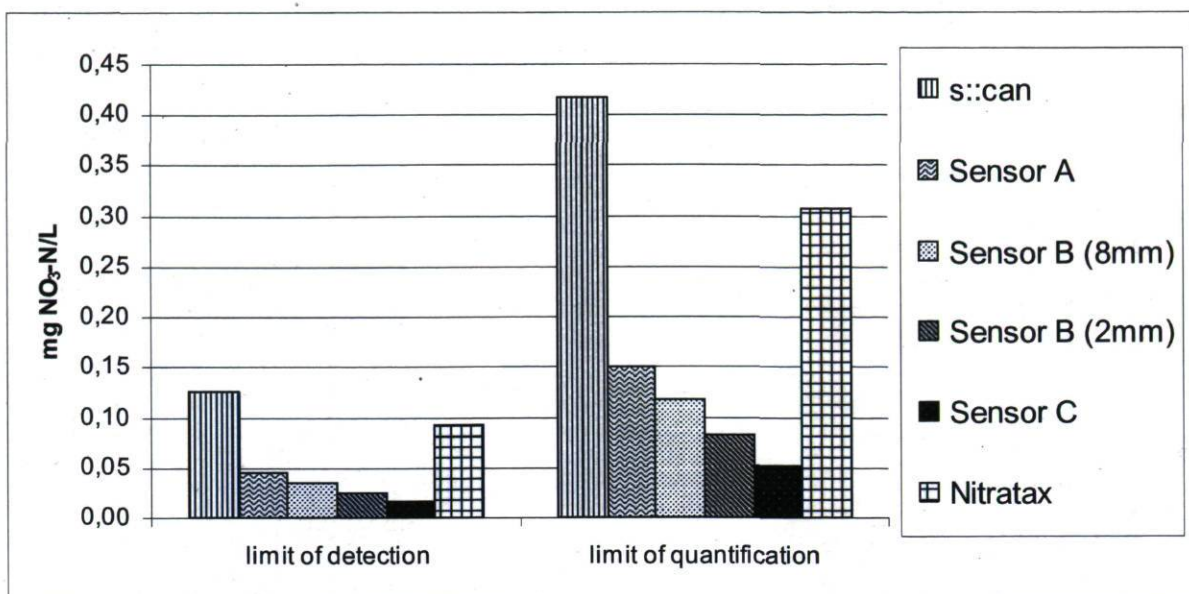
Figure 12: Comparison of limit of detection and quantification
