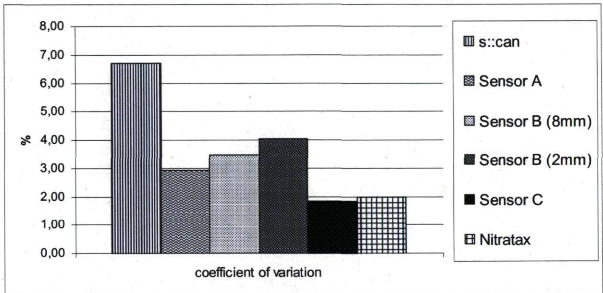
Figure 16: Comparison of coefficient of variation
