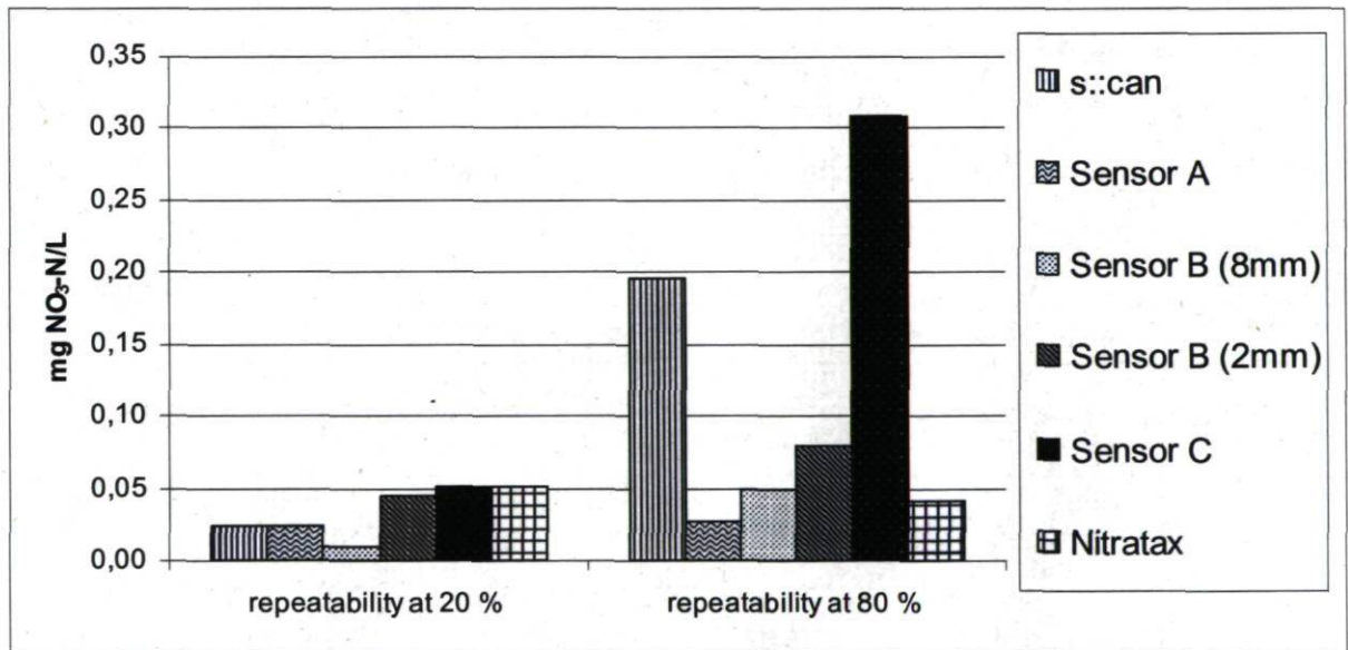
Figure 13: Comparison of repeatability
