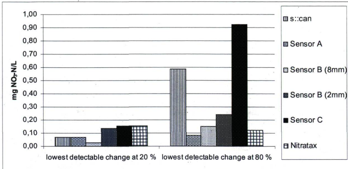
Figure 14: Comparison of lowest detectable change
