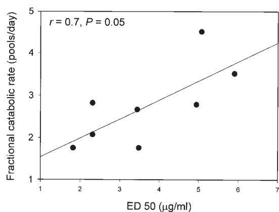
Fig. 5. Relationship between ED_{50} values for 3G10 and apoA-I fractional catabolic rate (FCR). ED_{50} represents the reconstituted complex concentration required to inhibit 50% of the maximal 3G10 binding on a HDL_3 -coated plate in a radioimmunoassay. 3G10 is a monoclonal antibody directed against residues 98–121 of the human apolipoprotein A-I molecule (23). A decrease in the ED_{50} value indicates an increase in the exposure of the 98–121 domain at the surface of the reconstituted Lp2A-I complex. FCR were calculated from the area under plasma decay curves of reconstituted complexes (see Table 1) using the equation of Matthew (31) and are expressed as pools/day \pm 0.3 (SD), and plotted against ED_{50} values expressed in \mu\text{g/ml} \pm 0.4 (SD). Correlation coefficients were determined by the method of Spearman.
