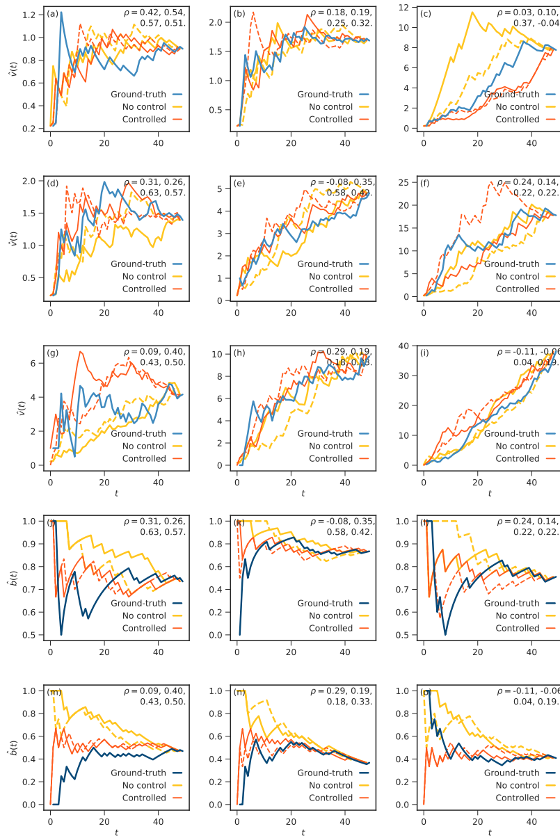
FIGURE 4.13 – Evolution of the ground-truth (blue lines), of two uncontrolled samples (yellow lines), and of two controlled samples (orange lines), on artificial graphs of T = 50 edges generated by the model. We use the kernel exponent (left column) \gamma = -1 , (central column) \gamma = 0 , and (right column) \gamma = 1 , and the node creation probability equals (top row) b = 1 , (second and fourth row) b = 0.75 , and (third and last row) b = 0.50 . The first 9 panels show the evolution of the estimated variance \hat{v}(t) and the last 6 panels show the evolution of the estimated node creation probability \hat{b}(t) . The panels are matched, e.g., the dotted orange line in panels (d) and (j) illustrate the evolution of the estimators in a single sample, on the same graph. There are only six panels associated with \hat{b}(t) since its evolution is trivial on trees (i.e., when b = 1 ). The number in the top-right corner of each panel indicates the correlation of the ground-truth and the uncontrolled samples (two topmost numbers), and of the ground-truth and the controlled samples (the two numbers below).
