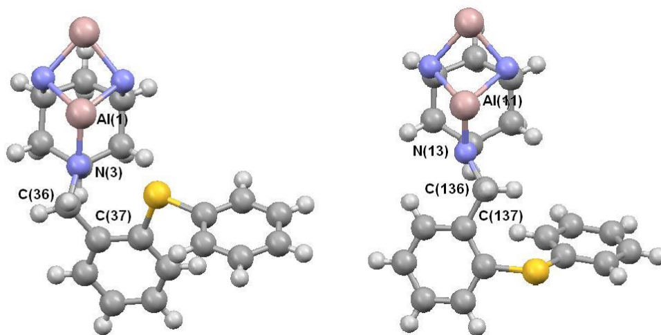
Figure 3. Depiction of the different orientations of the functionalized arm in crystal of 6
