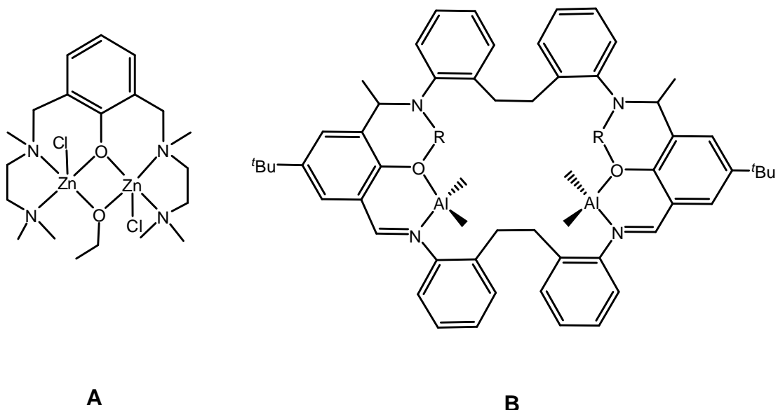
Figure 1. Two examples of bimetallic catalysts for ring-opening polymerization of cyclic esters.
