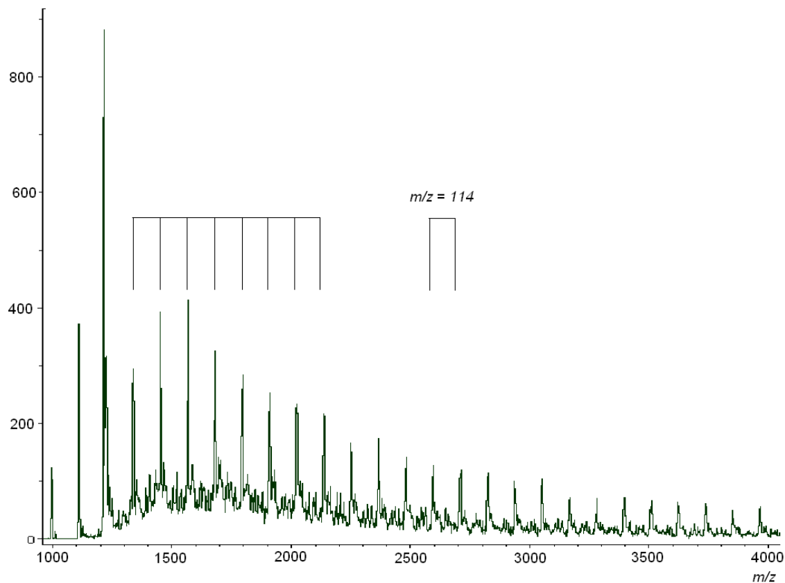
Figure 6. MALDI-TOF spectrum of entry 3.
