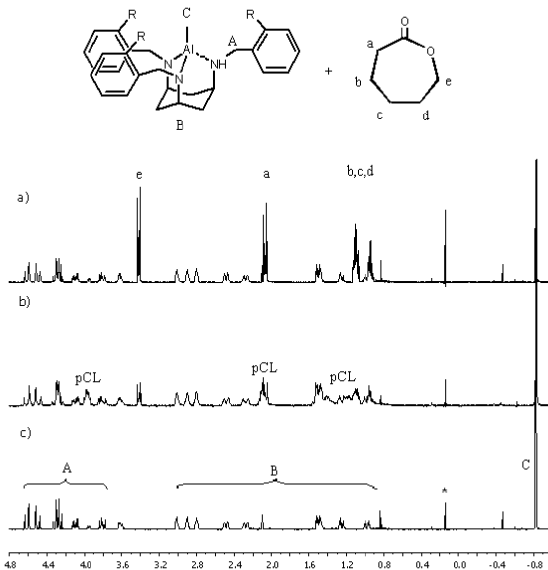
Figure 9. 1 H NMR spectra of catalyst 8 in the presence of 1 equiv. of CL in benzene- d 6 after a) 5 minutes at room temperature, b) 18 hours at 60°C, and c) before the addition of CL.
