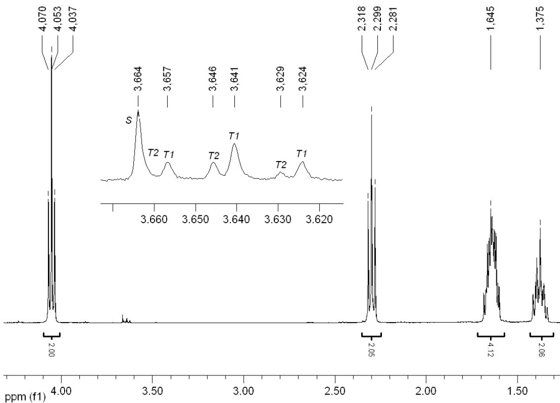
Figure 5. Typical ^1\text{H} NMR spectrum of polycaprolactone (entry 9) with a blow up of the resonances of the terminal groups. T1 and T2 are for the two triplets and S for the singlet.
