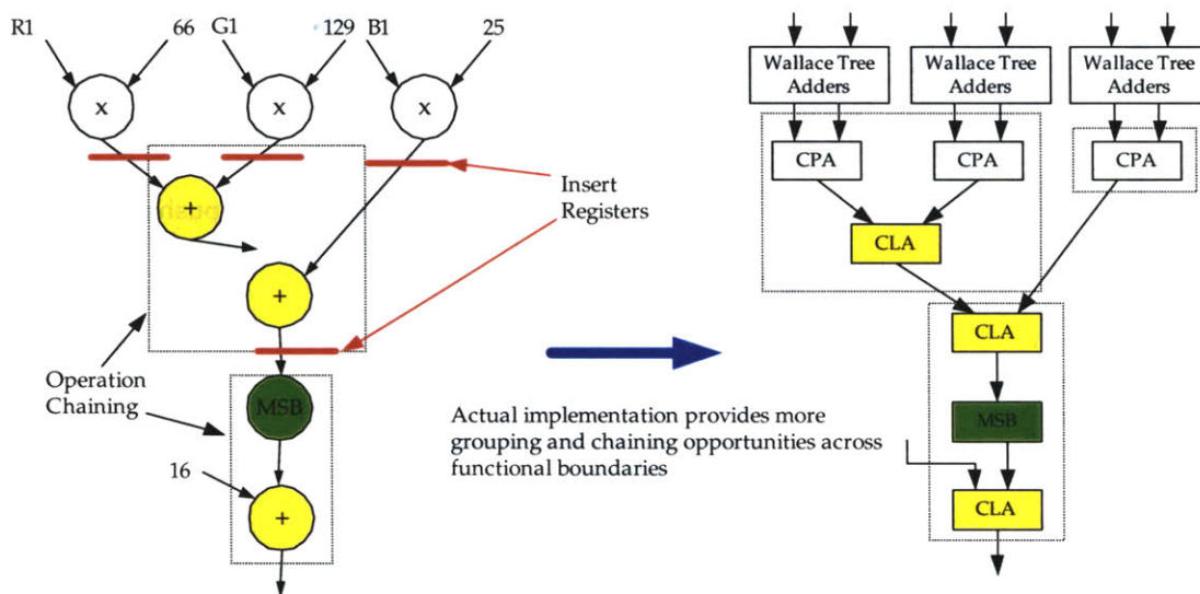
Figure 4-6: Code segments in Figure 4-4 translated into hardware macro functions.
