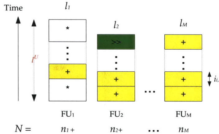
Figure 8-2: Finding upper bound visualized as minimizing the highest bucket.
