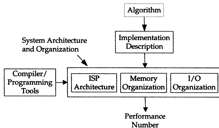
Figure 3-1: Performance is determined by the codes, the compiler, the architecture of the system and its components, and the organization of the components.
