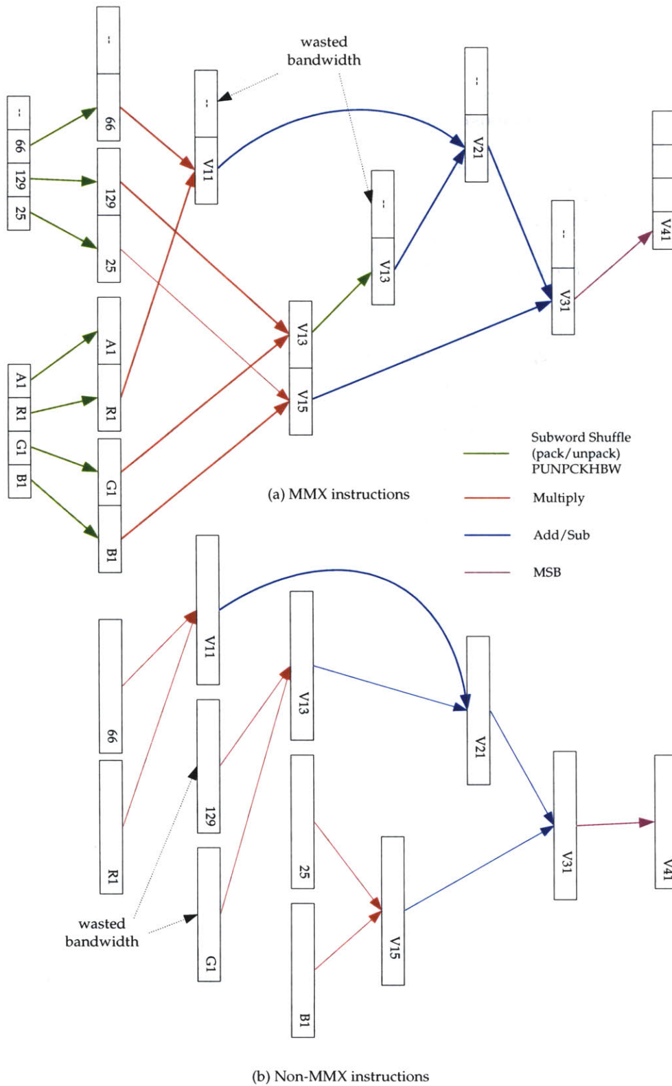
Figure 4-5: Code segment of color space transform represented as a sequence of three-register instructions on (a) MMX architecture (b) non-MMX architecture.
