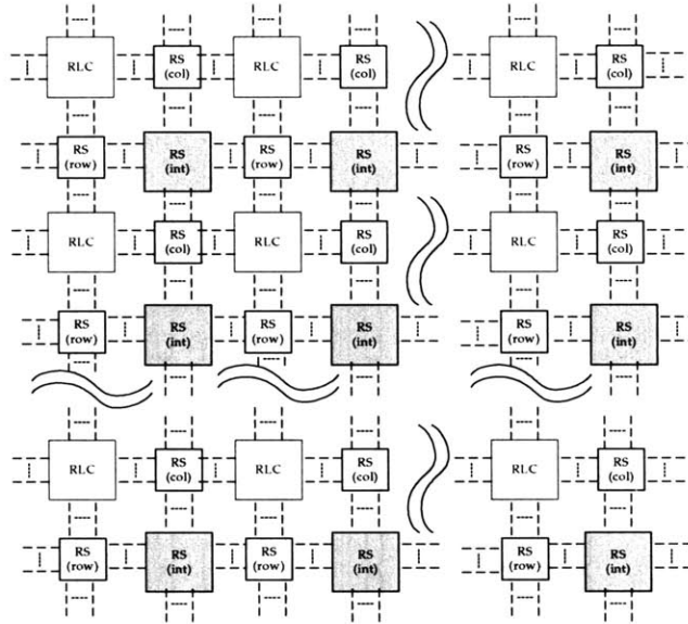
Figure 5-1: Topology and organization of a symmetrical FPGA
