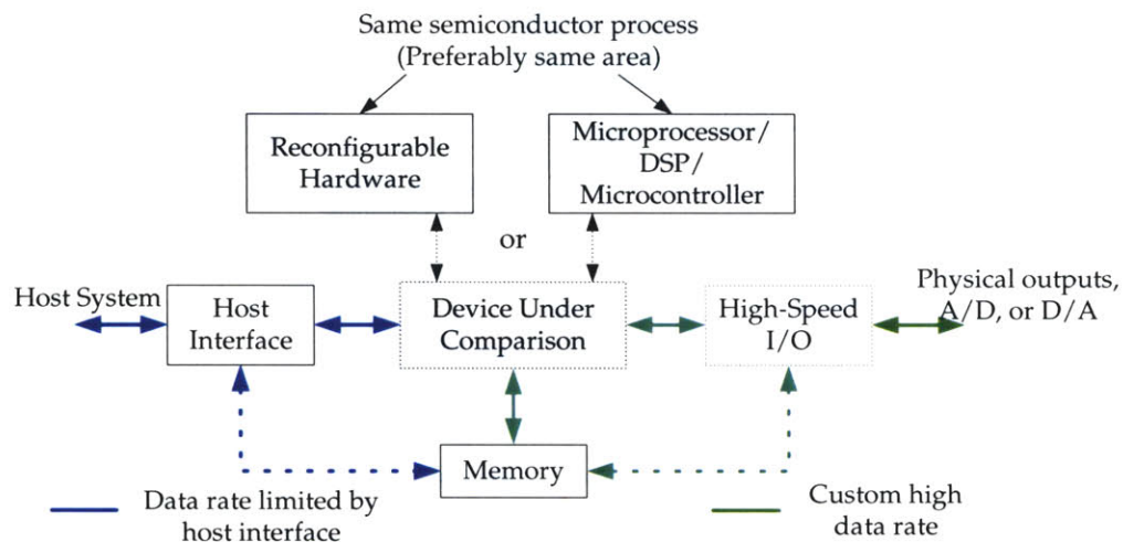
Figure 9-3: Drop-in replacement for performance comparison.
