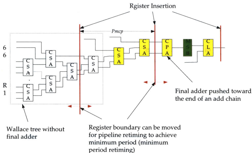
Figure 4-7: Pipeline retiming (or minimum period retiming) technique can be used to achieve high clock speed.
