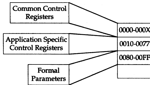
Figure 7-6: Memory address for common registers is fixed, while application specific registers addresses can change with applications 25 .
