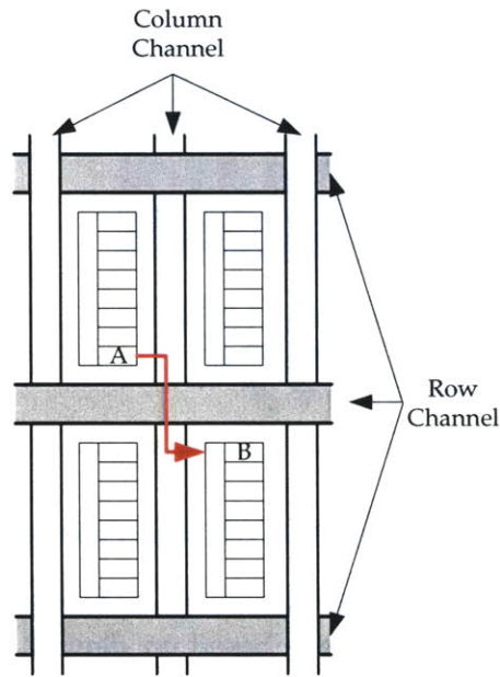
Figure 5-9: Estimate of minimum routing delay in Altera's FastTrack routing architecture.
