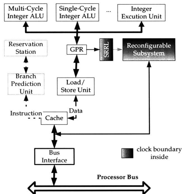
Figure 7-9: An integrated general-purpose reconfigurable architecture. The microprocessor core and reconfigurable logic core run asynchronously.
