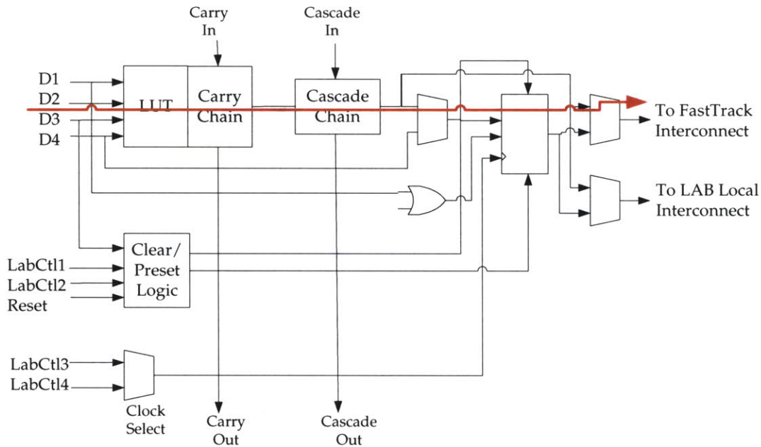
Figure 5-7: Altera FLEX 10K family FPGA combinational path delay.
