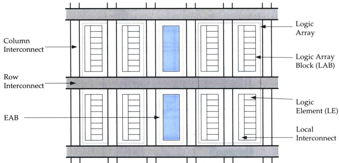
Figure 5-3: Altera Flex 10K architecture.
