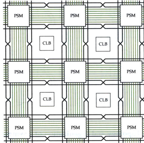
Figure 5-2: Xilinx's XC4000 single- and double length lines, with programmable switch matrices (PSMs) 12 .
