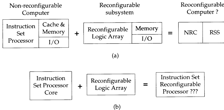
Figure 3-7: Searching for new architectures (a) an ad-hoc organization based on existing organization (b) an integrated organization
