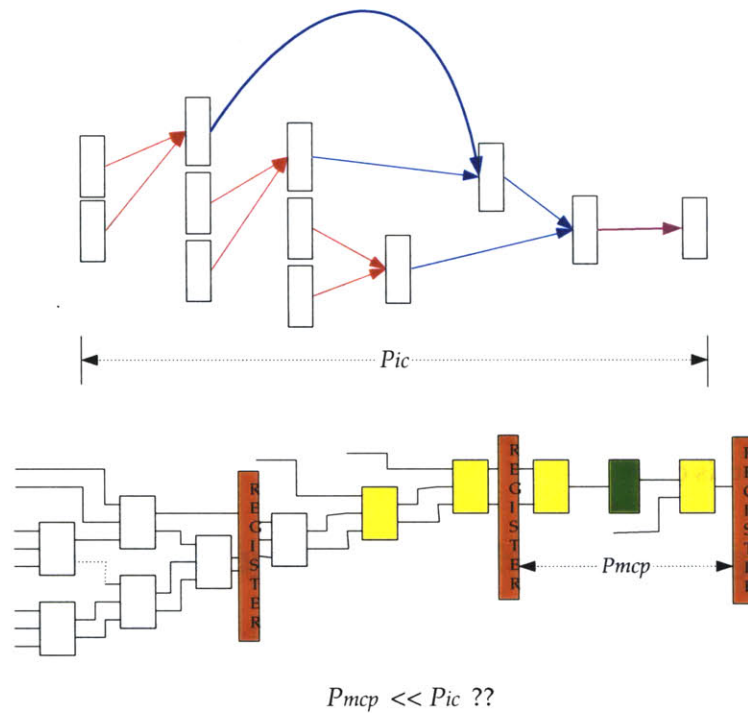
Figure 4-8: Instructions executed in sequence in the temporal domain vs. concurrent hardware execution in spatial domain.
