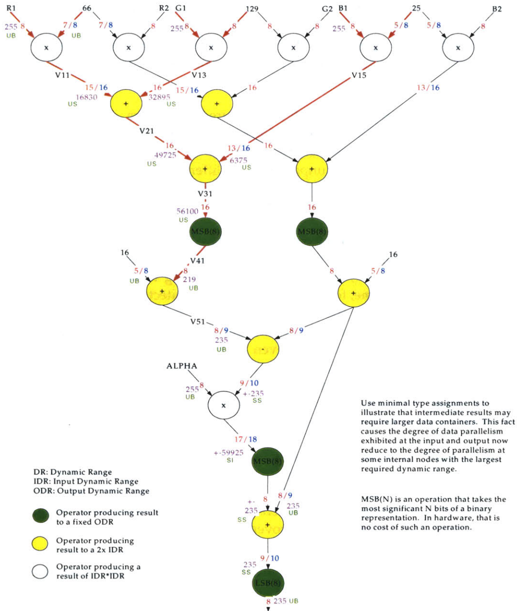
Figure 4-4: A color transformation and alpha blending example (shown only the luminance).
