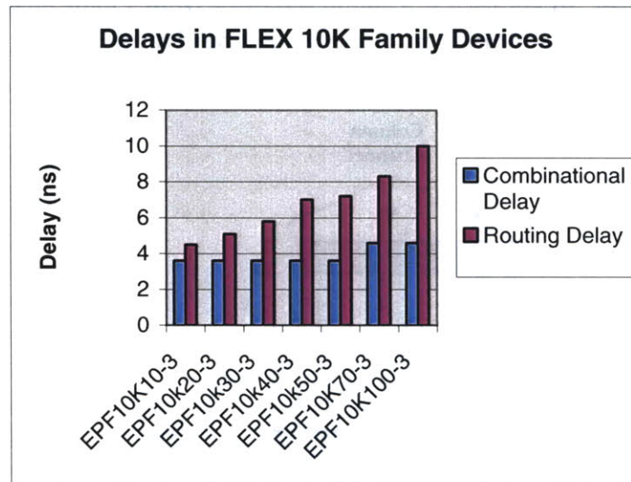
Figure 5-10: Delays in Altera FLEX 10k family devices (speed rating -3)
