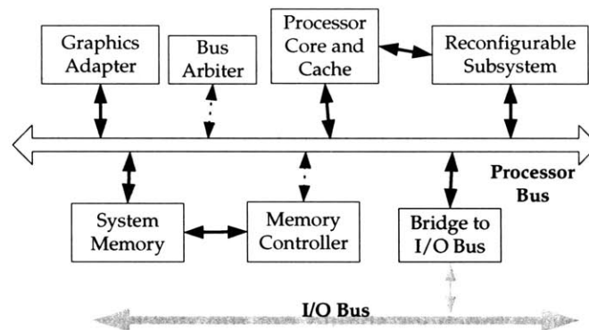
Figure 7-2: A reconfigurable subsystem directly sitting on the processor bus.
