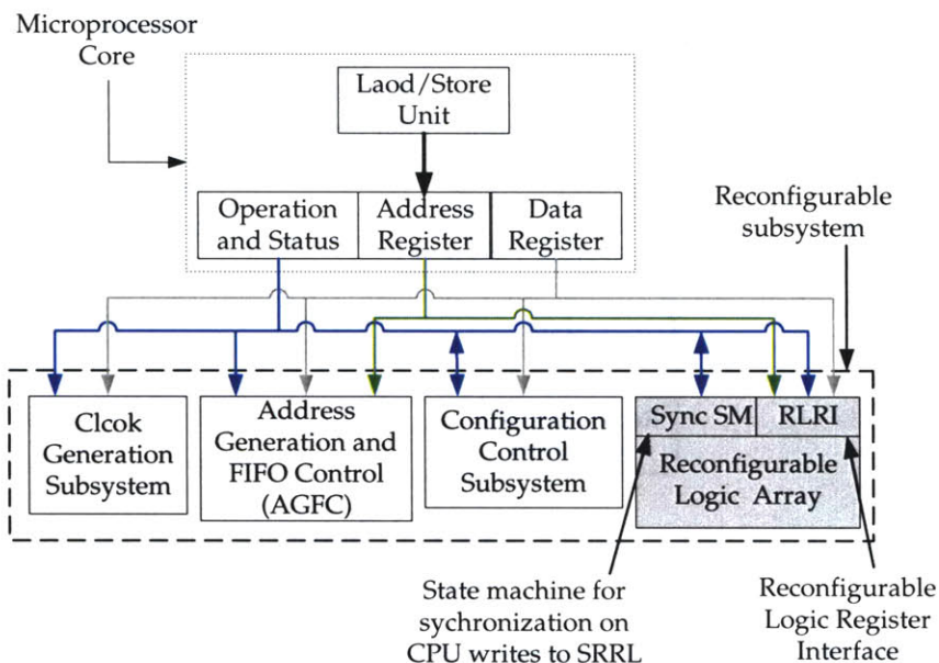
Figure 7-8: Reconfigurable system model showing the special register interface.
