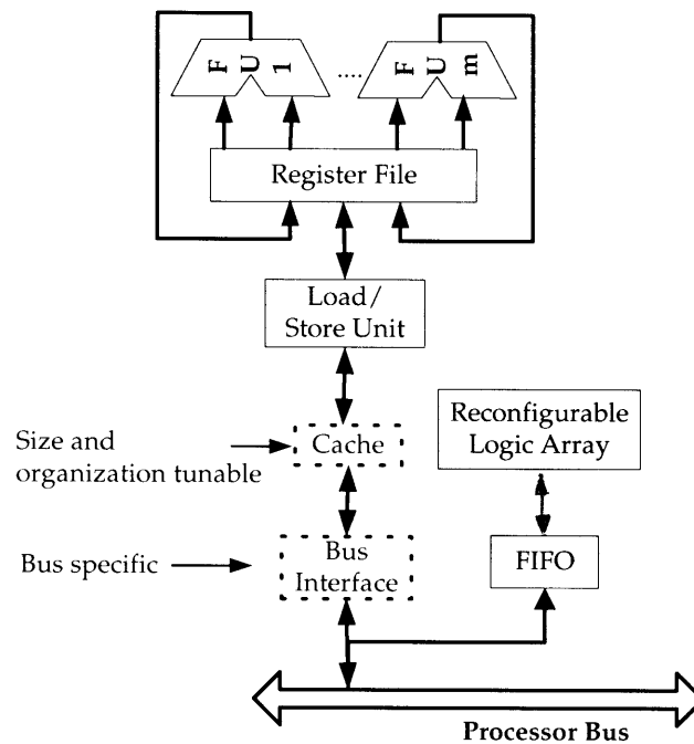
Figure 7-10: A datapath model of a general-purpose reconfigurable core.
