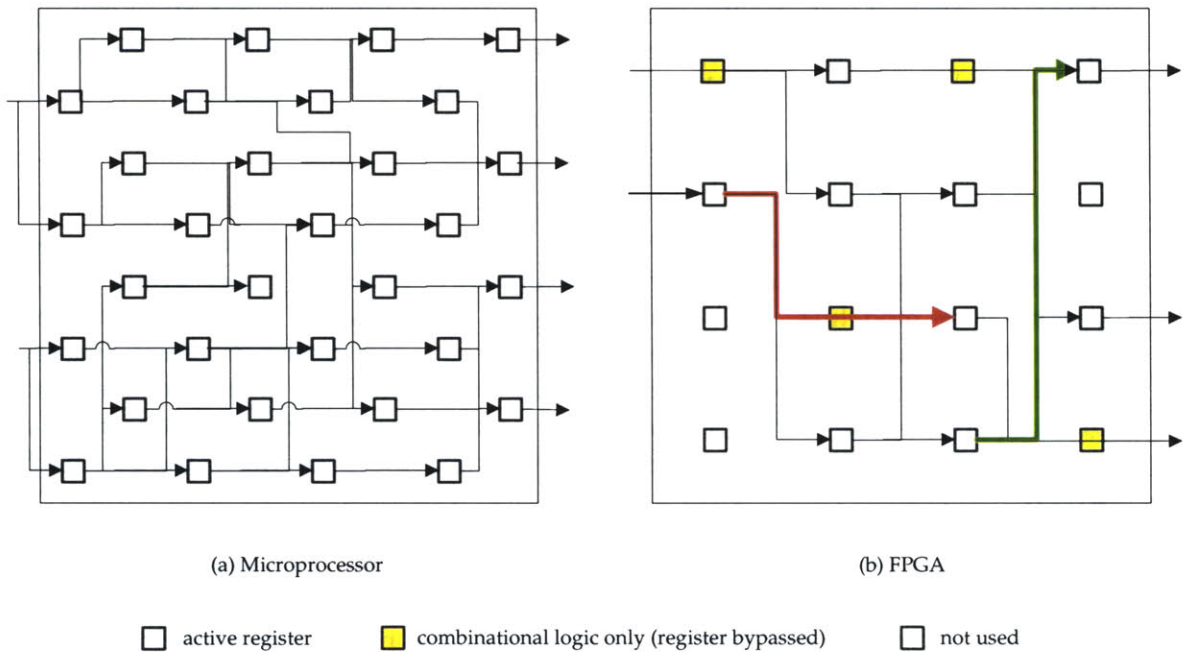
Figure 5-14: Register packing density (a) every register in a microprocessor is active (b) not every logic cell is used for every configuration, some are used for its combinational part only.
