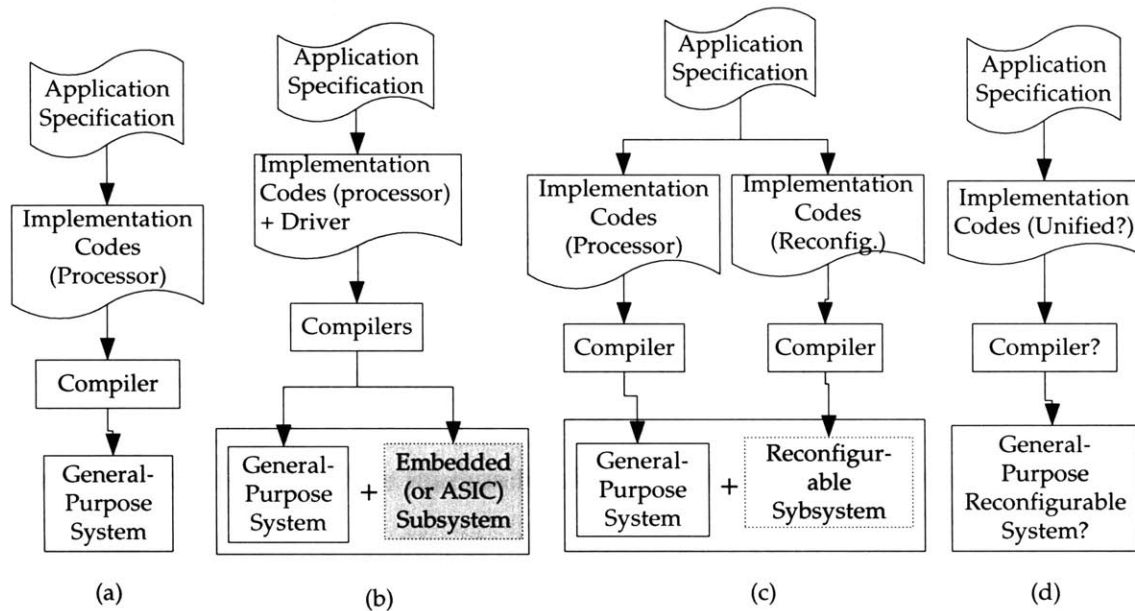
Figure 3-4: Four codes-architecture-organization-compiler structures: (a) general-purpose computer host (b) with add-on application-specific subsystem (c) with add-on reconfigurable subsystem (d) future reconfigurable system.
