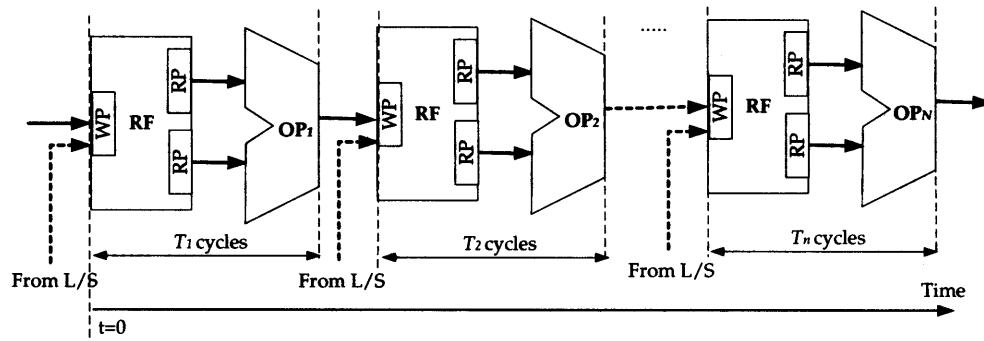
Figure 6-5: Temporal expansion of N data processing instructions.
