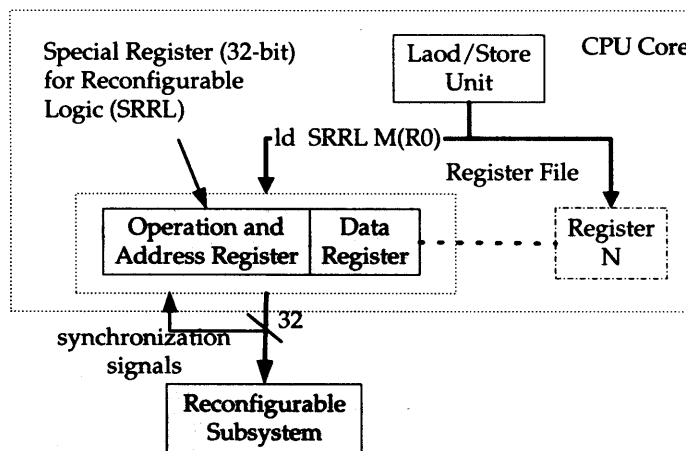
Figure 7-7: A special register for reconfigurable logic (SRRL) in an microprocessor's register file.
