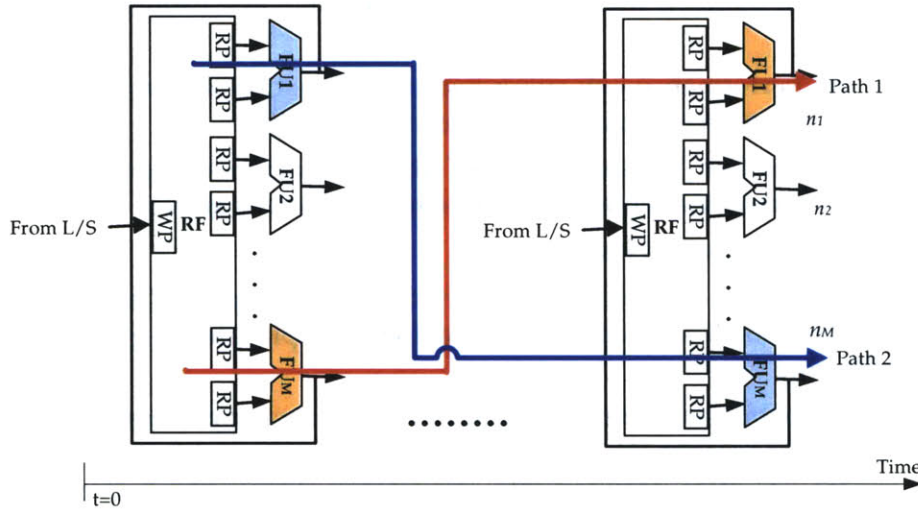
Figure 6-7: Temporal expansion of multiple FUDP. N instructions may be distributed among M functional units.
