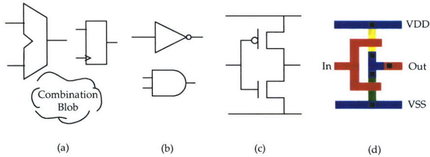
Figure 5-13: VLSI design hierarchy (a) register transfer level (b) gate level (c) circuit level (d) physical layout
