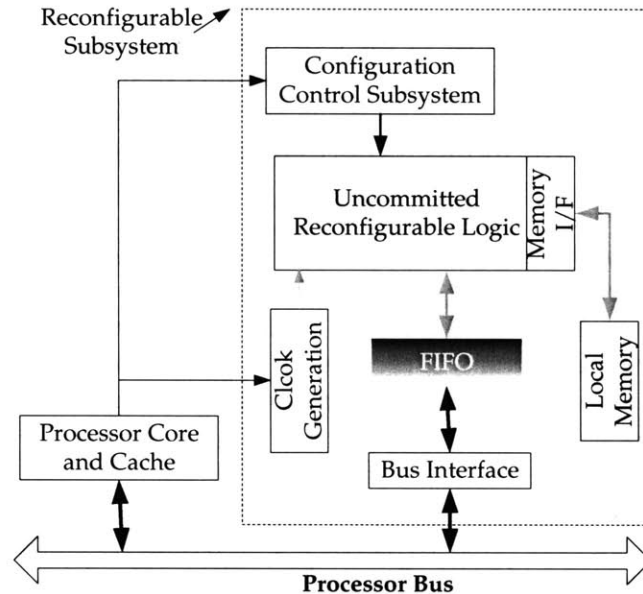
Figure 7-5: Reconfigurable subsystem showing constituent fixed functions and a reconfigurable logic core
