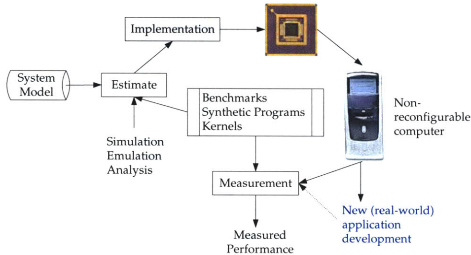
Figure 3-5: Non-reconfigurable computer system design and application development paradigm.
