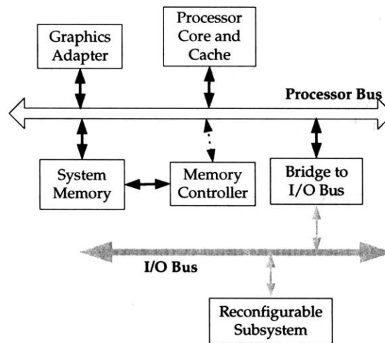
Figure 7-1: A reconfigurable subsystem attached to the I/O bus of a general-purpose system.
