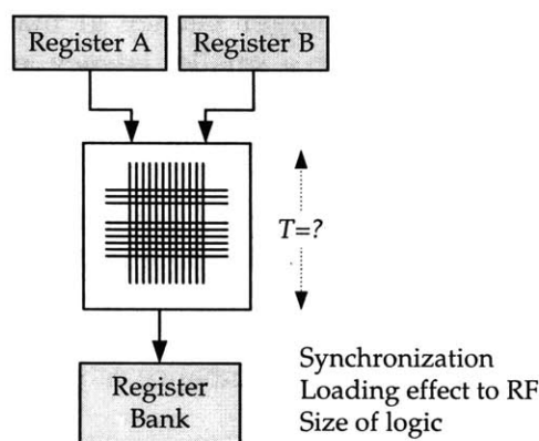
Figure 7-12: Problems with PFU as a functional unit attached to a register file
