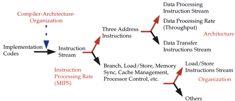
Figure 6-1: An instruction can be separated into data processing stream and control and data moving stream.
