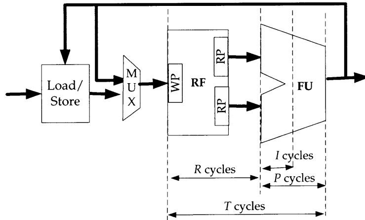
Figure 6-3: A single pipelined functional unit connected to a register file.
