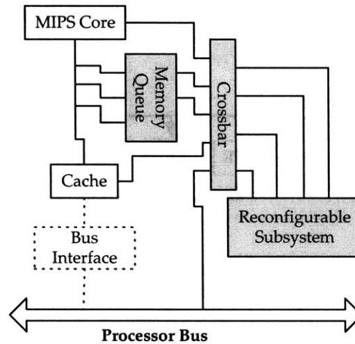
Figure 7-13: Garp architecture [11].
