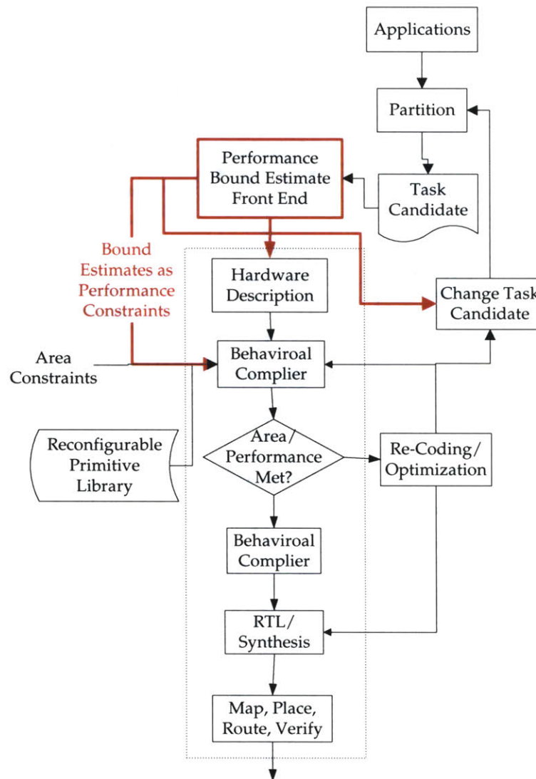
Figure 8-7: Performance bound estimates as a front end tool integrated into hardware design flow.
