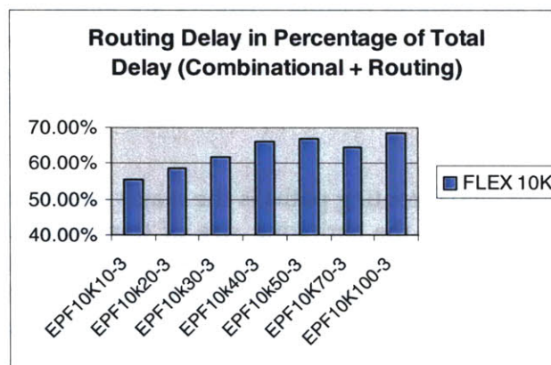
Figure 5-11: Percentage of Routing Delay in Minimum Clock Period increase with the Size of the FPGA.
