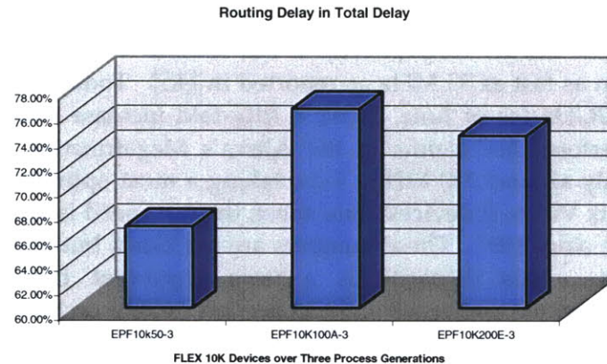
Figure 5-12: Routing Delay in FPGA Grow with Process Technology Upgrades 20 .
