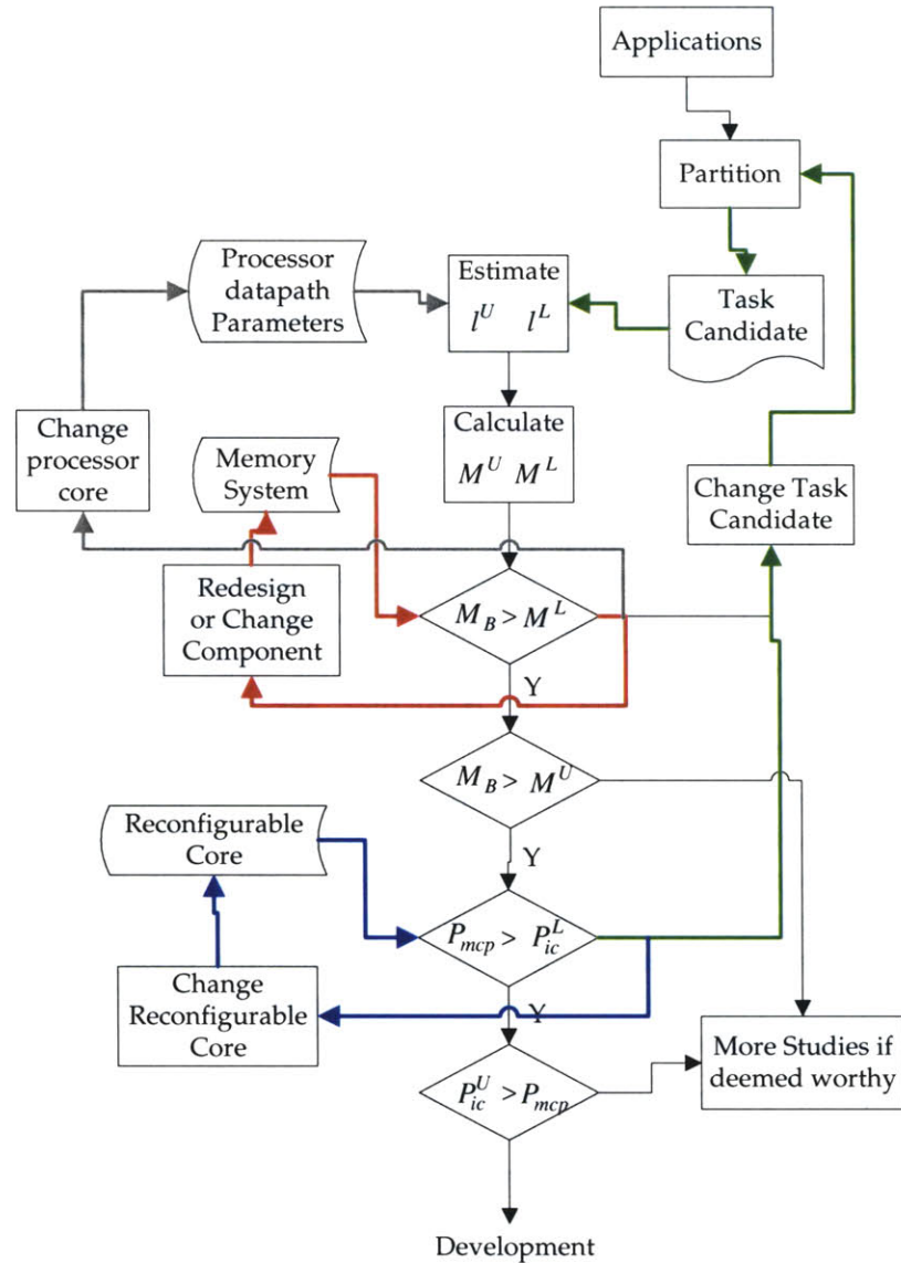
Figure 8-5: Front end for new reconfigurable system design
