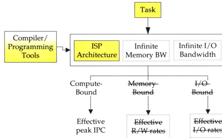
Figure 3-3: Determining performance bottleneck by emulating computer, memory, or I/O workloads.
