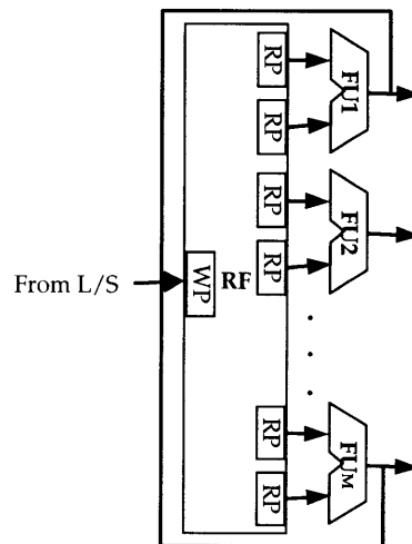
Figure 6-4: Multiple functional units sharing the same register file.
