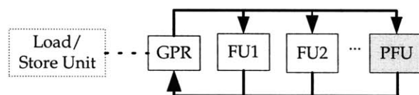
Figure 7-11: The PRISC architecture. A programmable functional units is sitting on the register bus.
