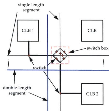
Figure 5-8: Estimation of a lower bound on routing delay (e.g. switch based routing structure).
