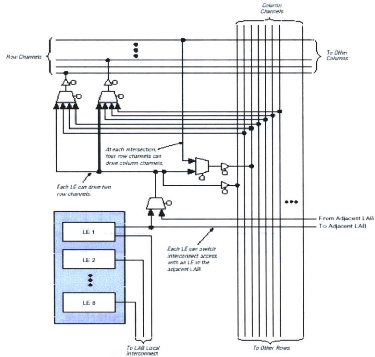
Figure 5-4: Altera FLEX 10K family's LAB connections to row and column interconnect.
