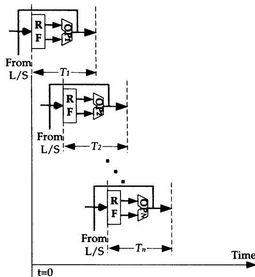
Figure 6-6: A block of N instructions execute on a pipeline functional unit.
