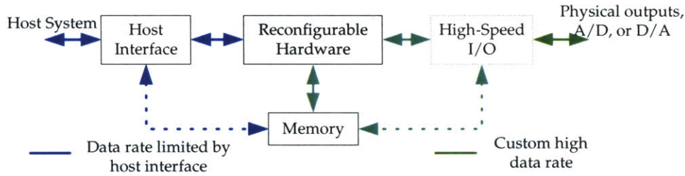
Figure 9-1: A typical functional datapath block diagram of a reconfigurable subsystem on early custom computing machines.
