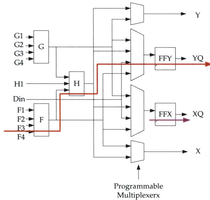
Figure 5-6: Estimation of combinational delay. Example uses Xilinx XC4000 family FPGAs.
