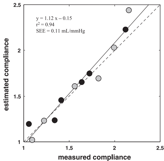
Fig. 9. Relationship between compliance (in \text{ml}/\text{mmHg} ) measured using the standard clinical formula (Eq. 8) and that estimated from the minimization method. Dotted line, identity line. Solid and shaded circles correspond to data before and after surgery, respectively.
