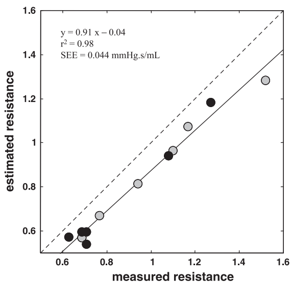
Fig. 8. Relationship between resistance (in \text{mmHg}\cdot\text{s}\cdot\text{ml}^{-1} ) measured using the standard clinical formula (Eq. 7) and that estimated from the minimization method. Dotted line, identity line. Solid and shaded circles correspond to data before and after surgery, respectively.
