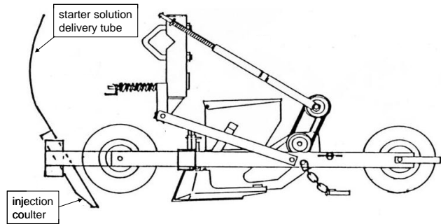
Fig. 2. Stanhay seed drill showing position of commercial prototype injection coultter.
