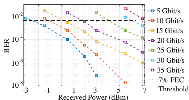
Fig. 6. BER as a function of the received power for different bitrates. Results are measured at V_{\text{bias}} of -1.5 V and operational wavelength of 1570 nm.
