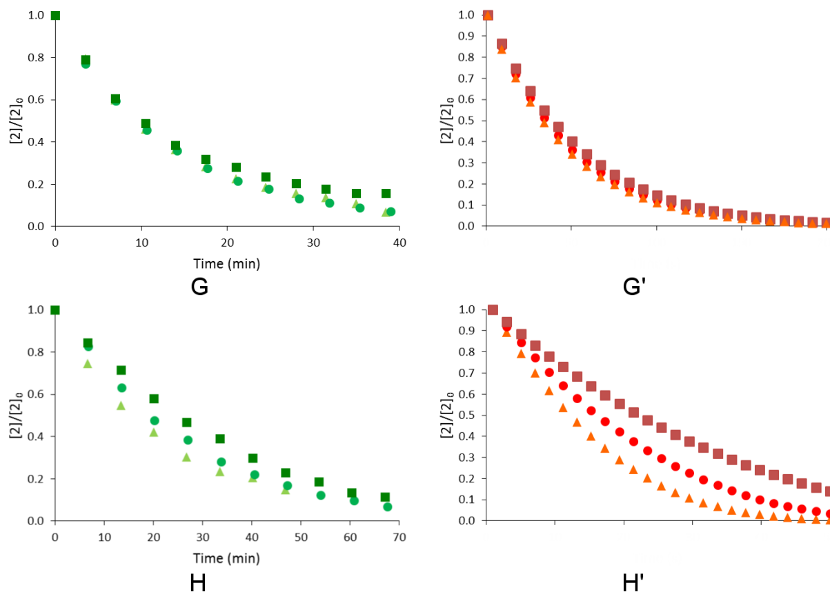
Figure 9. Left: Consumption of a solution of aminoborane 2 at various concentrations (38.8 ▲, 77.5 ● and 155 ■ \mu\text{M} ) in chloroform- d with a 1550 \mu\text{M} concentration of 1-methylpyrrole at 40°C (top row) or thiophene at 60°C (bottom row). Right: Simulated rate of consumption according to DFT data.
