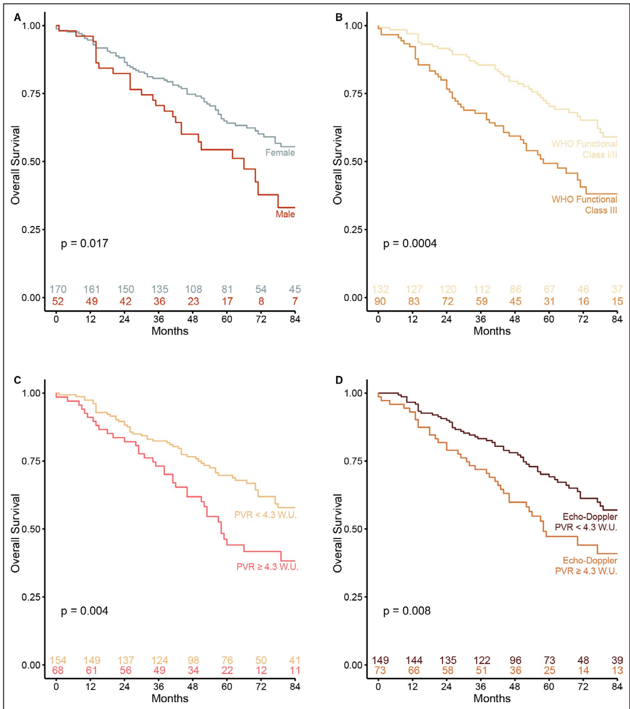
Figure 6. Kaplan-Meier overall-survival curves based on most relevant predictors.
