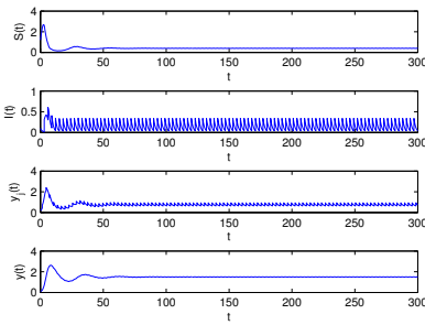
(a) Time series of system (1.3). System (1.3) is uniformly permanent.
