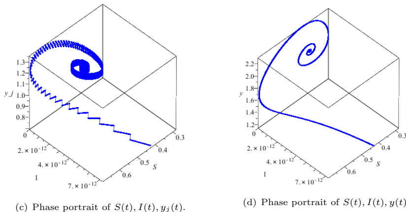
(c) Phase portrait of S(t), I(t), y_j(t) .
