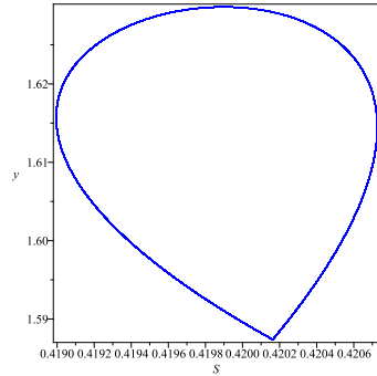
(b) Phase portrait of S(t), y(t) .
