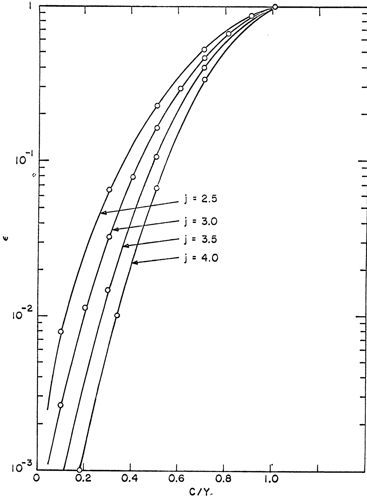
FIGURE 16. AREA RATIO VERSUS COMPLIANCE RATIO
