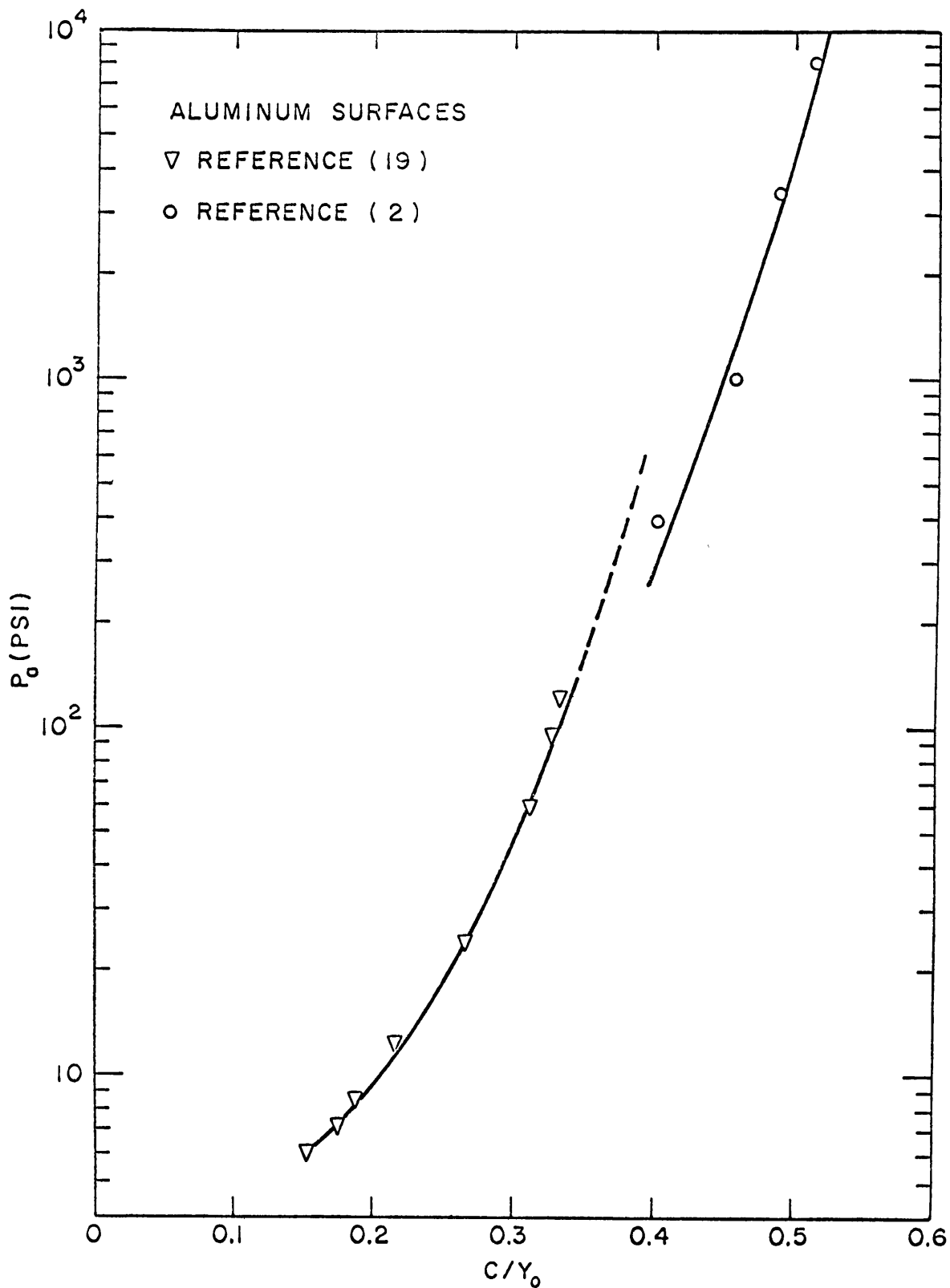
FIGURE 30. APPARENT PRESSURE VERSUS COMPLIANCE RATIO
