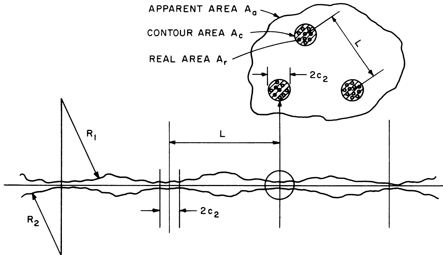
FIGURE 4. SPHERICAL CONTACT MODEL
