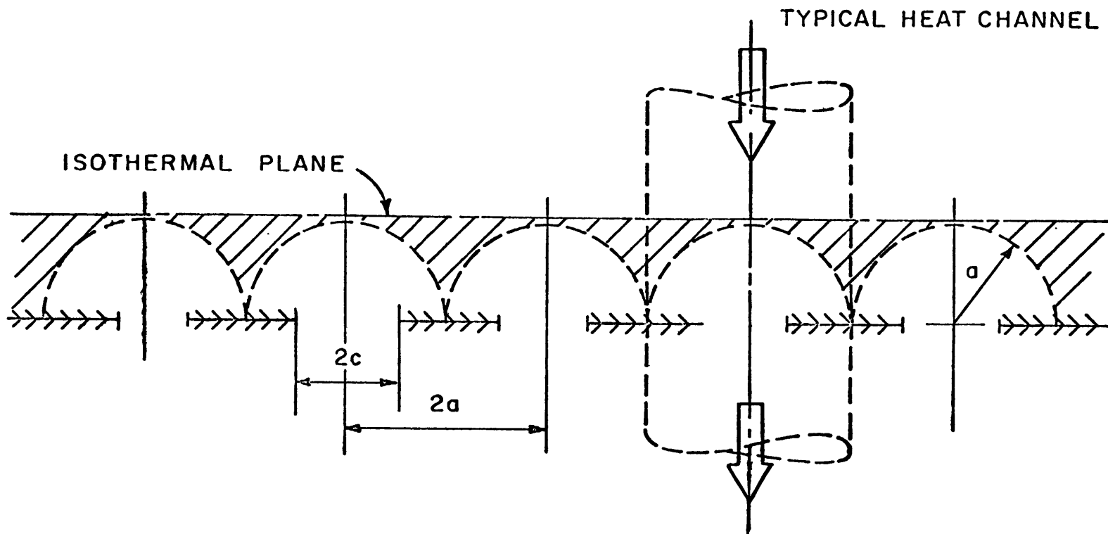
FIGURE 6. CONTACT MODEL FOR MULTIPLE CONTACTS
