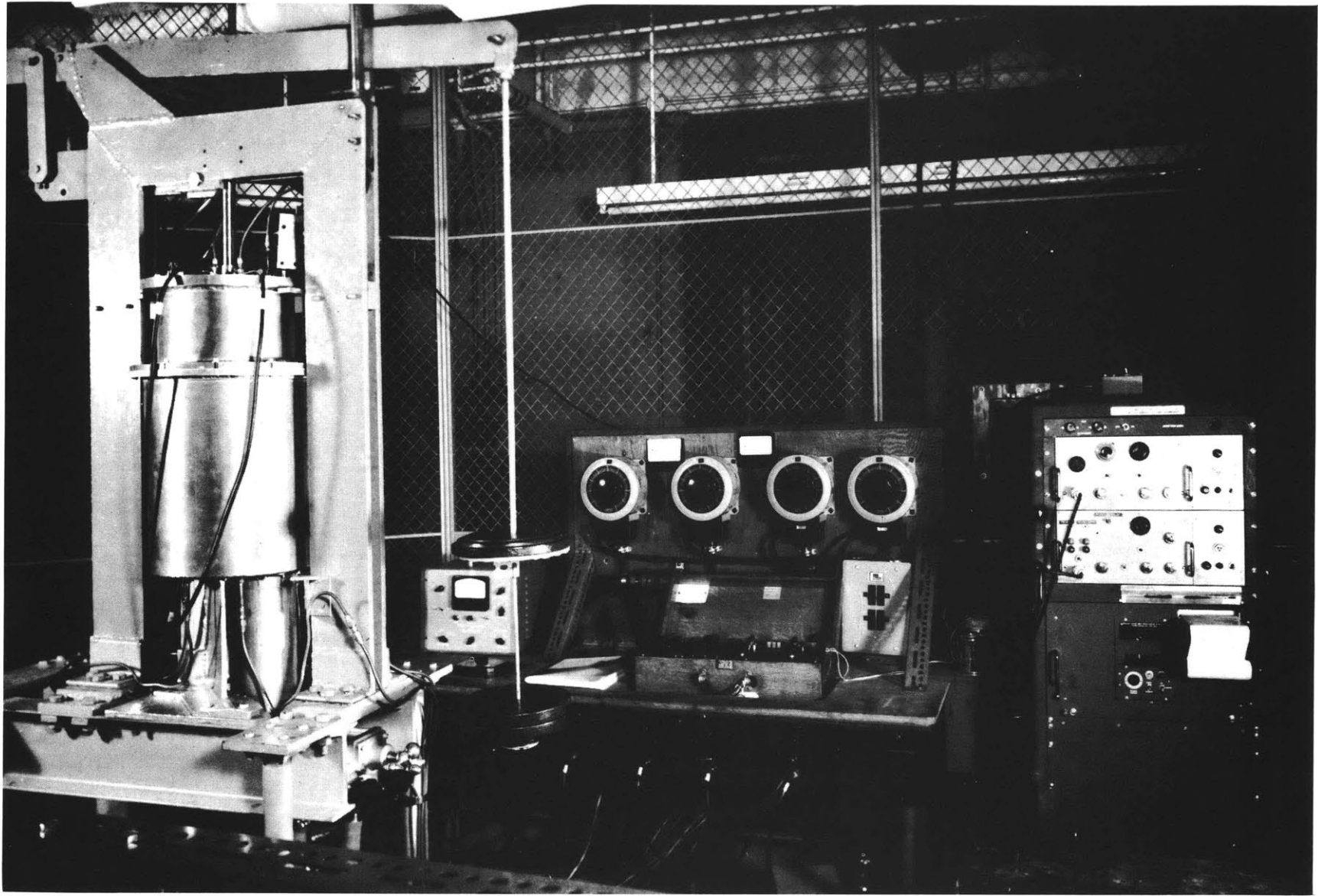
FIGURE 17: CONTACT RESISTANCE APPARATUS
