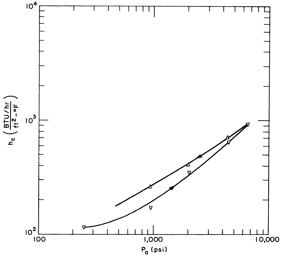
FIGURE 27. CONDUCTANCE VERSUS APPARENT PRESSURE STAINLESS STEEL
