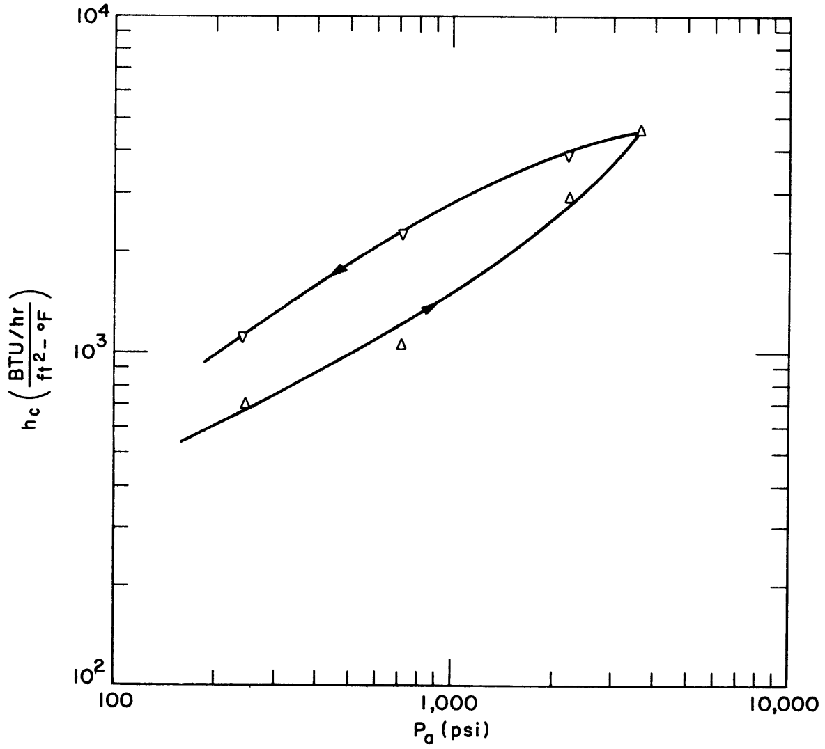
FIGURE 28. CONDUCTANCE VERSUS APPARENT PRESSURE MAGNESIUM
