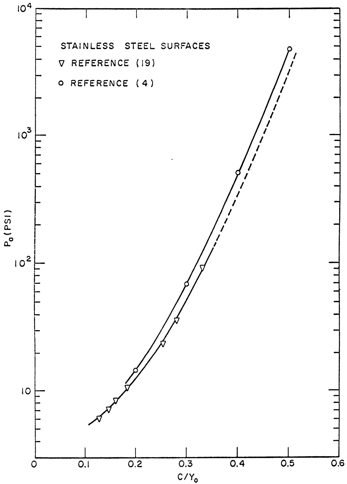
FIGURE 31. APPARENT PRESSURE VERSUS COMPLIANCE RATIO
