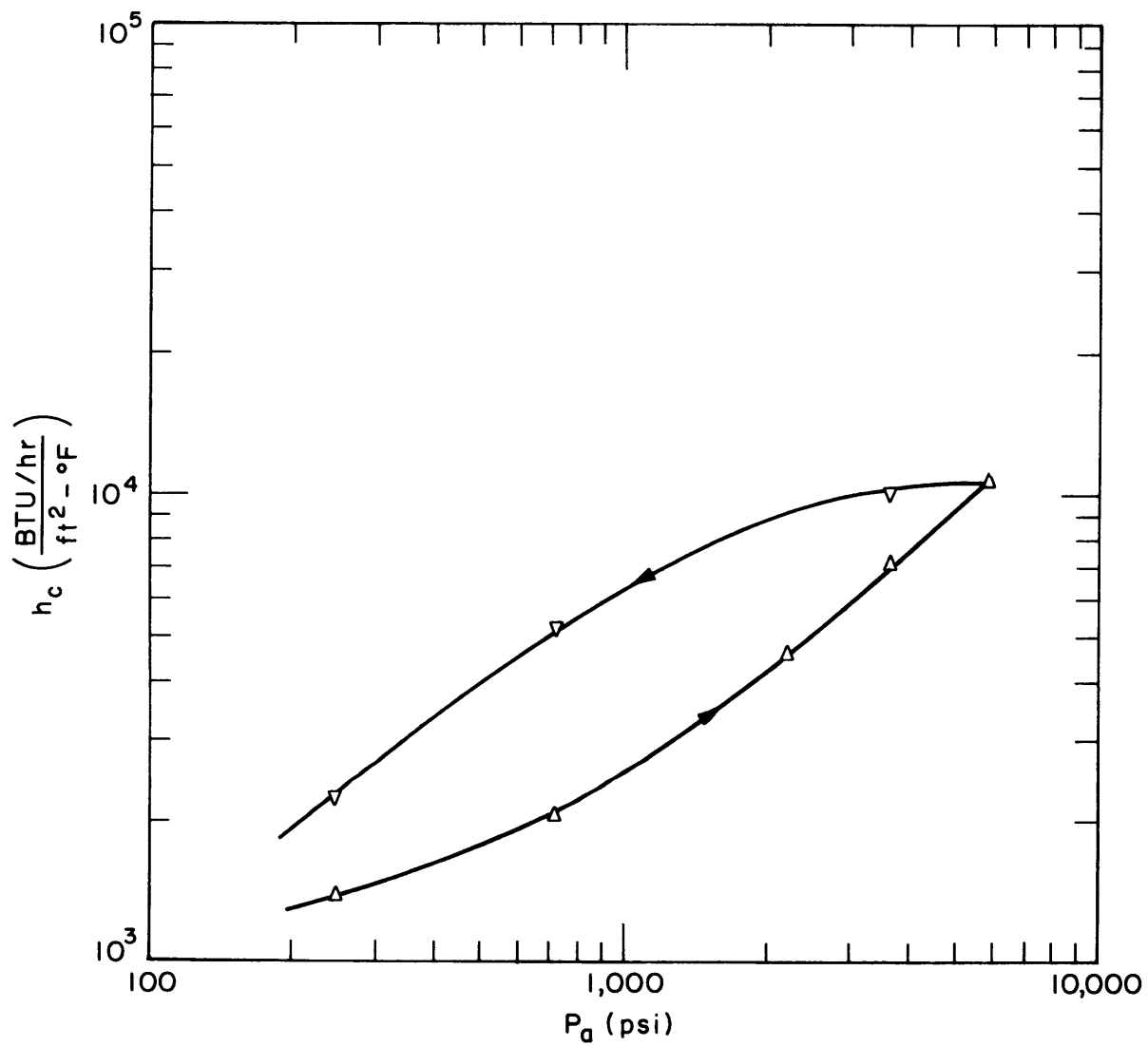
FIGURE 26. CONDUCTANCE VERSUS APPARENT PRESSURE ALUMINUM
