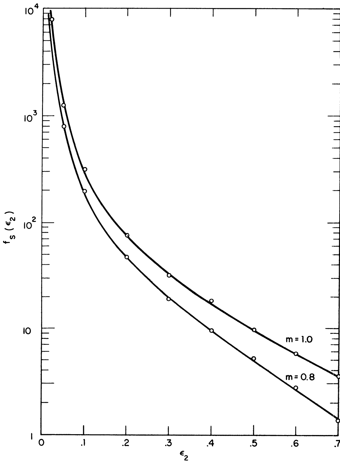
FIGURE 8. CONTACT CONDUCTANCE FACTOR FOR CYLINDRICAL WAVINESS
