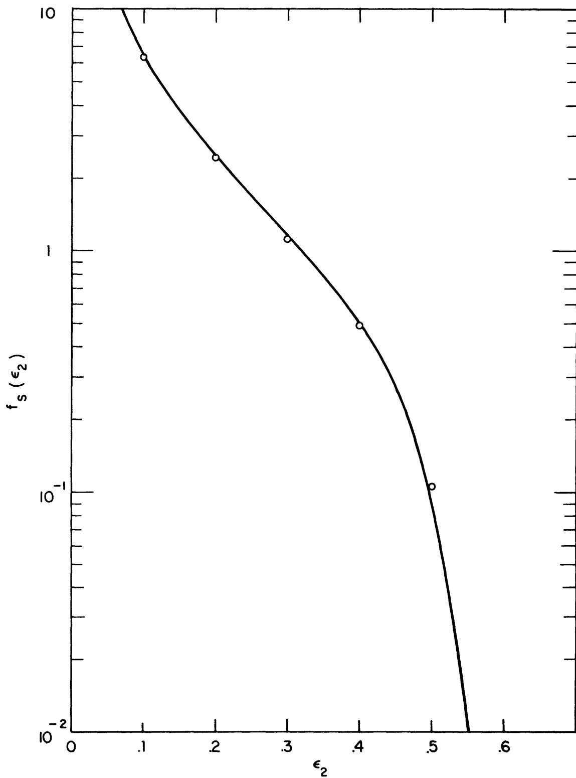
FIGURE 9. CONTACT CONDUCTANCE FACTOR FOR SPHERICAL WAVINESS
