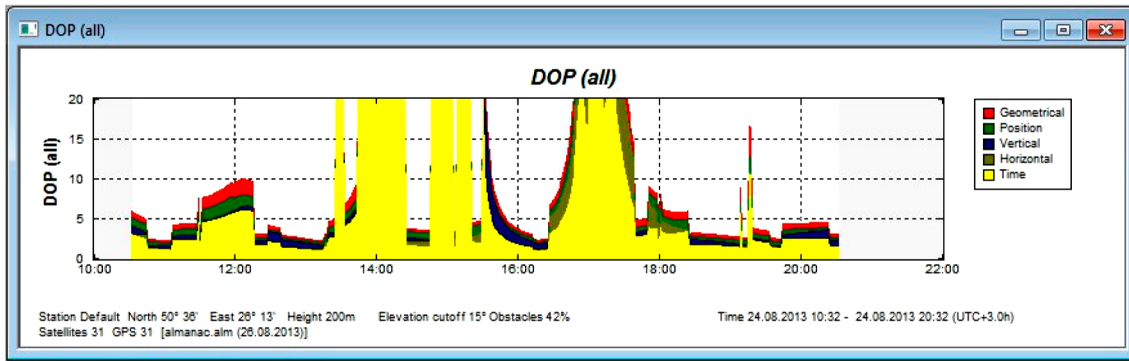
Fig. 4. Value of DOP criteria for the point 001 with the horizon closedness 42% received from the program planning
