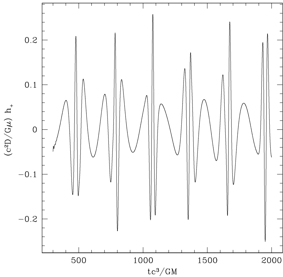
Figure 3: Waveform arising from a generic geodesic black hole orbit, neglecting orbital evolution due to backreaction. This orbit has p = 8GM/c^2 and e = 0.5 , corresponding to motion in the range 16GM/3c^2 \leq r(t) \leq 16GM/c^2 ; it also has \theta_{\min} = 60^\circ . The large black hole has a spin parameter a = 0.9M . Note that the wave has structure at several timescales, corresponding to the three frequencies \Omega_r , \Omega_\theta , and \Omega_\phi (cf. Fig. 2).
