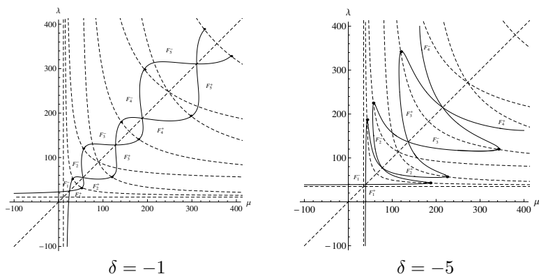
Figure 8. The spectrum of the problem (1.5), (1.6) for some negative \delta values.
