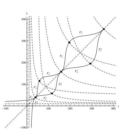
Figure 2. The spectrum of the problem (1.2).
