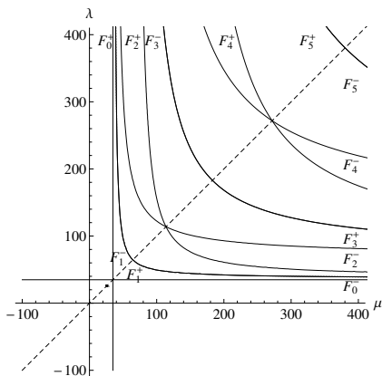
Figure 5. The spectrum of the problem (2.1) for \delta = 5 .
