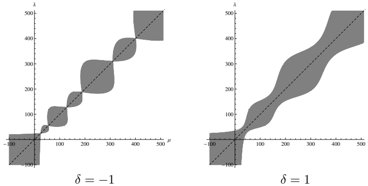
Figure 9. Solvability regions for the the problem (1.7), (1.6).
