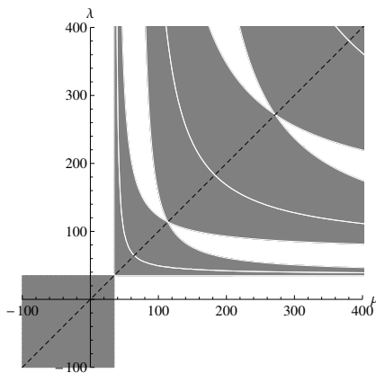
Figure 6. The solvability regions for the problem (2.2) for \delta = 5 .
