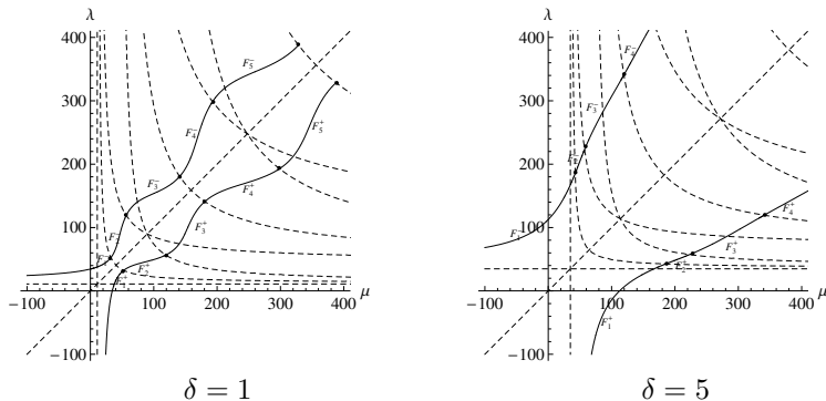
Figure 7. The spectrum of the problem (1.5), (1.6) for some positive \delta values.
