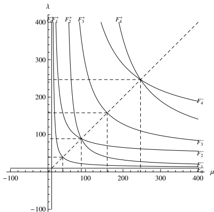
Figure 1. The spectrum of the problem (1.1).
