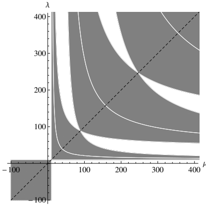
Figure 3. The solvability regions for the problem (1.3).
