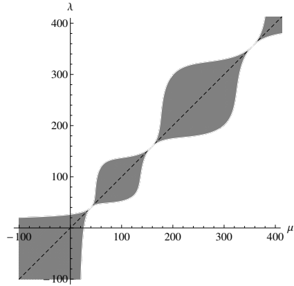
Figure 4. The solvability regions for the problem (1.4).
