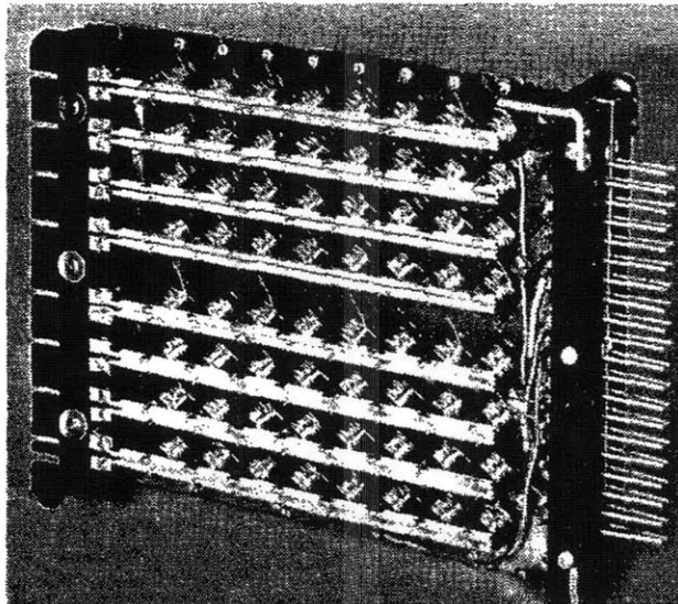
Figure 2-23: Ferreed switch containing 64 crosspoints, used to switch telephone calls by Bell System 1ESS Switch, the first electronic telephone switching system, which went into service in 1960. (Reprinted from "The No. 1 Electronic Switching System, Ketchledge, 1965) [49]
