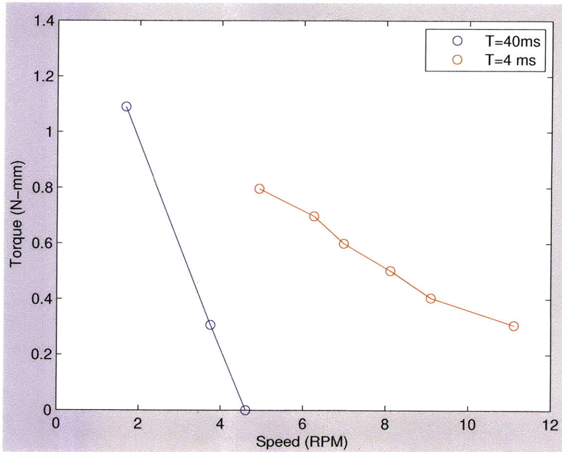
Figure 5-25: EP stepper torque vs. speed curves, measured by hanging weights on a string from the rotor, and measuring the time for one revolution with a stopwatch.
