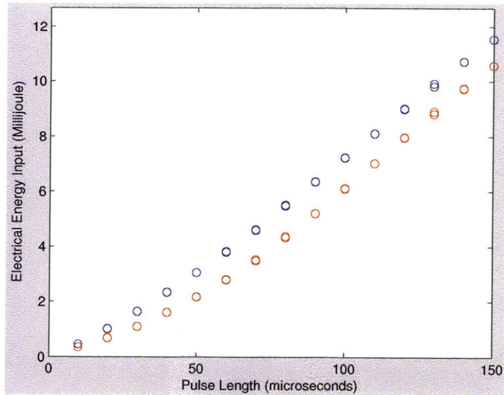
Figure 5-9: EP actuator electrical pulse energy vs. pulse length. Blue dots are the measured electrical pulse energy, \int VIdt over the pulse. Red dots are the I^2R dissipation, \int I^2Rdt , using a value of R measured using an ohmmeter.
