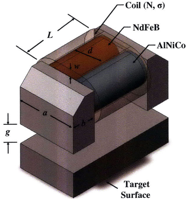
Figure 3-1: Switchable electropermanent magnet construction.
