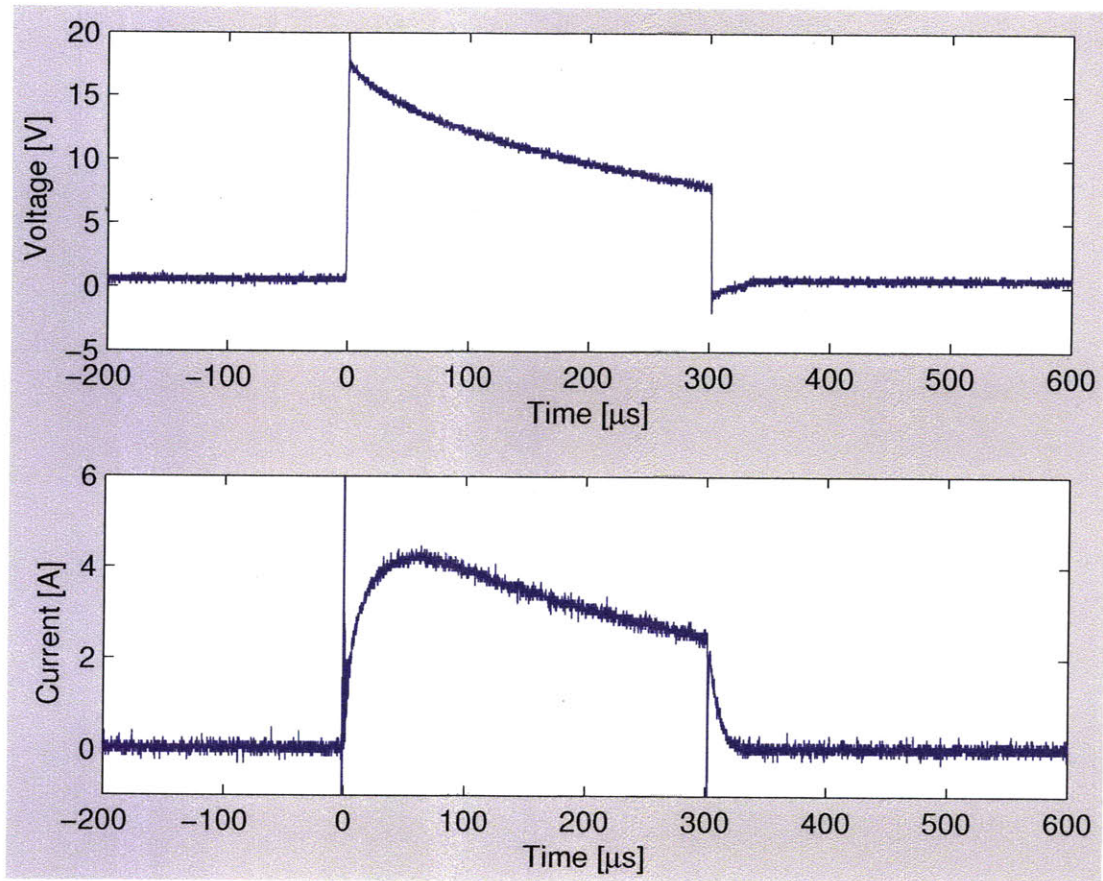
Figure 4-8: Voltage and current vs. time through the electropermanent magnet coil, driven with a 300\mu\text{s} pulse from the 100\mu\text{F} module energy storage capacitor. The peak magnetizing current of 4.2 A is reached after 60\mu\text{s} .
