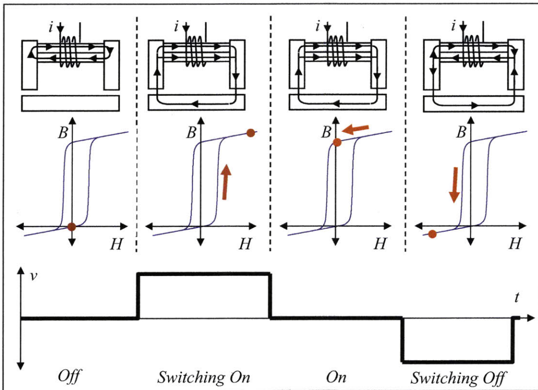
Figure 3-2: Switchable Electropermanent Magnet Operation. In the off state, the two magnetic materials are oppositely polarized, so magnetic flux circulates inside the device, and there is no force on the target. In the on state, the two magnetic materials are polarized in the same direction, so magnetic flux travels outside the device and through the target, attracting it to the magnet. A current pulse in the coil of proper magnitude and sufficient duration switches the device between the on and off states, by switching the polarization of only the Alnico magnet, which has a lower coercivity than the NIB magnet.
