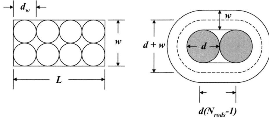
Figure 3-3: Left: Cross-section view of coil. Assuming square wire packing, the sum of the area of the bounding boxes around each wire equals the total cross-sectional area of the coil, so Nd_w^2 = Lw . Right: Side view of the coil. The dotted line shows the middle turn, distance w/2 from the core. This is an average-length turn; the total length of the wire is N times the length of this turn. By adding the lengths of the straight segments and circular caps, we can find the length of the wire, l = N(2d(N_{rods} - 1) + \pi(d + w)) .
