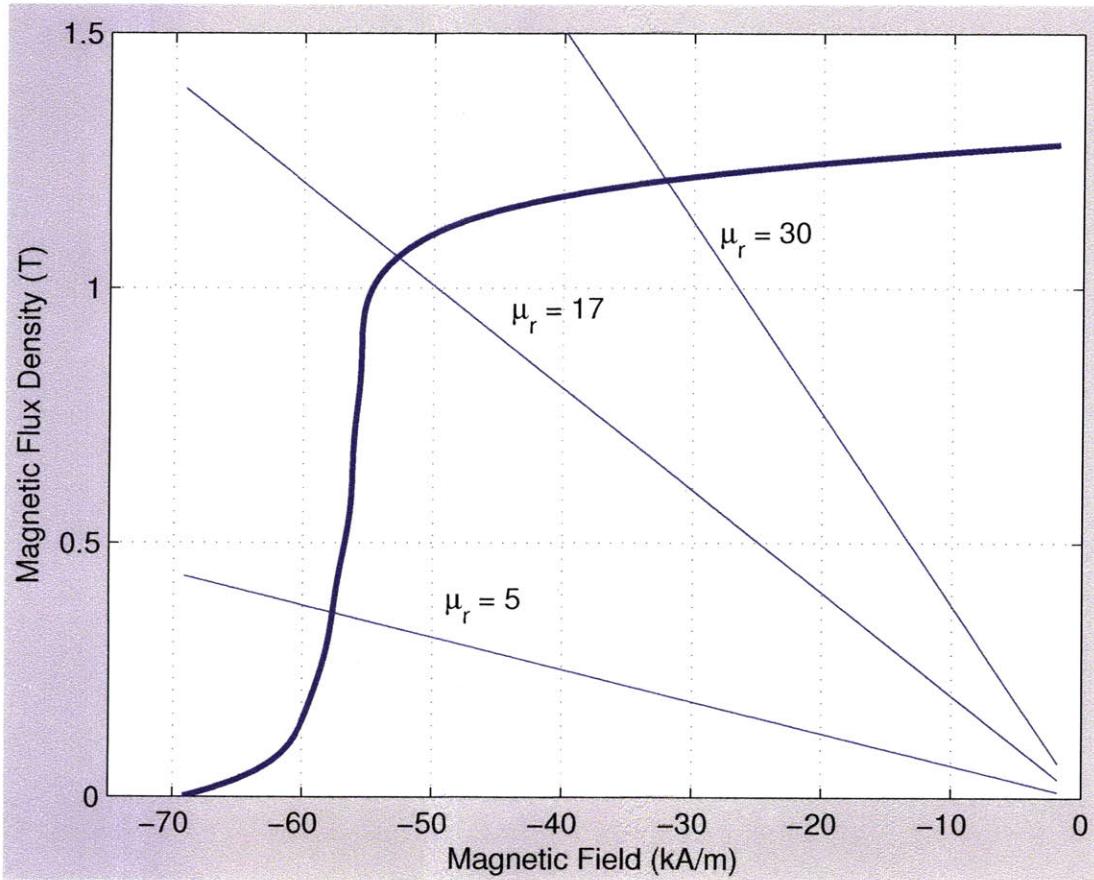
Figure 5-21: Load line analysis. The second-quadrant hysteresis curve for Alnico V in parallel with NdFeB is plotted with three gap load lines. The magnet/gap size ratio \mu_r is defined in the text; for a design with equal permanent magnet and pole area, it is equal to the ratio of the total magnet length on the flux path to the length of the air gap. The system will start the power stroke at the intersection of the load line and the hysteresis curve.
