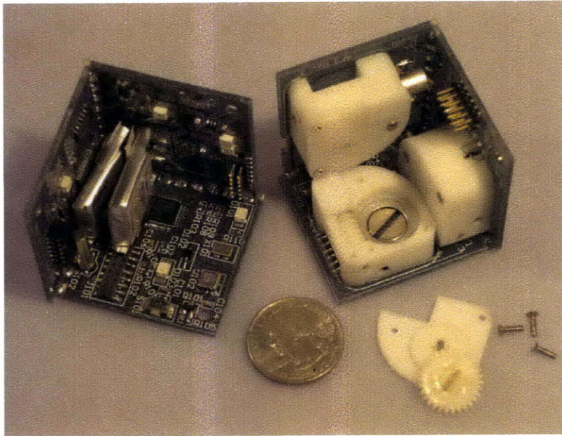
Figure 2-19: A disassembled MICHE module, showing the lithium polymer batteries, mechanically switched permanent magnets, and circuitry. [33]
