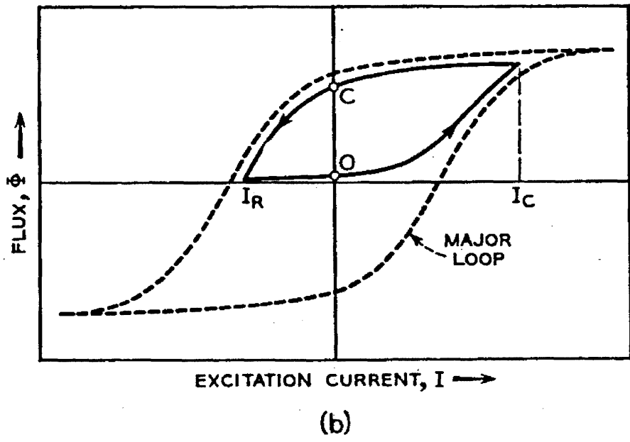
Figure 2-22: (a) The single-branch ferreed (b) its magnetization characteristic. (Reprinted from "The Ferreed — A New Switching Device", Feiner, Lovell, Lowry, and Ridinger, 1960) [23]
