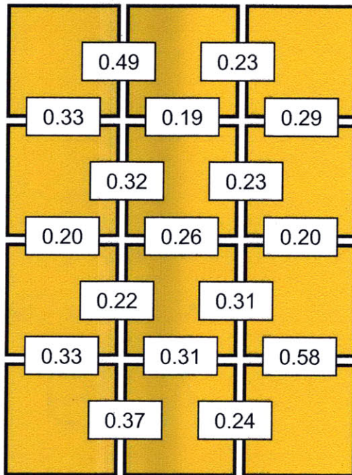
Figure 4-9: Electrical resistance of power connections in a block of pebbles, in ohms, measured with an ohm-meter on an un-powered block of pebbles. The mean resistance is 0.3\Omega . For each connection though which the power for a pebble travels, the I^2R dissipation at 11mA is 27 \mu\text{W} . This is about 10,000 times less than the power used by the pebble to power its microcontroller and LED, 220 mW.
