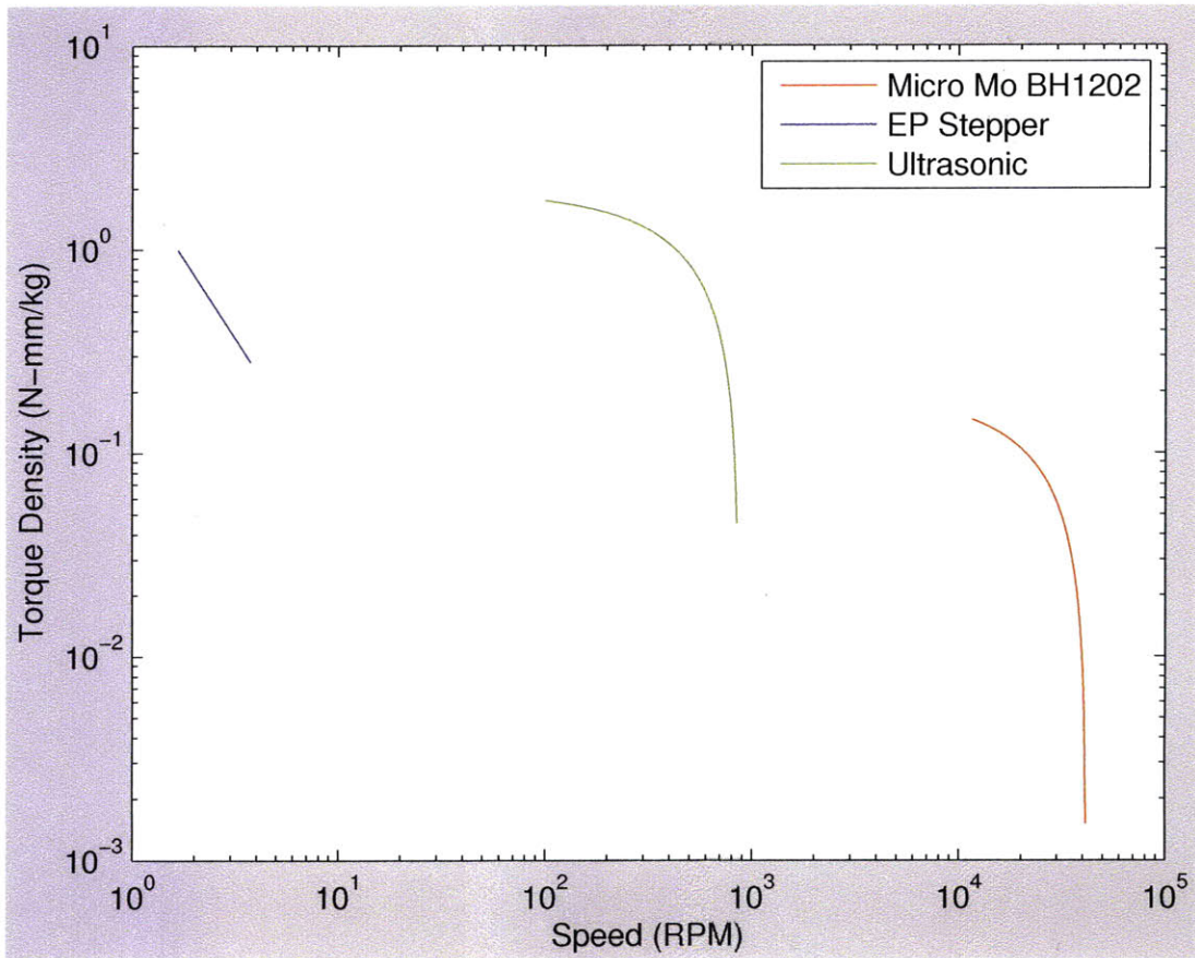
Figure 5-27: Torque density vs. speed comparison with two motors of similar size to the EP stepper. The EP stepper torque/speed curve at T=40 ms is plotted against the torque speed curve for a Micro-Mo BH1202 electromagnetic penny motor and Flynn's 8 mm diameter ultrasonic motors. [TODO CITE] The EP stepper has higher torque density than the electromagnetic motor, but lower torque density than the ultrasonic motor.
