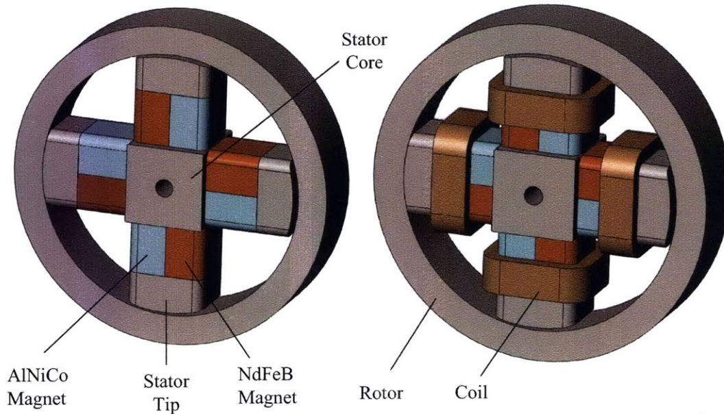
Figure 5-16: Electropermanent stepper construction.
