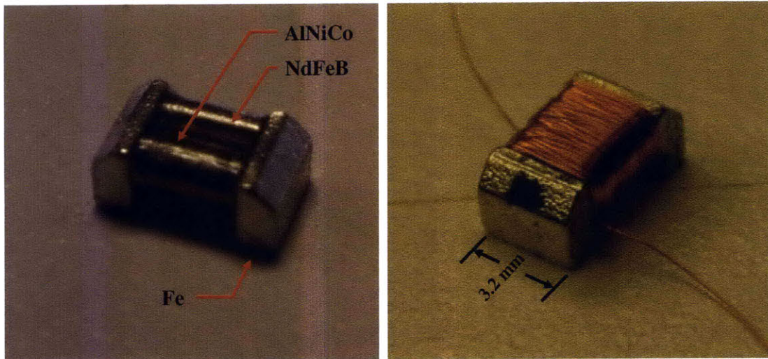
Figure 1-1: Miniature electropermanent magnet. This magnet is made from cylindrical rods of hard Nd-Fe-B, semi-hard Alnico, iron pole pieces, and a copper wire coil. The magnet can hold 4.4 N, which is over 2000 times its own weight, switches with a 5 mJ electrical pulse, and holds its state zero power.
