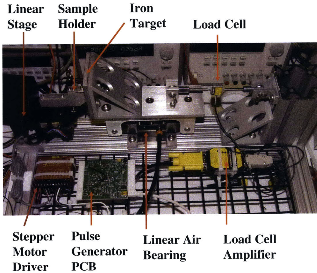
Figure 3-8: Experimental setup used to measure the force vs. displacement relationships.
