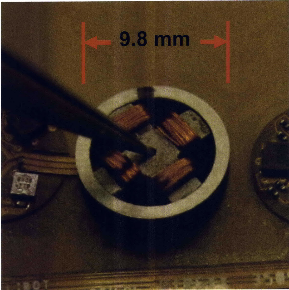
Figure 5-15: Electropermanent stepper motor, being driven by the millibot electronics. The stator is fixed by a pair of tweezers, and the outer ring rotates. A pair of Alnico and NdFeB permanent magnets are located under each coil, making each arm of the stator an electropermanent magnet.
