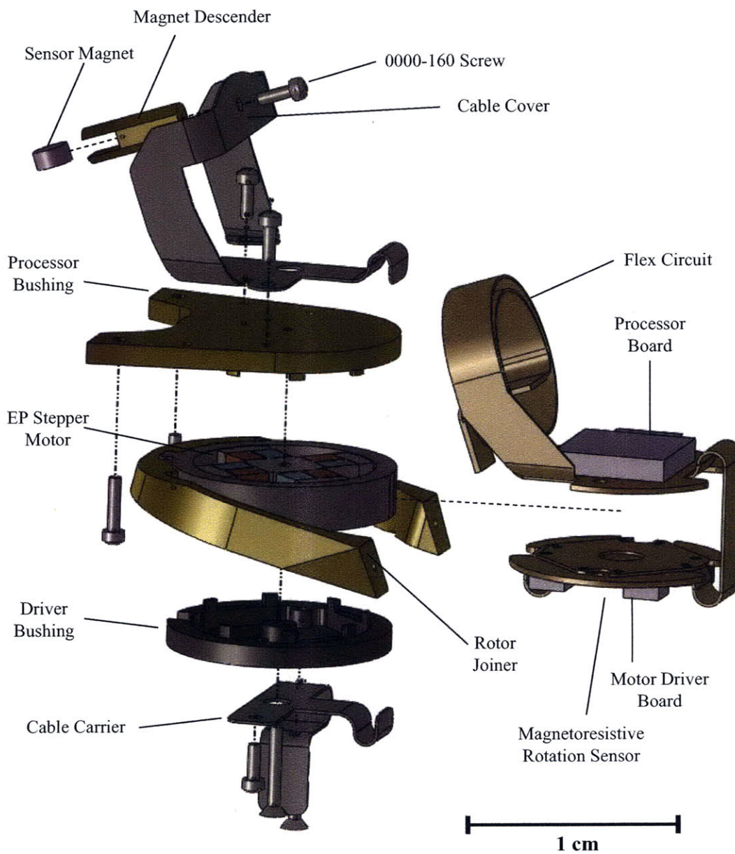
Figure 6-6: Millibot module exploded view. This assembly is repeated for each joint. One segment of the continuous flex circuit is shown in its folded configuration. The electropermanent stepper motor rotates the rotor joiner relative to the rest of the assembly. The rotor joiner connects to the processor bushing of its neighbor using two screws. See Figure 6-7 for an assembled view.
