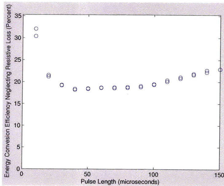
Figure 5-12: EP actuator efficiency after subtracting ohmic loss. These plots are for a magnet slowly pulled away from an iron plate. The efficiency is the total mechanical work divided by the electrical energy in two switching pulses after subtracting I^2R losses using the measured values of I(t) and R .
