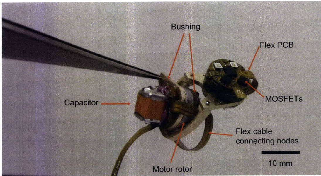
Figure 6-1: A two-module millibot, showing the major components.
