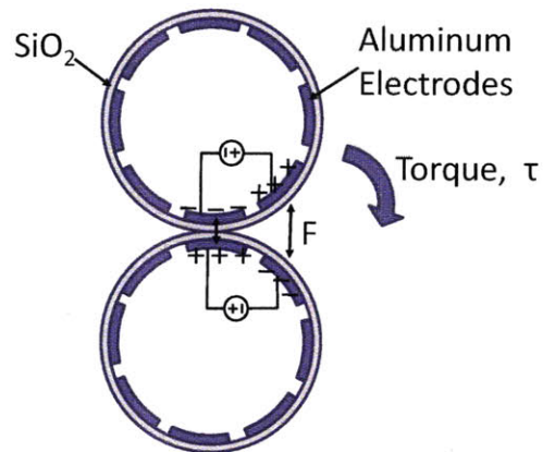
Figure 2-11: Electrostatic Catom actuation: The force from the electric fields between the capacitor plates will move the Catoms. [48]
