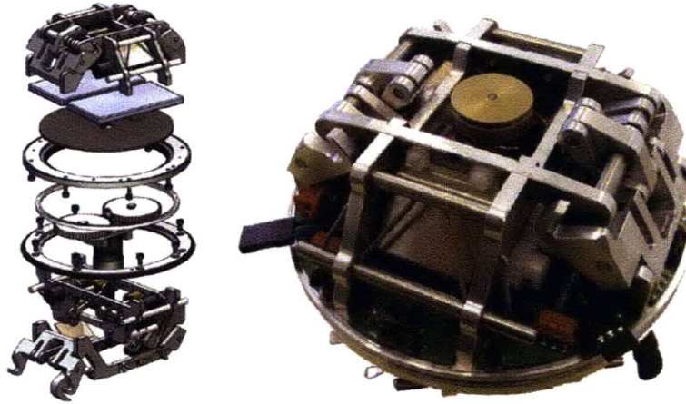
Figure 2-8: ATRON Module Mechanics. [67]
