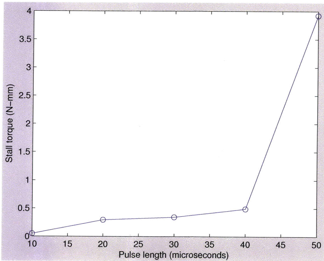
Figure 5-26: EP stepper torque vs. pulse length, measured by hanging weights on a string from the rotor until the motor backdrove. This plot shows that the stall torque of the motor is considerably higher than its dynamic torque and that the torque can be controlled by the driving pulse length.
