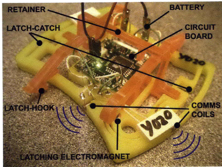
Figure 2-15: One of Griffith, Goldwater, and Jacobson’s Electromechanical Assembler Modules.
