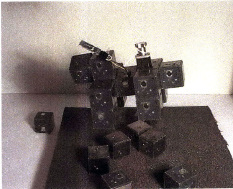
Figure 2-20: MICHE system forming a 15-module dog out of a 27-module block. The mechanically-switched permanent magnets release un-needed modules and they fall away. [33]
