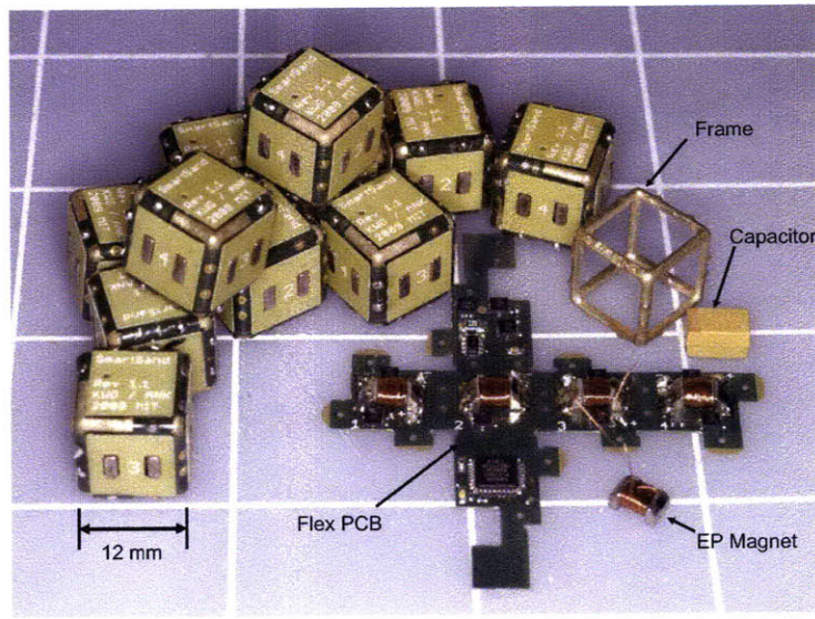
Figure 1-3: The Robot Pebbles are fully printed-circuit integrated, solid-state programmable matter. All of the components, including the four electropermanent magnet connectors and the frame are soldered to a flexible printed circuit board. The electropermanent magnet connectors provide mechanical connection, electrical power transfer, and inductive communication between modules.
