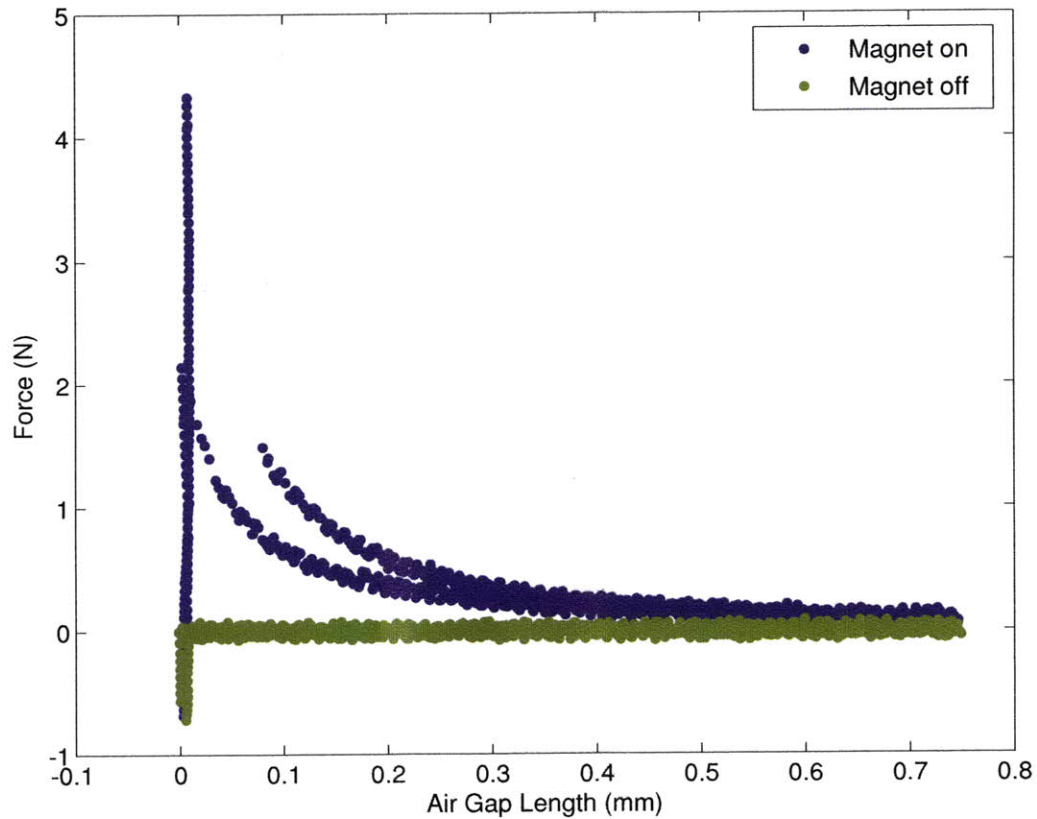
Figure 3-13: Attractive force vs. air gap length. The device was switched on while in contact with the plate, pulled away to a distance of 0.75 mm, returned to the plate, switched off, and pulled away again. While still in contact with the plate, the peak force reached 4.4 N. When the linear stage drove the device further from the target, the device broke away from the plate dynamically, reaching a new static equilibrium (between the magnetic force and load cell stiffness) at a distance of 0.07 mm, which is why there are no data points on the upper curve between 0 and 0.07mm. The middle curve shows the magnet returning to the plate; the force is lower because the device has been partially self-demagnetized. The lower (green) curve shows that, with the magnet switched off, the force is near zero.
