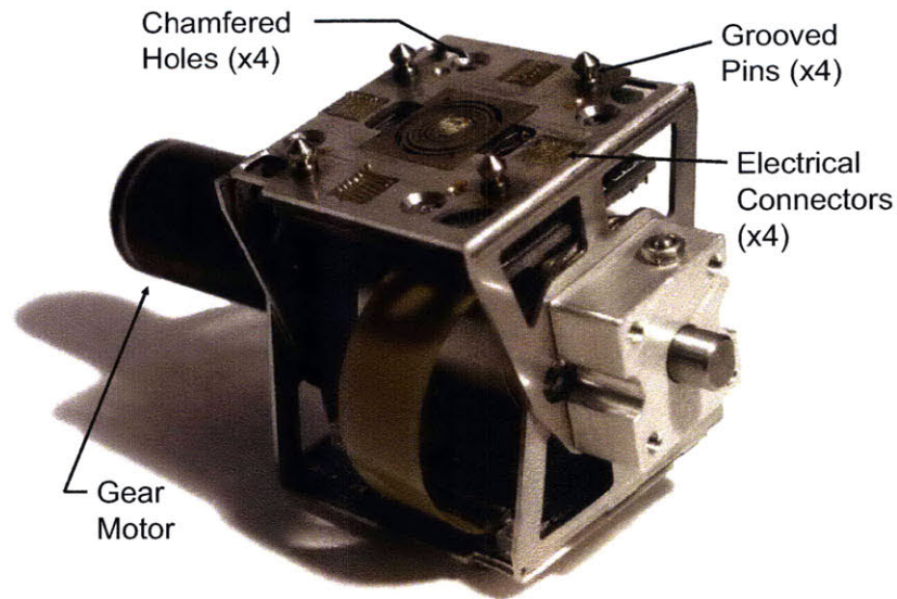
Figure 2-1: Polybot G2 segment module. The segment has a rotary joint and two square connection faces. Polybot also uses node modules, which are cubes with six connection faces. [94]
