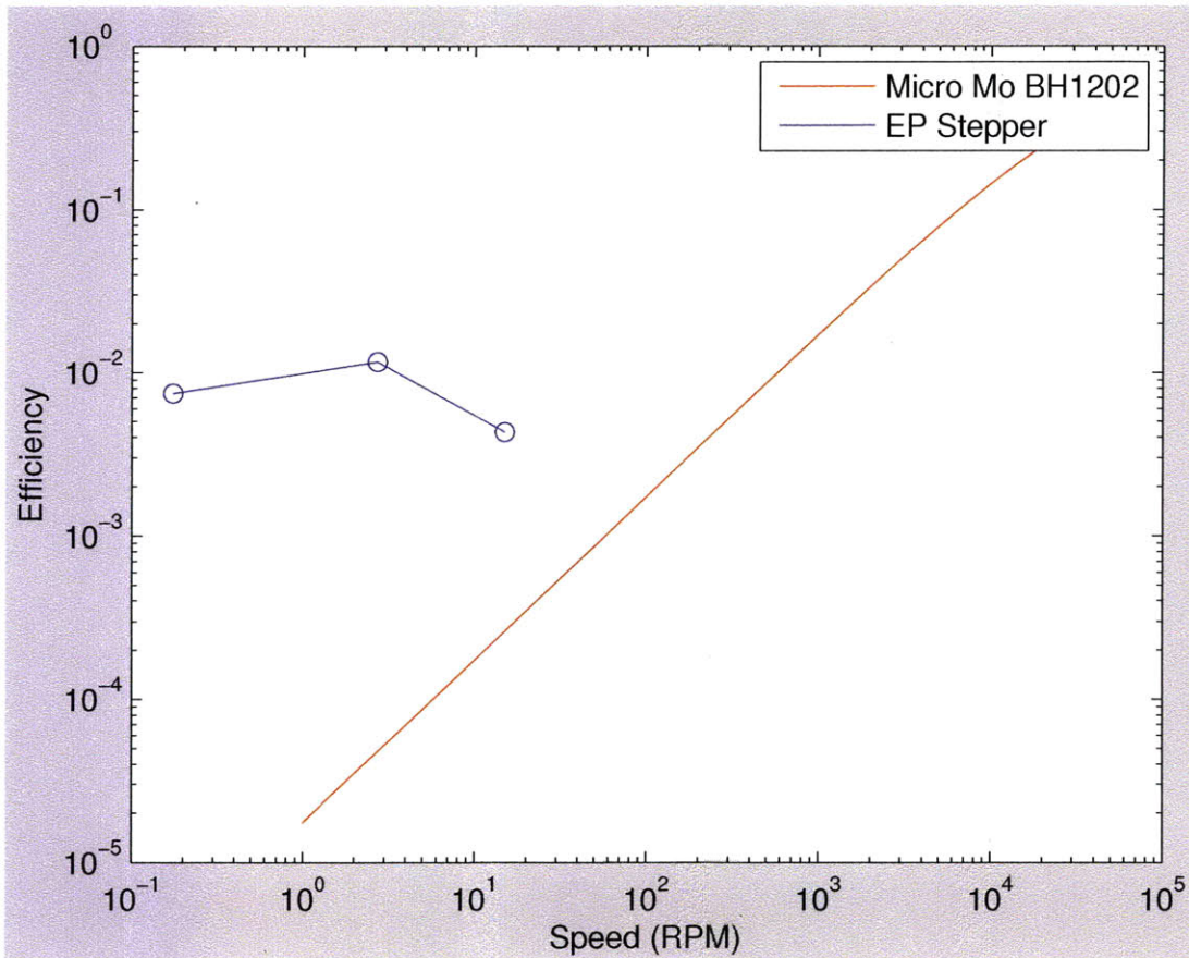
Figure 5-28: Efficiency vs. speed comparison with the Micro-Mo BH1202 electromagnetic motor. Lifting the maximum rated load of the BH1202, 0.16 N-mm, the EP stepper has 1% efficiency, independent of driving pulse length. The Micro-Mo BH1202 has lower efficiency than this at speeds below 1000 RPM. Note that this is a log-log plot.
