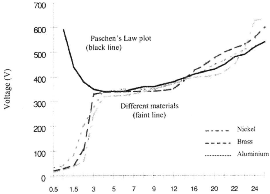
Figure 3-4: Breakdown voltage of air vs. gap [28].
