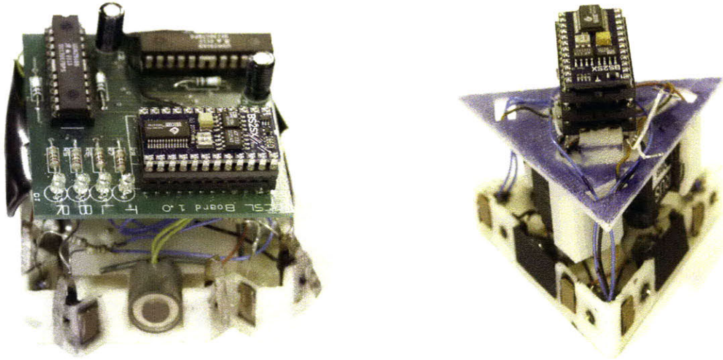
Figure 2-17: White, Kopanski, and Lipson's Magnetic Modules for Stochastic Self-Reconfiguration. (a) Square unit with electromagnets. (b) Triangular unit with swiveling permanent magnets. [90]
