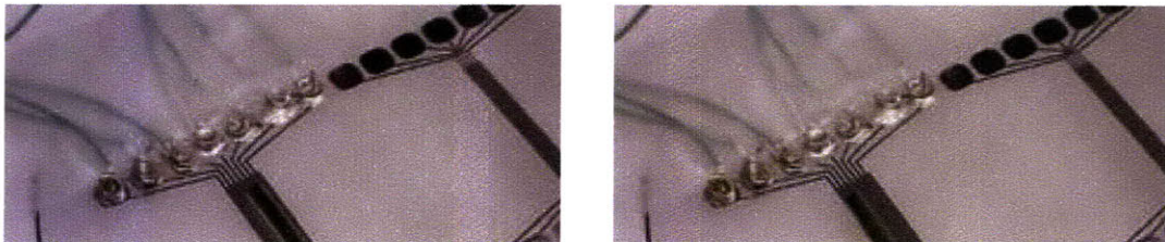
Figure 2-12: Demonstration of electrostatic actuation of a 1 mm aluminum tube, showing proof of concept for the Electrostatic Catoms. [48]
