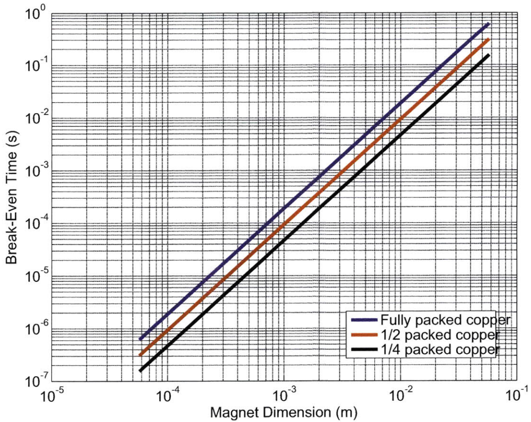
Figure 3-6: Time to break-even energy consumption for electromagnets vs. electropermanent magnets, for a scaled version of the device described in this paper. At centimeter scale, the break-even time is about 10 ms, and at millimeter scale, 100\mu\text{s} . The break-even time gets lower with reduced wire packing density.
