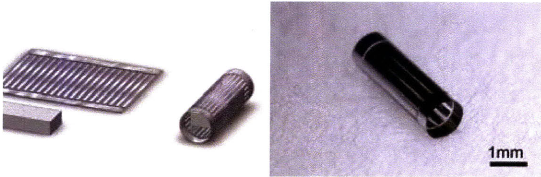
Figure 2-10: Microfabrication process for aluminum-on-silicon-dioxide tubes to be used for the electrode shells of electrostatic Catoms. [48]
