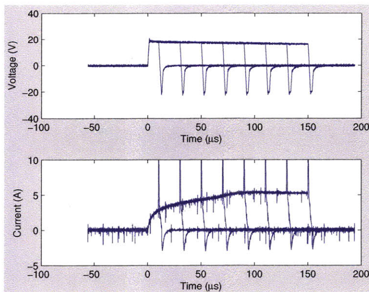
Figure 5-13: EP actuator pulse voltage and current vs. time. In the figures above, we have overlaid the plots for eight linearly-spaced pulse lengths from 10 \mu\text{s} - 150 \mu\text{s} . Demonstrating the causality and repeatability of the system, the pulses follow identical trajectories until the voltage is turned off, when a negative-voltage spike corresponding to the partial collapse of the magnetic field is observed.
