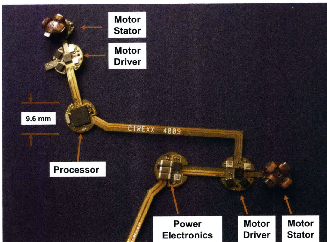
Figure 6-3: Millibot flex circuit. The circuits link together in a continuous hot-air reflow-soldered chain. Shown is the electronics to drive two joints: one microcontroller, one power electronics board, two motor driver boards, and the stators of two motors.
