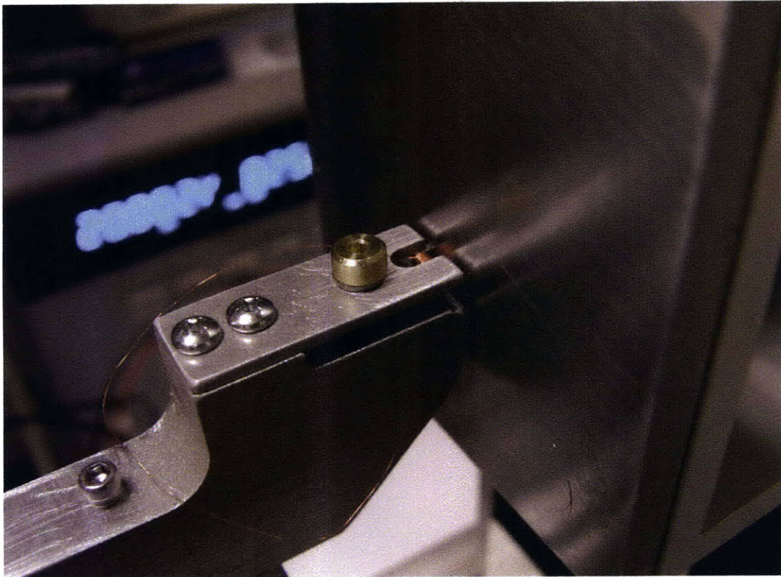
Figure 3-9: Flexure clamp used to hold magnet square as it is pulled away from the iron target plate.
