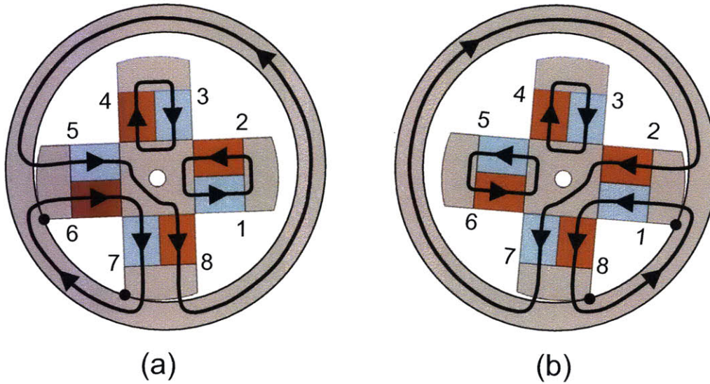
Figure 5-17: EP stepper principle of operation. The red magnets are NdFeB, always polarized in the direction shown. The magnetization of the blue AlNiCo magnets switches as the motor operates. The motor starts in position (a), with magnets 5-6 and 7-8 on, and magnets 1-2 and 3-4 off. Flux flows through the rotor and stator as shown. Applying a current pulse to the horizontal winding around magnets 5-6 and 2-1 switches the magnetization of magnets 5 and 1, turning magnet 5-6 off and magnet 2-1 on, resulting in the new flux paths shown at right. The rotor pivots counterclockwise about magnet 7-8, taking one step to arrive at the new position shown in (b). Repeated steps drives the rotor around the stator with a continuous rotary motion and oscillating translational motion.
