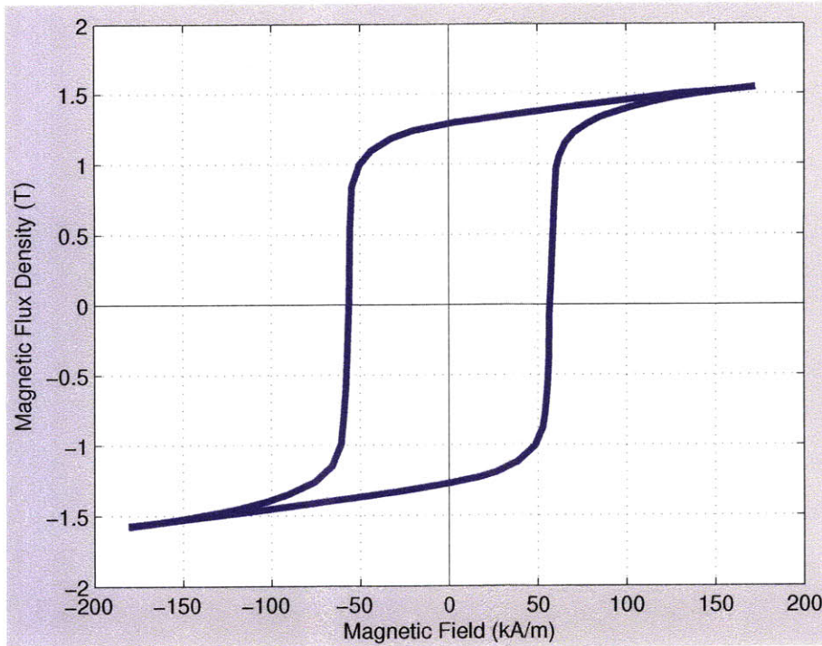
Figure 2-21: Hysteresis loop of AlNiCo V. (Data from Campbell [11])
