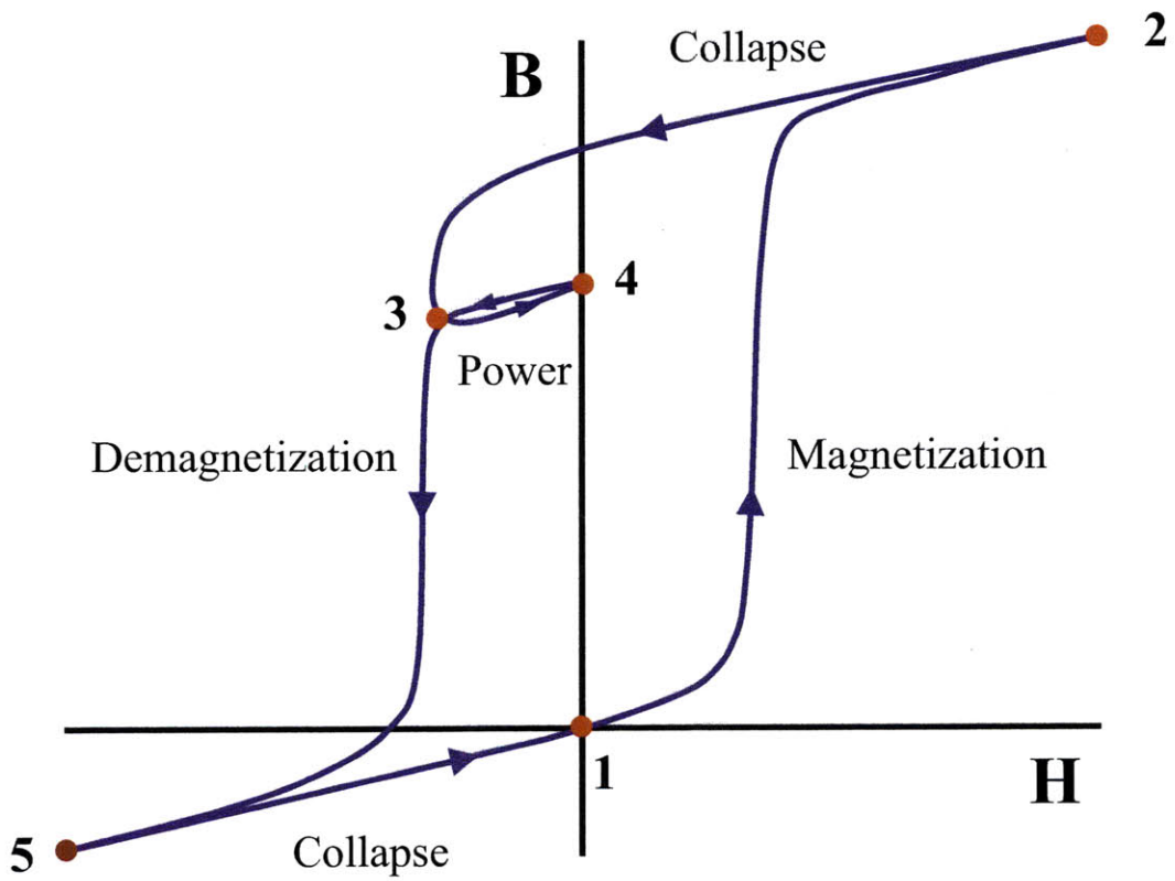
Figure 5-2: Electropermanent actuator thermodynamic power cycle.
