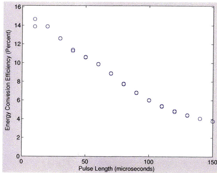
Figure 5-11: EP actuator efficiency vs. pulse length. These plots are for a magnet slowly pulled away from an iron plate. The efficiency is the total mechanical work divided by the electrical energy in two switching pulses.
