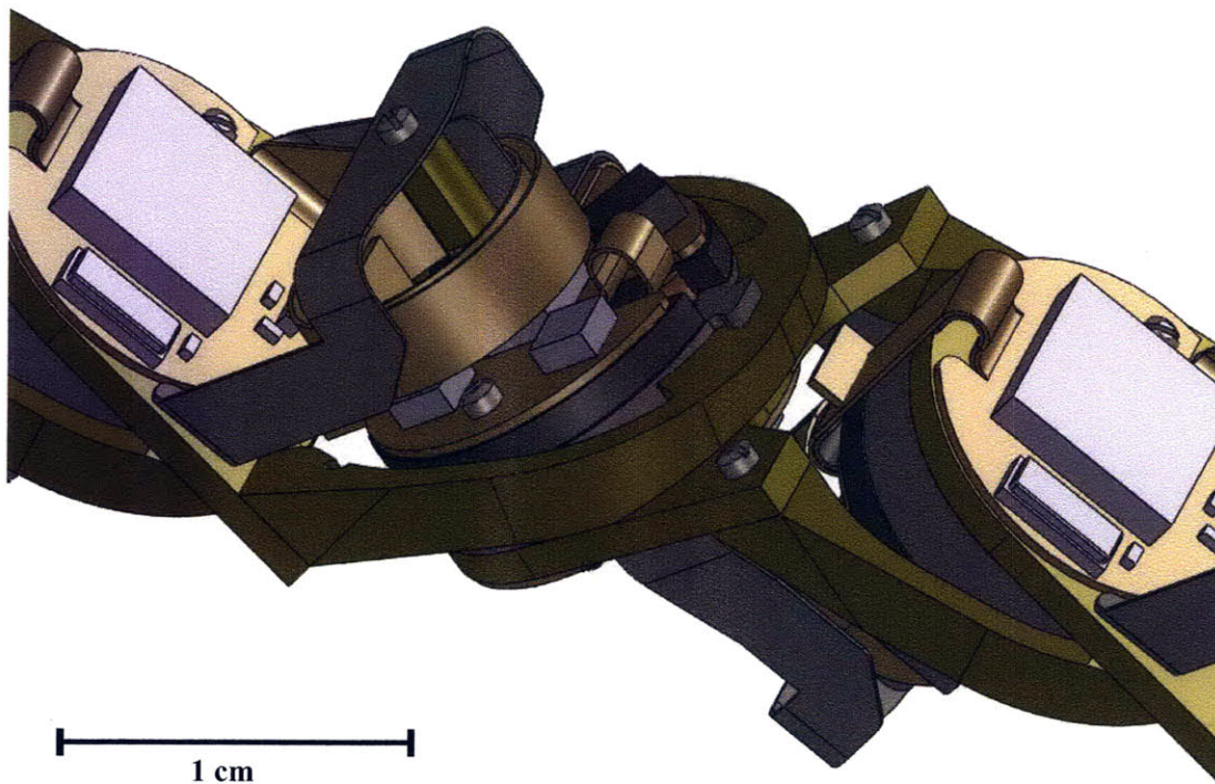
Figure 6-8: Millibot chain, assembled by building a millibot module around each section of the continuous flex circuit. This view shows how the rotor joiner of each module attaches to the processor bushing of its neighbor. When the chain is assembled, the sensor magnet is positioned above the magnetoresistive sensor of the next module. Power and data are transferred between modules over the coiled section of the continuous flex circuit.
