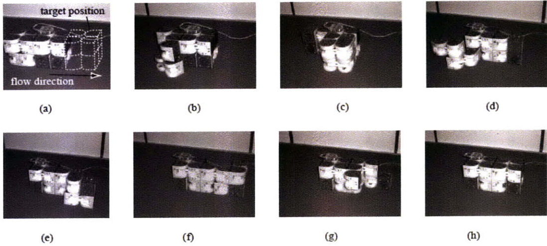
Figure 2-5: M-TRAN cluster flow experiment. A block of nodes can move along the floor as shown through self-reconfiguration. [62]
