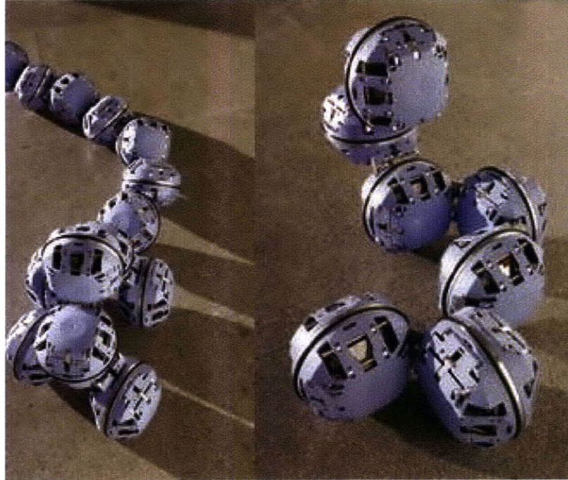
Figure 2-7: ATRON system, consisting of hemispheres connected by a rotary joint, and connected to each other by a right-angle bracket. The hemispheres are 110 mm in diameter. [67]
