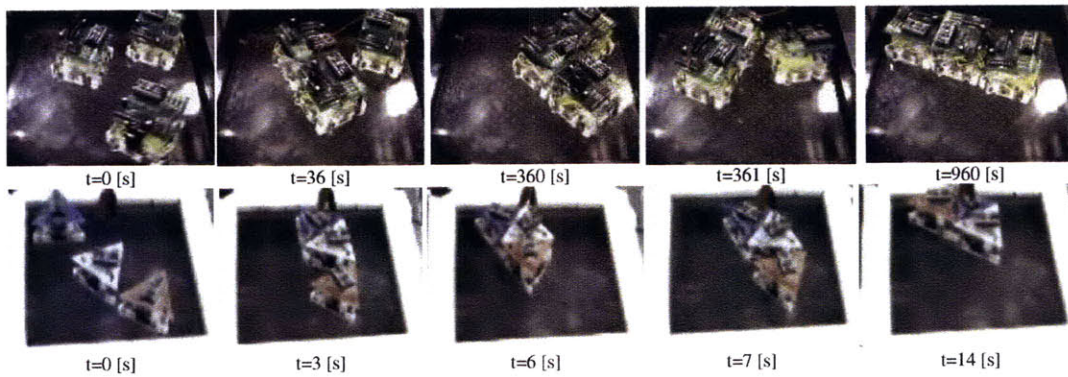
Figure 2-18: Stochastic self-reconfiguration of White, Kopanski, and Lipson's Magnetic Modules. The top row shows the square units assembling into a line. The bottom shows the triangular units. [90]
