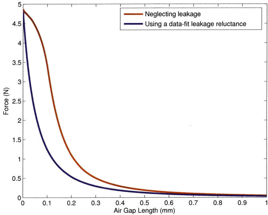
Figure 3-12: Force vs. air gap, computed using the magnetic circuit model, with and without leakage. The top curve neglects leakage, while the bottom curve uses a leakage permeance fit to match the finite element analysis result.
