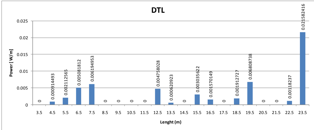
Figure 4.1.4.- Beam power loss map [watts per meter] in the DTL for 0.1 % duty cycle (700 V, field maps).
