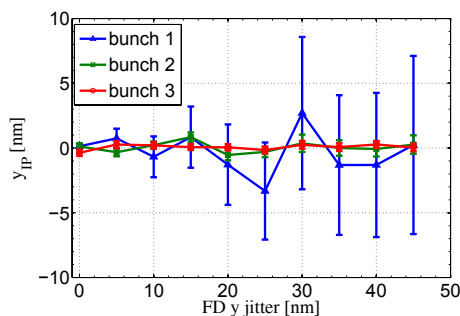
Figure 6: IP bunch position versus vertical position jitter of the FD magnets for operation with three bunches in ATF2, applying IP-FB correction.
