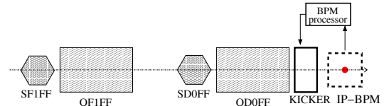
Figure 3: Schematic of a beam-based intra-train FB system at the IP of ATF2.
