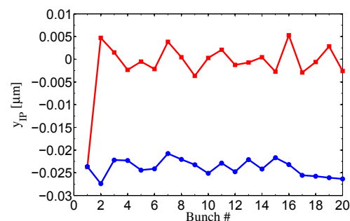
Figure 4: Example of vertical offset correction by an IP-FB system for operation with 20 bunches in ATF2. The blue line shows the vertical bunch position at the IP without IP-FB correction. The red line shows the bunch position at the IP with IP-FB correction.
