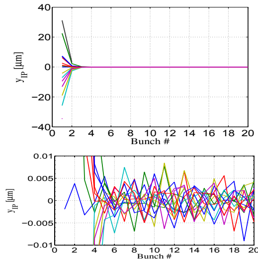
Figure 5: IP vertical bunch position correction by the IP-FB system for several vertical position jitters of the FD magnets in the range [0, 30] \mu\text{m} . On the bottom plot the ordinate scale has been reduced.
