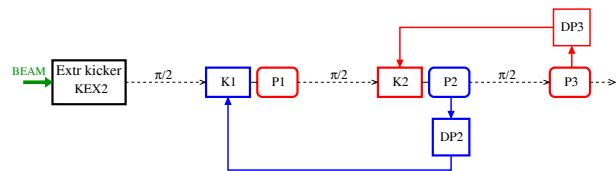
Figure 1: Scheme of an intra-train feedback system for the ATF2 EXT line, downstream of the second extraction kicker KEX2. K1 and K2 denote kickers; P1, P2 and P3 denote BPMs; and DP2 and DP3 digital processors.
