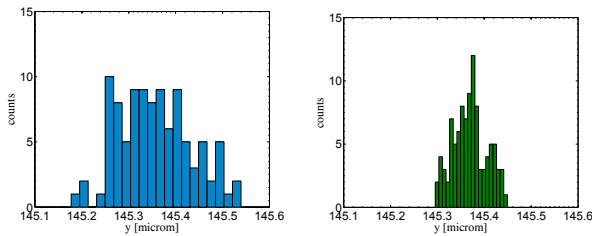
Figure 2: Beam position jitter distribution at the IP, without correction (left) and with FB correction (right).
