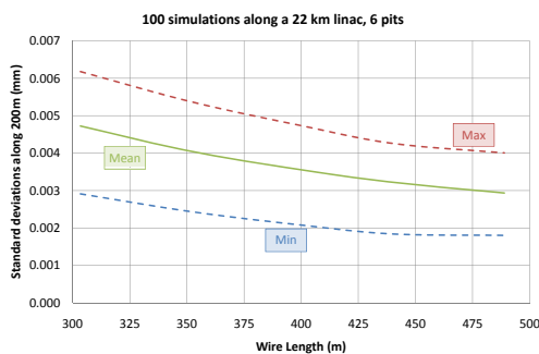
Figure 3: Simulations of the effects of the wire length.
