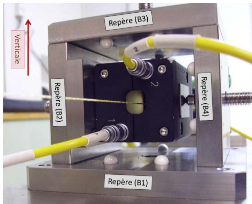
Figure 6: A sensor being calibrated.
