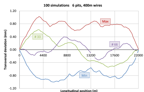
Figure 1: Propagation network simulations.
