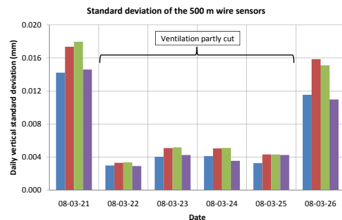
Figure 4: Standard deviations of the 500 m wire sensors.
