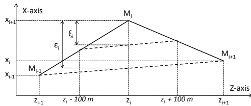
Figure 2: The deviation along 200 m.
