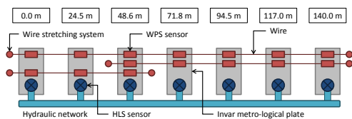
Figure 7: Layout of the TT1 facility.
