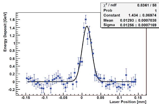
Figure 3: Convoluted horizontal size of 13 microns measured by BSM in laser wire mode in March of 2009.
