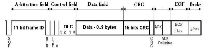
Figure 4. CAN standard data frame
