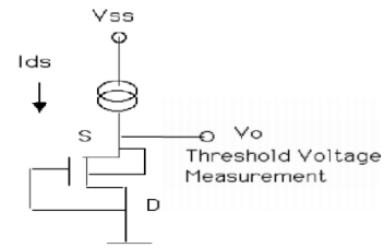
Figure 6. RadFET reader circuit configuration
