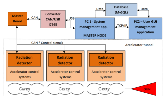
Figure 1. Block diagram of Radiation Monitoring System based on CAN
