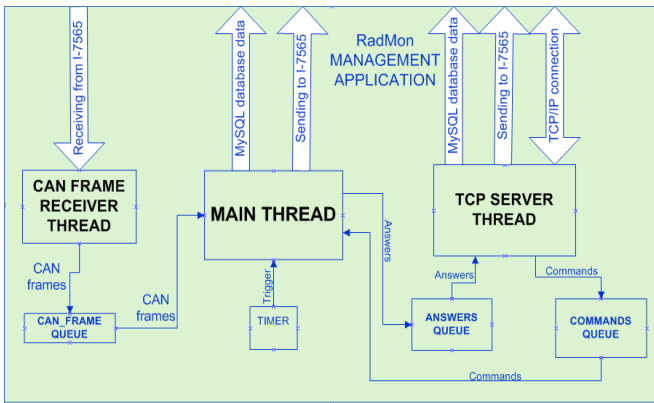
Figure 7. Block diagram of Management Application
