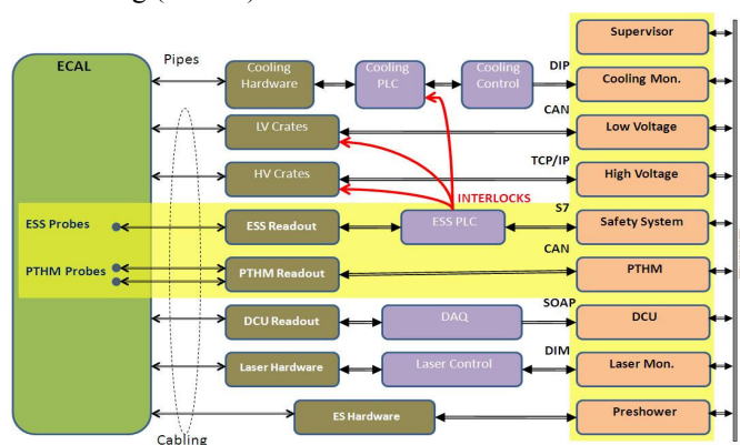
Figure 1: CMS ECAL DCS block diagram (simplified)
