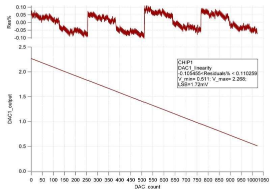
Figure 10: DAC linearity.
