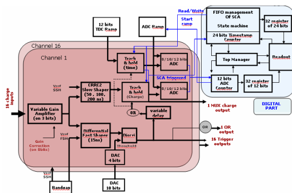
Figure 2: PARISROC global schematic.
