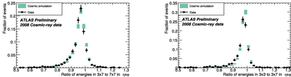
Figure 4: Lateral shower containment along \eta (left) and \phi (right), for photon clusters with E_T > 5 GeV in the barrel EM calorimeter.
