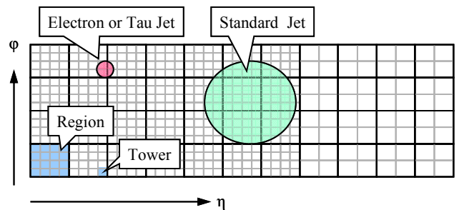
Figure 3: A portion of the RCT input geometry. Only 4 of the 18 regions in \phi are shown and only 1/2 of \eta . The approximate size of an electron, tau and normal jet are shown to give the reader an indication of size.
