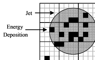
Figure 4: The 3x3 regions required to encompass a jet centred on a tower somewhere in the central region. If a single tower is considered the centre of the jet then the algorithm could sum energy depositions from up to 9 towers in each dimension.
