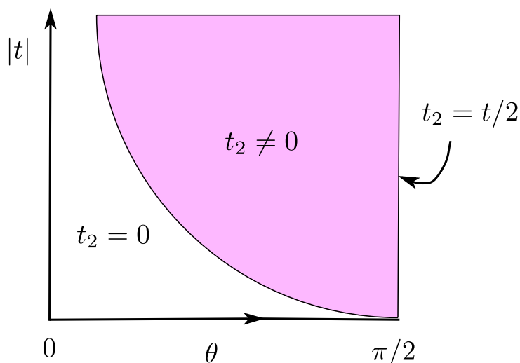
Figure 7. The phase diagram describing the large N limit of Chern-Simons theory on L(2,1) for 0 \leq \theta \leq \pi/2 , where \theta = \text{Arg}(g_s) . There are two phases distinguished by the equilibrium value of t_2 and separated by the critical curve (4.30). In the region t_2 = 0 , the 1/N asymptotics is given by a genus expansion, and corrections due to neighbouring geometries are exponentially suppressed. In the region where t_2 \neq 0 , neighboring geometries correct the genus expansion with oscillatory terms. Notice that, in this region, the equilibrium value of t_2 changes as we change t . The line \theta = \pi/2 , where t_2 = t/2 , can be regarded as an anti-Stokes line.
