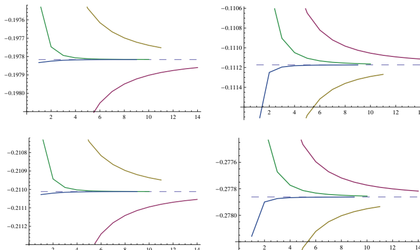
Figure 6. On the left column we plot the sequence \text{Re } f_{e,1}(\ell, z) as well as its Richardson transforms \text{Re } f_{e,1}^{(k)}(\ell, z) for k = 1, 2, 3 , and for \ell = 2 \cdots 14 . On the right column we plot the sequence \text{Re } f_{o,1}(\ell, z) as well as its Richardson transforms \text{Re } f_{o,1}^{(k)}(\ell, z) , again for k = 1, 2, 3 and for \ell = 2 \cdots 14 . The plots on the top are for z = 1/4 , and the plots of the bottom are for z = 1/8 . The dashed line shows the expected value \text{Re}(F_1(z) + \log \vartheta_{e,o}(z)) .
