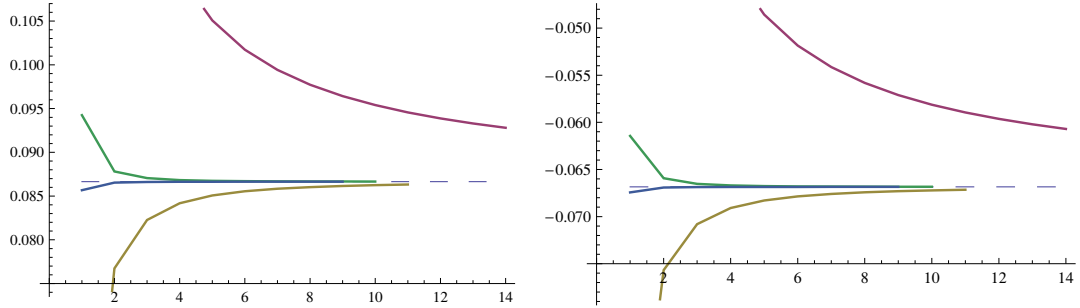
Figure 4. On the left column we plot the sequence \text{Re } f_e(\ell, z) as well as its Richardson transforms \text{Re } f_e^{(k)}(\ell, z) for k = 1, 2, 3 , and for \ell = 2 \cdots 14 . On the right column we plot the sequence \text{Re } f_o(\ell, z) as well as its Richardson transforms \text{Re } f_o^{(k)}(\ell, z) for k = 1, 2, 3 for \ell = 2 \cdots 14 . The plots on the top are for z = 1/4 , and the plots of the bottom are for z = 1/8 . The dashed lines in the plots show the expected value -\text{Re } F_0(z)/(\pi z)^2 .
