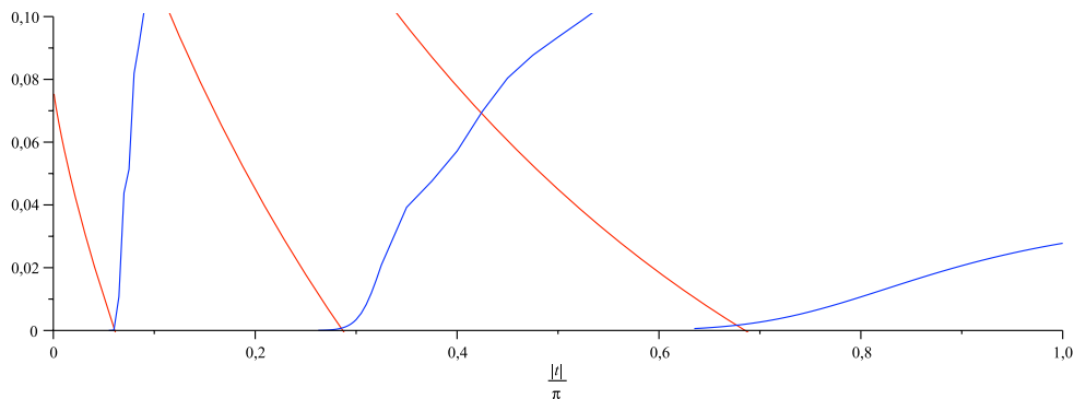
Figure 8. Plot of (4.32) (blue), calculated for N = 22 , and the real part of the instanton action (4.29) (red), as a function of |t|/\pi , for \theta = 9\pi/20, 7\pi/20 and \pi/4 , from left to right. The function (4.29) decreases monotonically until it becomes zero at |t|_c(\theta) . At this point, the average (4.32) gets triggered and it increases with |t| .
