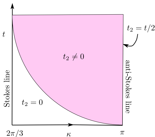
Figure 13. The phase diagram of the cubic matrix model (5.13) as a function of 2\pi/3 \leq \kappa \leq \pi and t = g_s N (which is taken to be real), for small t . The Stokes and anti-Stokes lines of the N = 1 case, which occur for \kappa = 2\pi/3 and \kappa = \pi , respectively, determine to a large extent the phase diagram for small t . On the anti-Stokes line, the saddle value of t_2 is t/2 , and the classical 1/N asymptotics requires corrections beyond the genus expansion.
