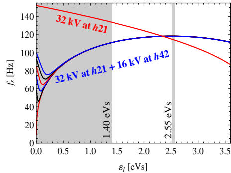
Figure 3: Synchrotron frequency versus single particle emittance for single and DH RF system (voltage ratio 0.5). A bunch of \varepsilon_l = 1.4 eVs covers the gray shaded area. A phase error of 0^0, 2^0, 4^0, 6^0, 8^0, 10^0 (from bottom to top trace) has been assumed between the two RF systems.
