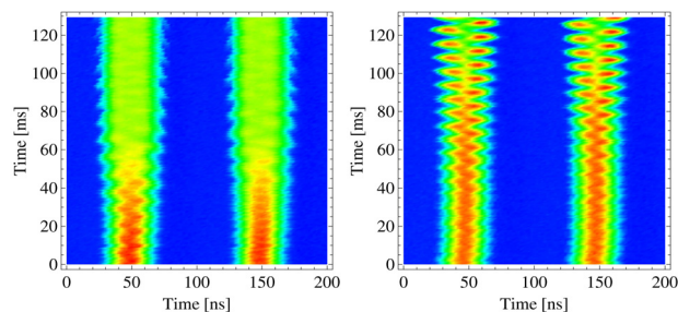
Figure 1: Last two bunches of the 18 bunch batch on the flat-top. The second harmonic ( h = 42 ) is increased to 16 kV within the first 70 ms (left). The SH case ( h = 21 only) is shown on the right plot.
