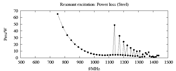
Figure 6: Resonant power loss versus the mode frequency.
