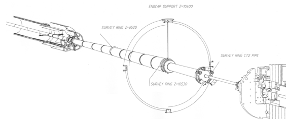
Figure 1: A 3D view of the CMS vacuum chamber. The beam pipe is shown from the interaction point to the compensation module.
