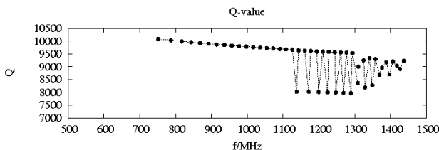
Figure 4: Plot of the Q-values of the monopole modes versus frequency for stainless steel.
