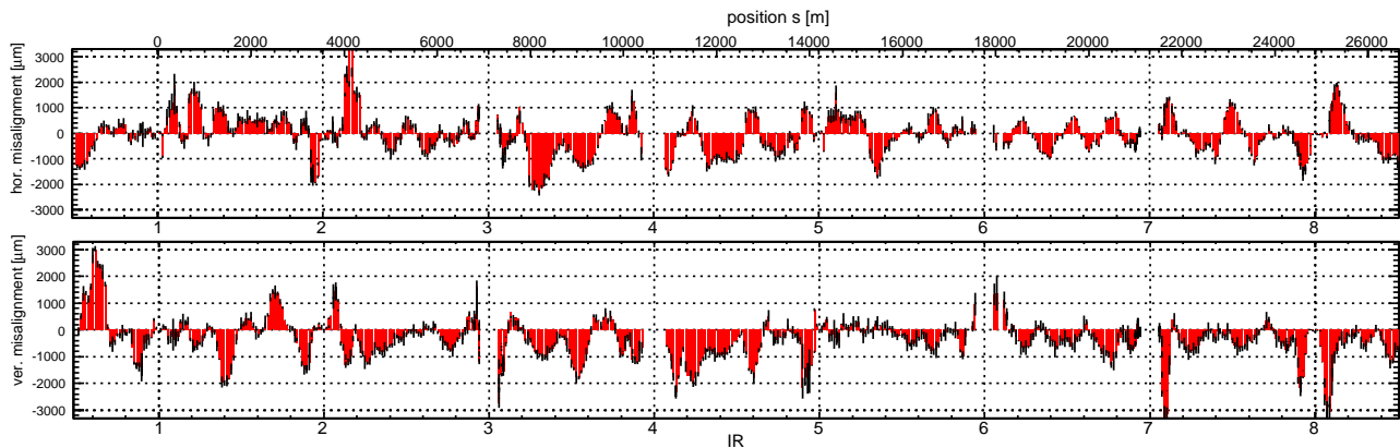
Figure 6: Beam-based quadrupole alignment estimate.
