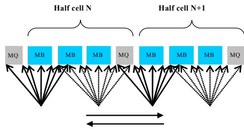
Figure 1: Vertical levelling sequence.
