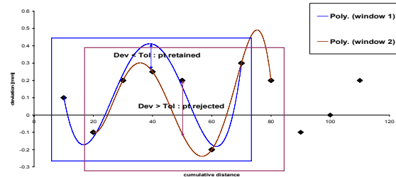
Figure 5: Windowing with PLANE.
