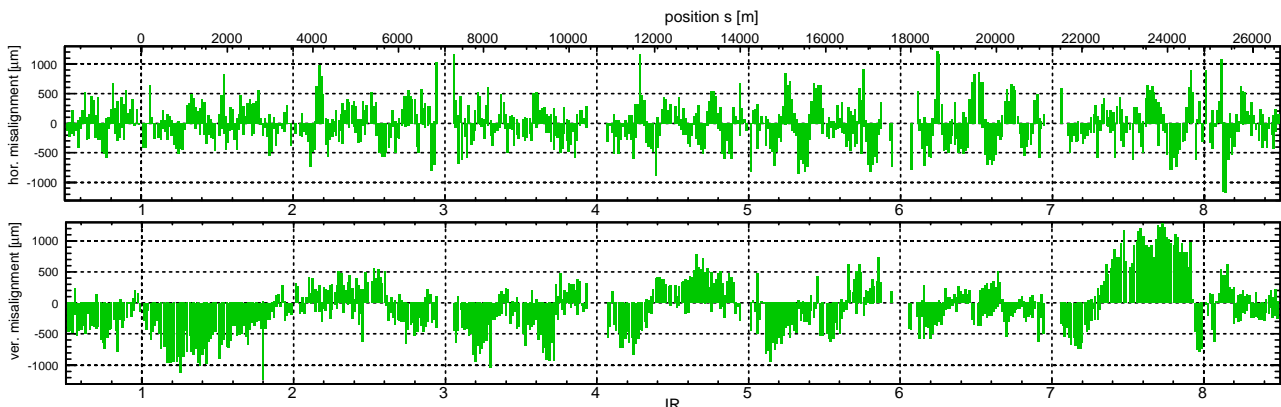
Figure 2: Horizontal and vertical magnet position deviation.
