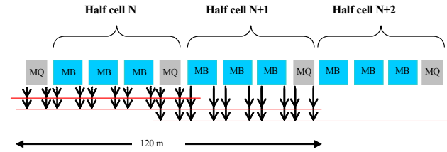
Figure 4: Horizontal offset sequence.
