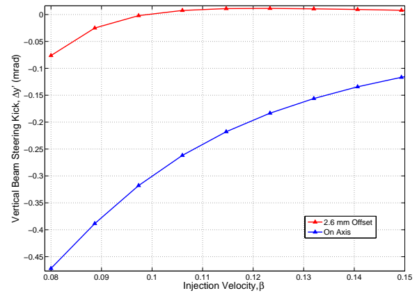
Figure 4: The compensation of a beam with A/q = 2.5 .
