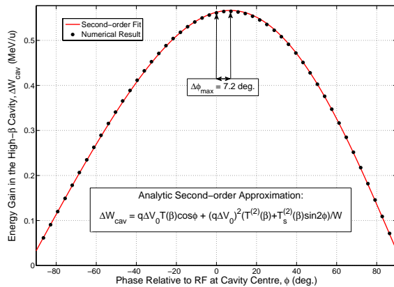
Figure 3: The energy gain as a function of phase for ions with A/q = 2.5 , injected into the high- \beta cavity at 8% of the speed of light.
