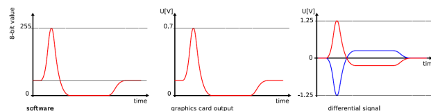
Figure 1: The desired pulse shape is created and mapped to the 8-bit output of the graphics card (left), which generates a single-ended unipolar signal (middle). To condition the signal for a specific task, gain and offset are adjusted, including the conversion to e.g. differential signals (right) [2].
