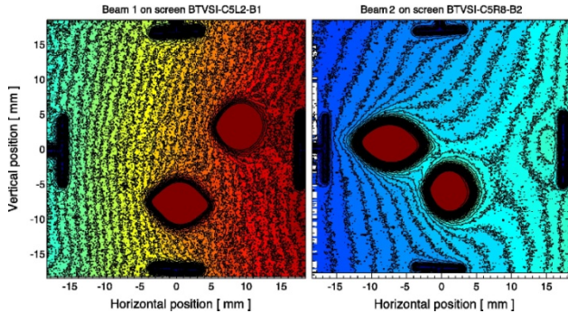
Figure 1: Beam screen (BTV) acquisitions that illustrate the very first turn of B1 (left) and B2 (right).
