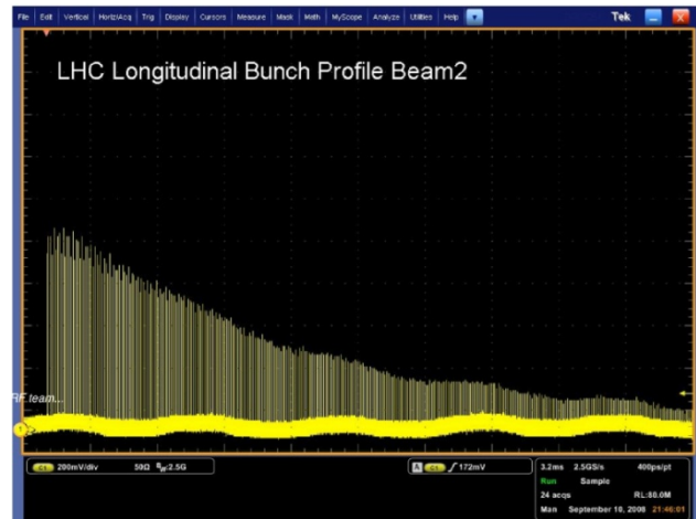
Figure 2: Longitudinal beam profile of the circulating, un-captured B2. Each vertical line represent one turn. Courtesy of RF team.
