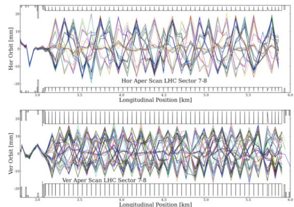
Figure 3: Measured horizontal (top) and vertical (bottom) beam trajectories during the aperture scans of arc 7-8 (Beam 2). The nominal machine aperture is also shown.
