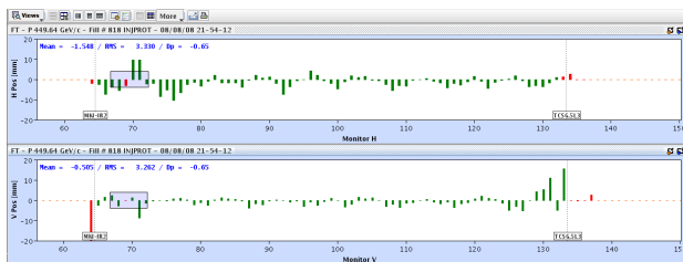
Figure 2: corrected trajectory in sector 23 shortly after injection of first beam and adjustment of SPS momentum.
