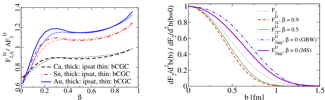
Figure 3: Left: nuclear modification of the diffractive structure function, showing characteristic suppression at small \beta (large mass of the diffractive system) and enhancement at large \beta . From Ref. [22]. Right: dominant impact parameters for the different contributions to the proton diffractive structure function.
