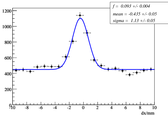
Figure 4: Residual of clusters in TTbX to IT Bottom tracks. The result of a fit to a Gaussian signal combined with a flat background is superimposed.
