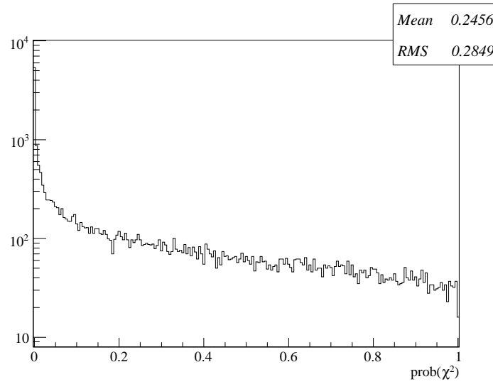
Figure 2: Probability of \chi^2 for reconstructed tracks.
