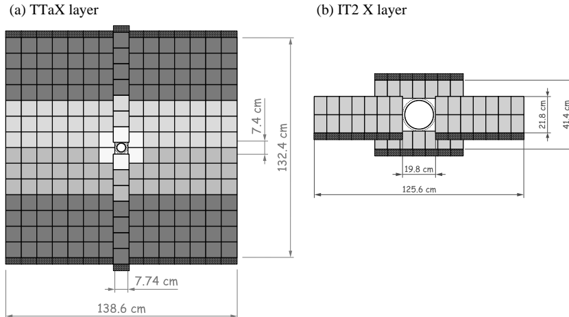
Figure 1: Layout of (a) the x layer in TTa and (b) a x layer in IT station 2.
