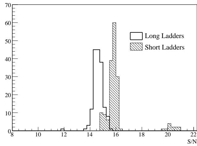
Figure 3: Measured S/N of the Inner Tracker ladders.
