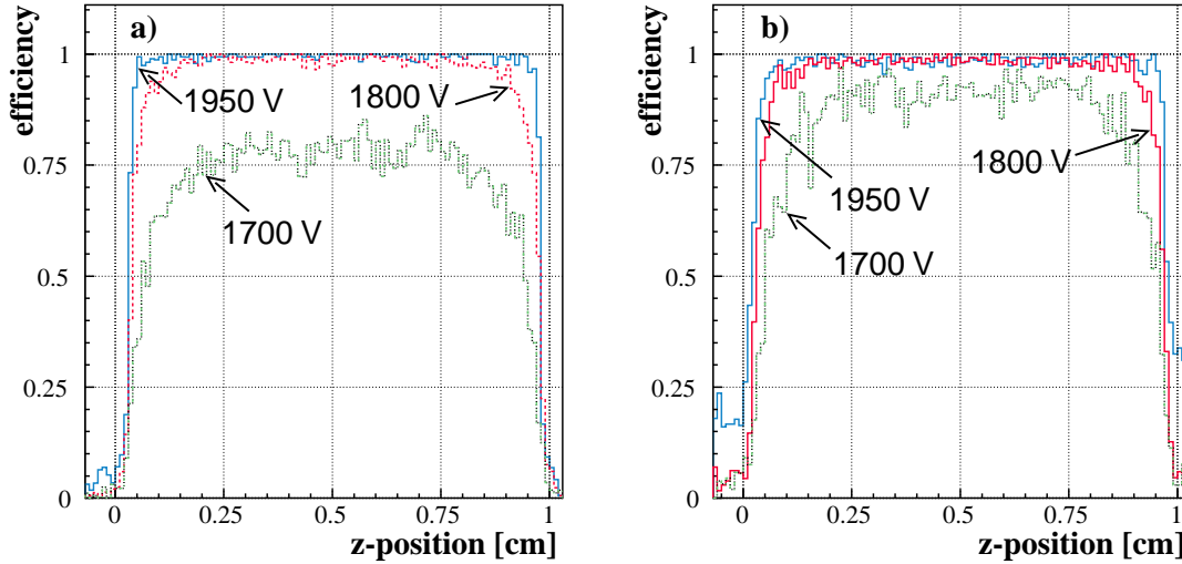
Figure 3.13: Efficiency as function of drift distance z for the a) ASD8b and b) MADIV, at three different gas gains. (The wire position is at 0.5 cm).
