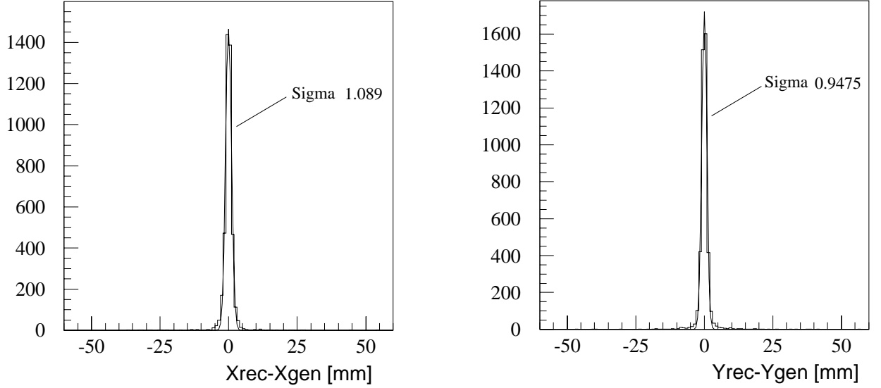
Figure 4.20: Simulated spatial resolution of ECAL2 for x and y coordinates. x_{gen}, y_{gen} and x_{rec}, y_{rec} refer to the generated ( gen ) and reconstructed ( rec ) x, y coordinates.
