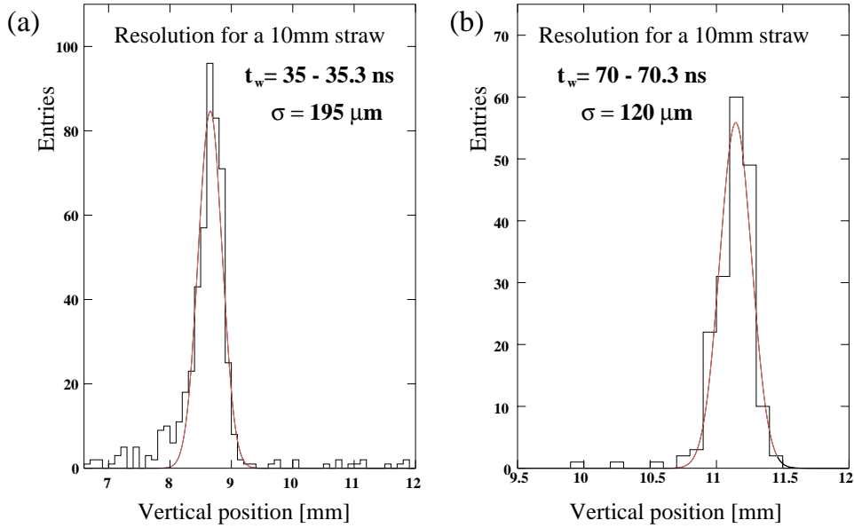
Figure 3.31: Resolution for a 10 mm straw for a time window of (a) 35-35.3 ns (b) 70-70.3 ns.
