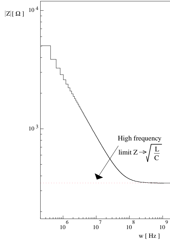
Figure 3.10: Impedance versus frequency for a 10 mm straw. The dashed lines shows the high frequency limit.
