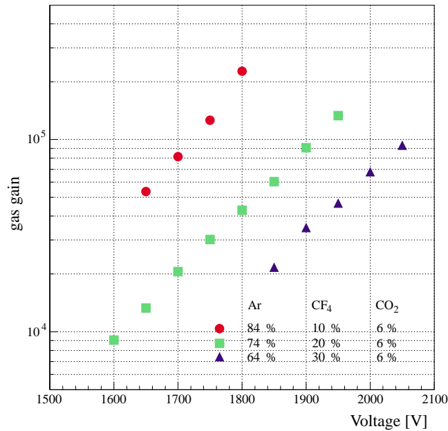
Figure 3.6: Measured gas gain versus wire voltage for an 8 mm diameter straw using the gas mixture Ar/CF 4 /CO 2 at different percentages.
