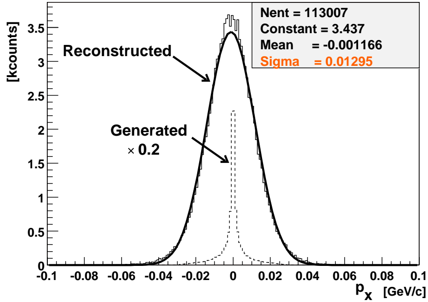
Figure 4.23: x component of the transverse transfer momentum. It is the sum of the x components of the momenta of the scattered \pi^- and \gamma [70].
