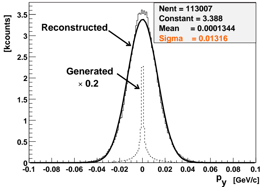
Figure 4.24: y component of the transverse transfer momentum. It is the sum of the y component of the momenta of the scattered \pi^- and \gamma [70].
