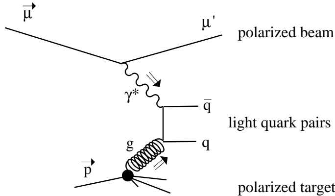
Figure 2.2: The photon-gluon fusion diagram for q\bar{q} production.
