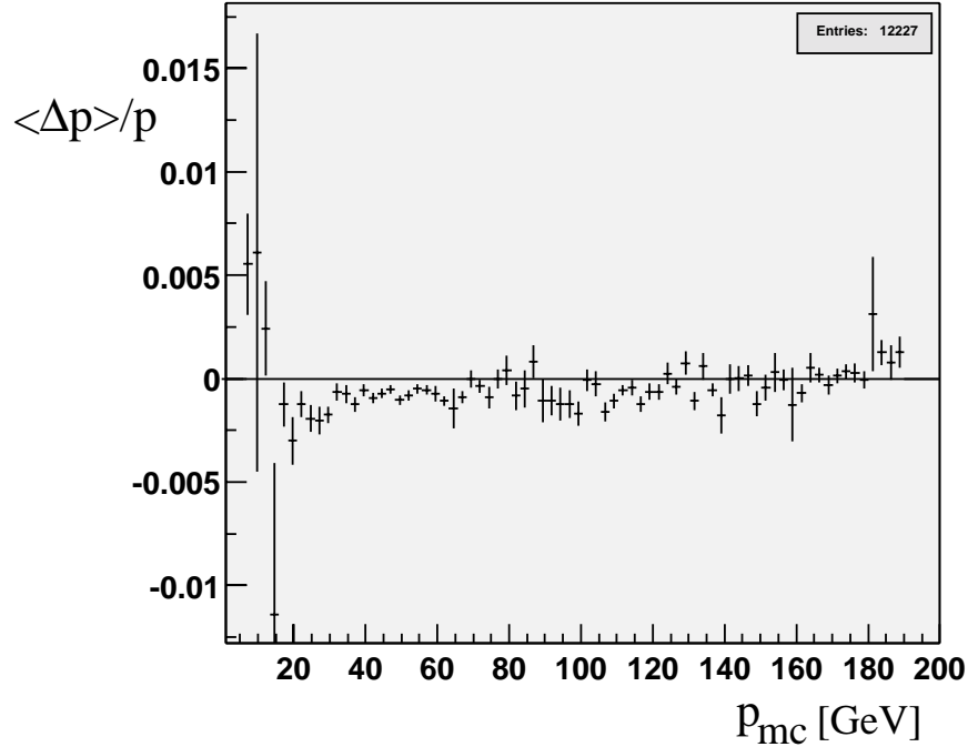
Figure 4.17: Reconstruction error for the momentum of a pion [70].
