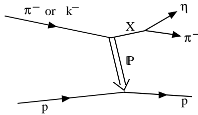
Figure 1.2: Single diffractive dissociation of the projectile.
