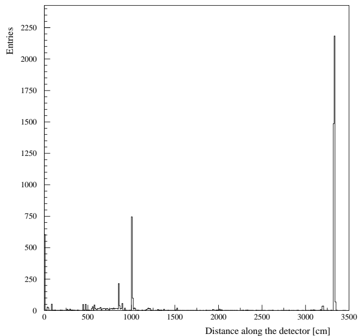
Figure 4.14: Position of the conversion of the gammas created in the \eta decay generated with the diffractive event generator.
