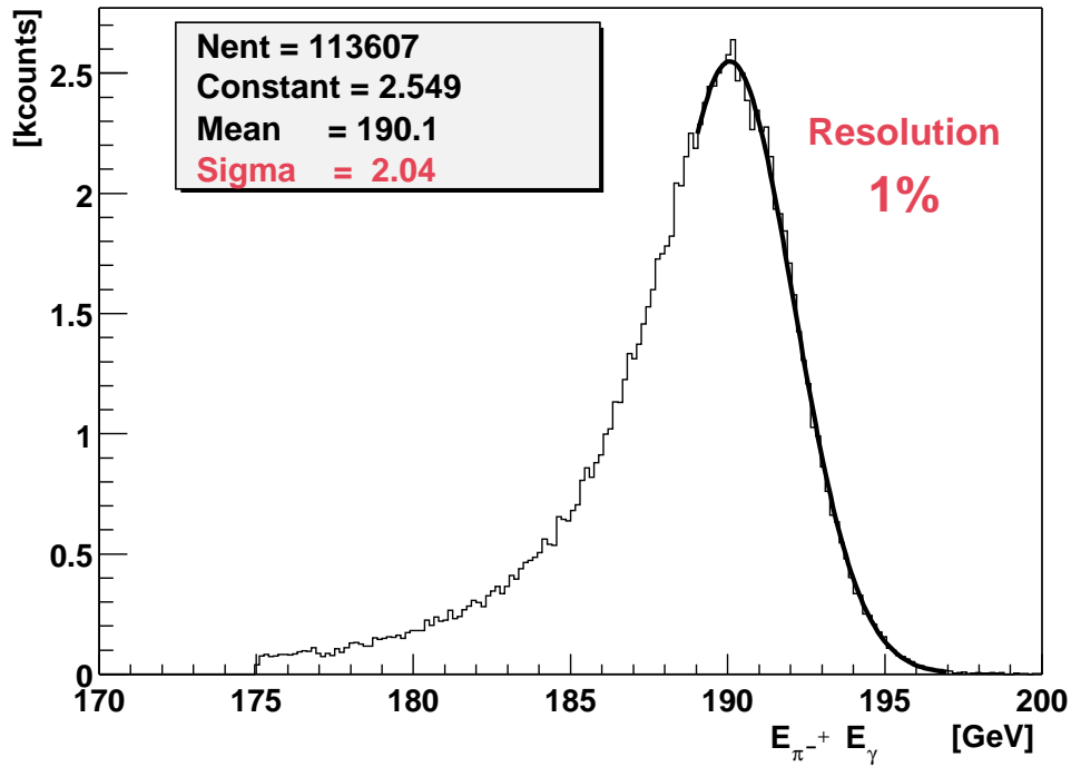
Figure 4.21: Sum of the energies of \pi^- and \gamma , corresponding to the energy of the intermediate state (Monte Carlo simulation, including reconstruction, in COMPASS) [70].
