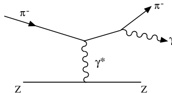
Figure 1.3: Primakoff reaction.
