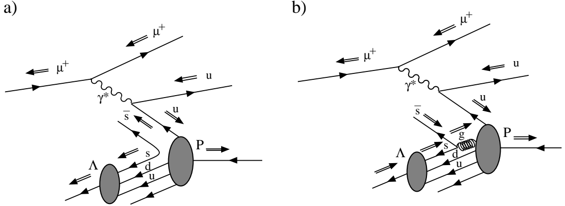
Figure 2.3: \Lambda polarization arising from a) polarized strange quarks, b) polarized gluons. The thicker arrows represent the spins of the particles.
