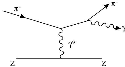
Figure 2.4: Pion radiative scattering in the Coulomb field of a nucleus
