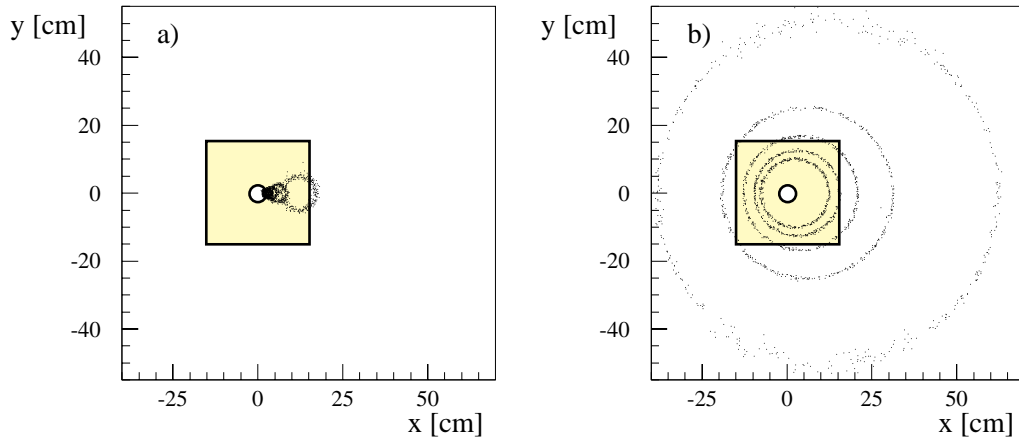
Figure 4.10: Spatial distributions at 1507 cm from the target for a) Primakoff pions and b) diffractively produced pions. The coloured box corresponds to the GEM detector. The insensitive region of the detector is also indicated at the centre. The boundaries of the MWPC are larger than the plot, thus they are not shown.
