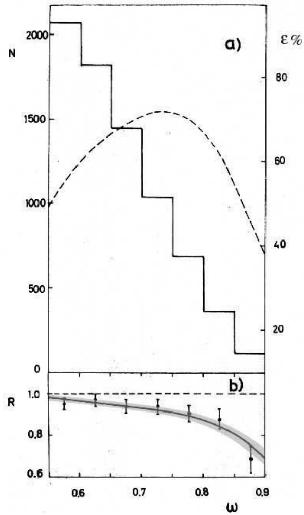
Figure 4.33: a) Distribution of the Primakoff events over the variable \omega = E_\gamma/E_{tot} . The discontinuous line is the detection efficiency; b) The \omega dependence of R = (d\sigma/d\omega)^{exp}/(d\sigma/d\omega)_{\alpha_\pi=0}^{theor} . The solid curve illustrates the results of the fit of the experimental data to the theoretical distribution with a polarizability \alpha_\pi = 6.1 \cdot 10^{-43} \text{ cm}^3 . The grey shadowed region represents the width of the errors that can be obtained with the COMPASS measurement.
