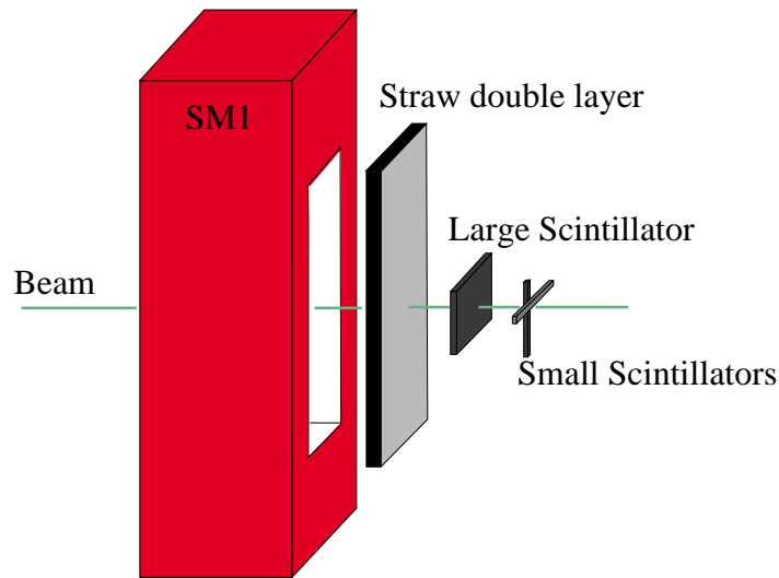
Figure 3.18: Setup for the rate measurements performed in September 1999 at the M2 beam line at the SPS at CERN.
