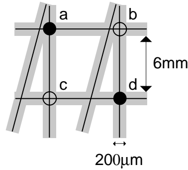
Figure 3.2: a and d are the real hits. b and c are not real hits. The black lines represent the measured coordinates and the grey areas correspond to the resolution of the straws.
