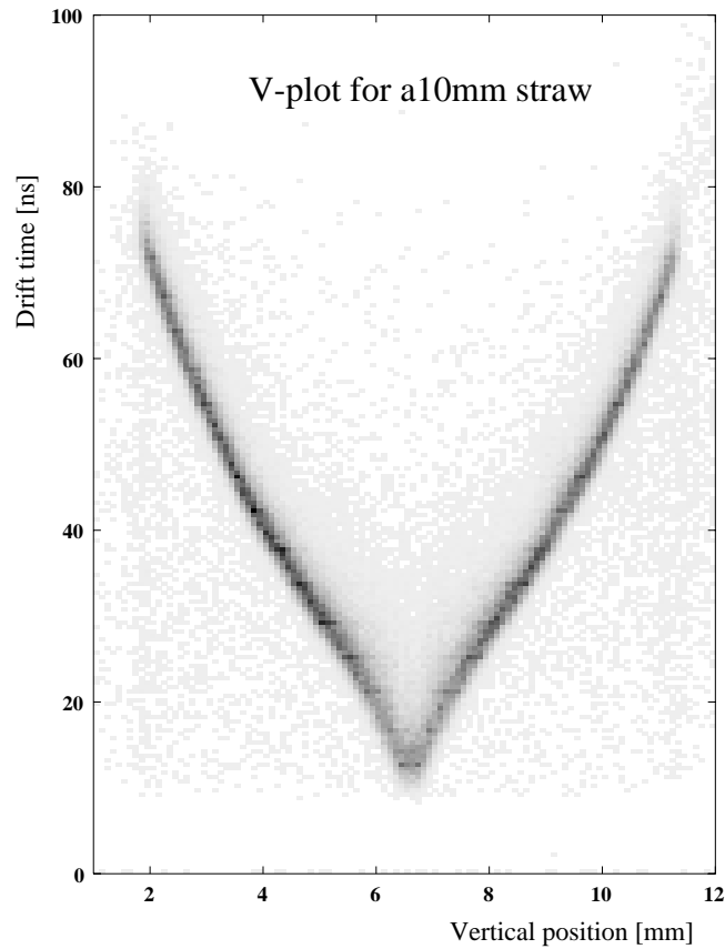
Figure 3.28: V-plot for a 10 mm straw.
