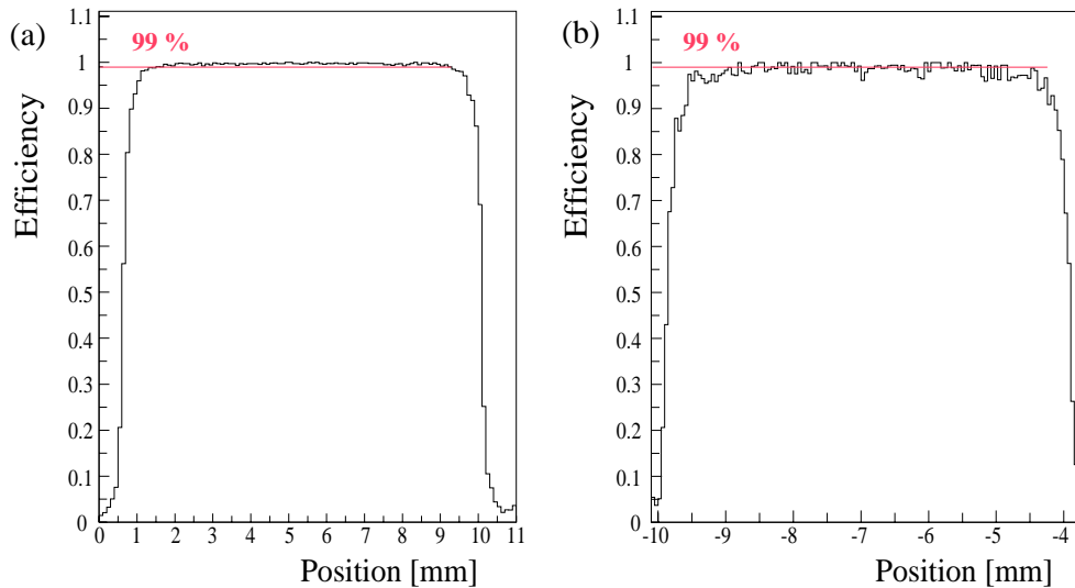
Figure 3.35: (a) Efficiency for a 10 mm straw and (b) Efficiency for a 6 mm straw.
