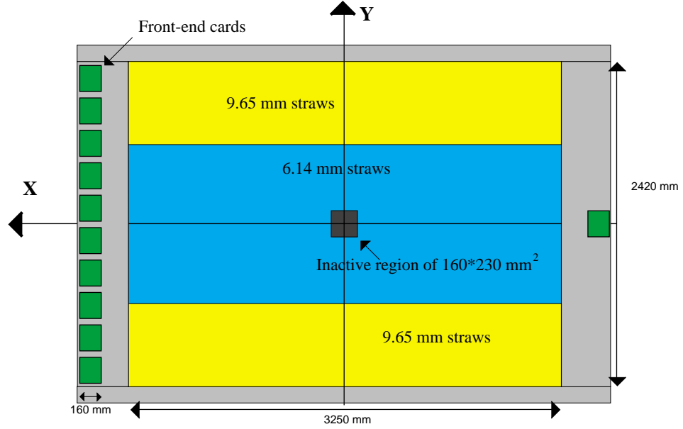
Figure 3.4: Horizontal straws, Y-plane.
