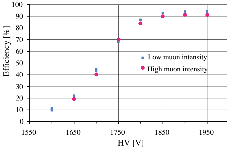
Figure 3.20: Efficiency versus high voltage for high and low intensity muon beam.
