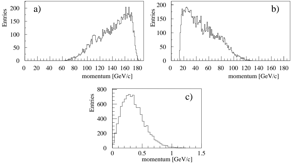
Figure 4.3: Total momentum for a) outgoing \pi^- , b) \eta and c) p of diffractive events.
