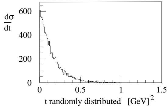
Figure 4.2: Simulated differential cross-section for diffractive dissociation as a function of t .
