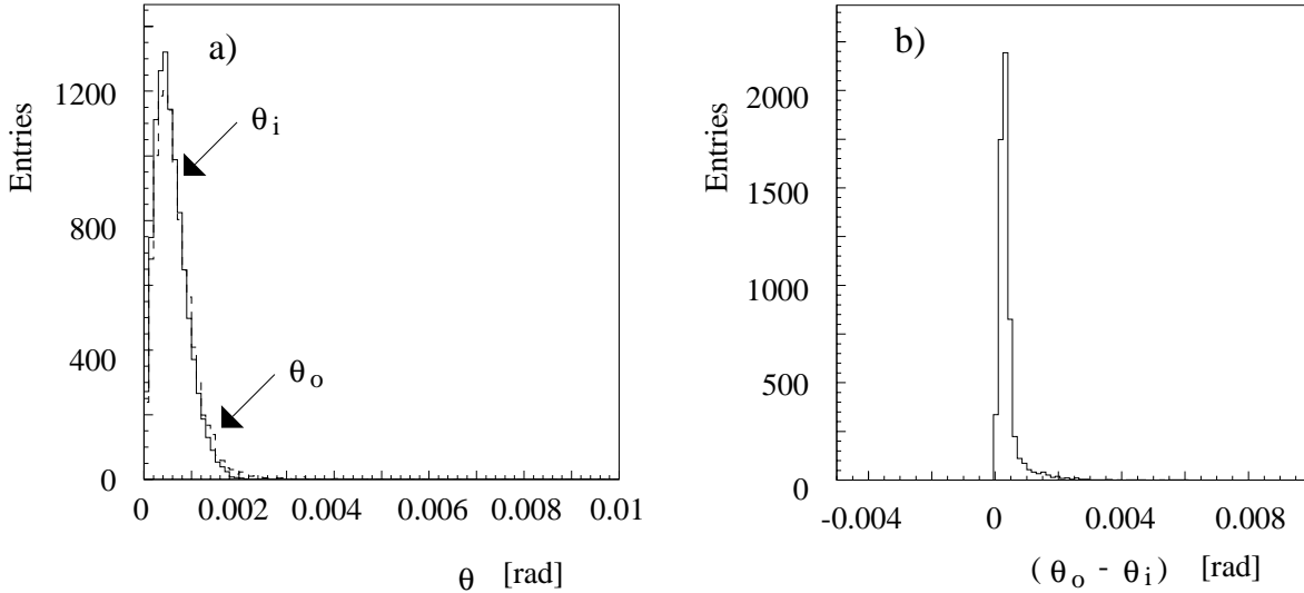
Figure 4.7: Primakoff reaction: a) polar angles \theta_i of the incoming \pi^- and \theta_o of the outgoing \pi^- . b) scattering angle \theta_o - \theta_i of the outgoing \pi^- .
