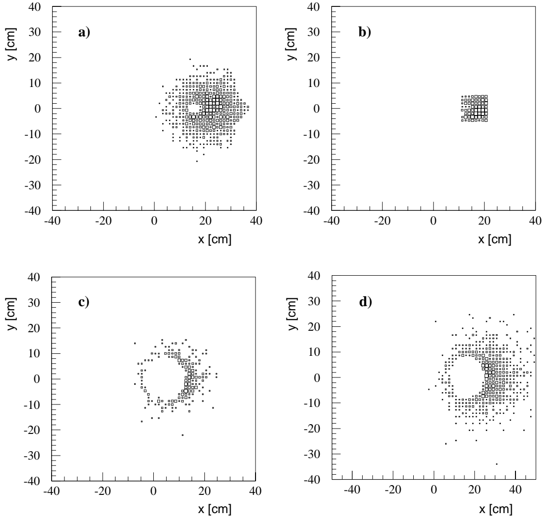
Figure 4.16: Pion hits positions at different places in the detector after SM2. These pions belong to the events where the eta decays into two gammas. a) Pion hits at the GEM 5, 31.7 m away from the target b) Pion hits at 31.5 m from the target, at the scintillating fibre station 8, c) Pion hits at 20.20 m from the target in MWPCA 5 d) Pion hits in MWPCA6 at 31.8 m.
