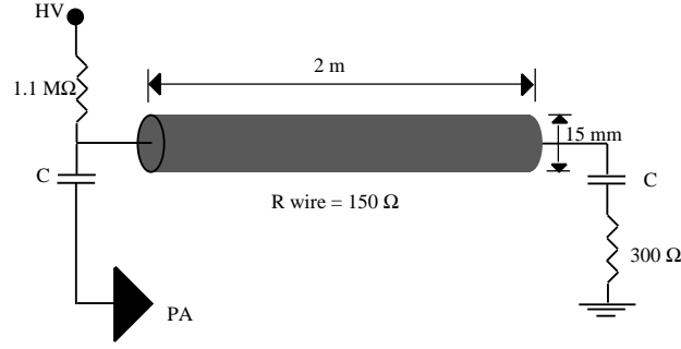
Figure 3.8: Setup for the test of the 4 straws from Dubna.
