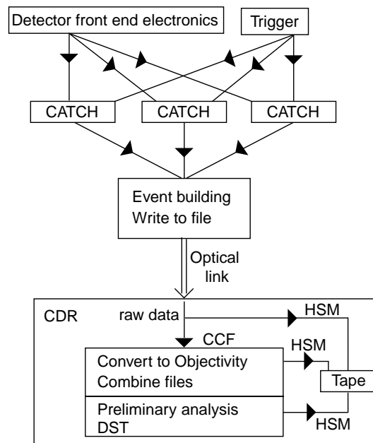
Figure 2.6: COMPASS data acquisition scheme.
