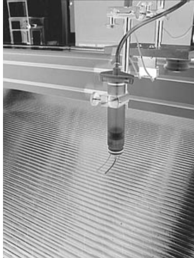
Figure 3.46: Gluing the plane of straws.
