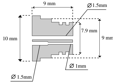
Figure 3.16: Endplug specially designed for a prototype. One hole is for the pin which will centre the wire and the other one, with two different diameters, is for the gas connection.
