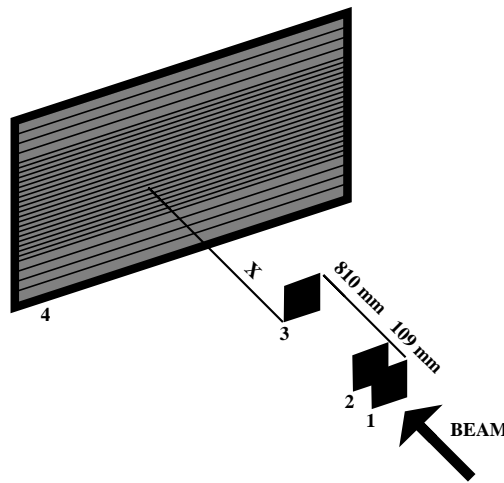
Figure 3.25: Test beam setup. 1, 2, 3 are the different planes of the silicon detector. The distance was 109 mm between 1 to 2 and 810 mm between 2 and 3. 4 is the prototype, and its distance from the silicon plane number 3 was X = 901 \text{ mm} for the Dubna prototype and X = 521 \text{ mm} for the Moscow prototype.
