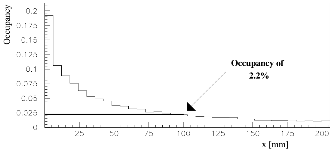
Figure 3.24: Simulated occupancy at different distances to the beam centre. The value of 2.2% is obtained for 100 mm which will be the distance at which will be situated the straw from the beam centre.
