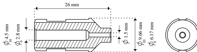
Figure 3.44: Side and front view of an end-plug. All the dimensions are equal for the 6 mm and the 10 mm straws, except for the dimensions which have a subindex which indicates to which straw diameter they belong to.
