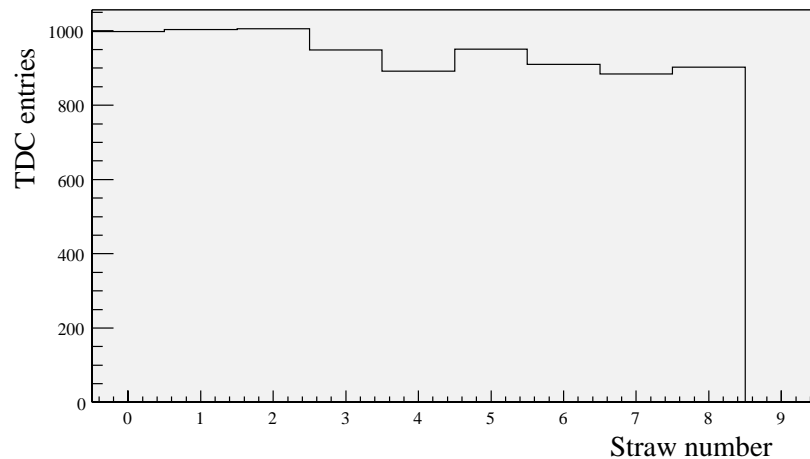
Figure 3.39: Profile of the beam given by the counts in the straws.
