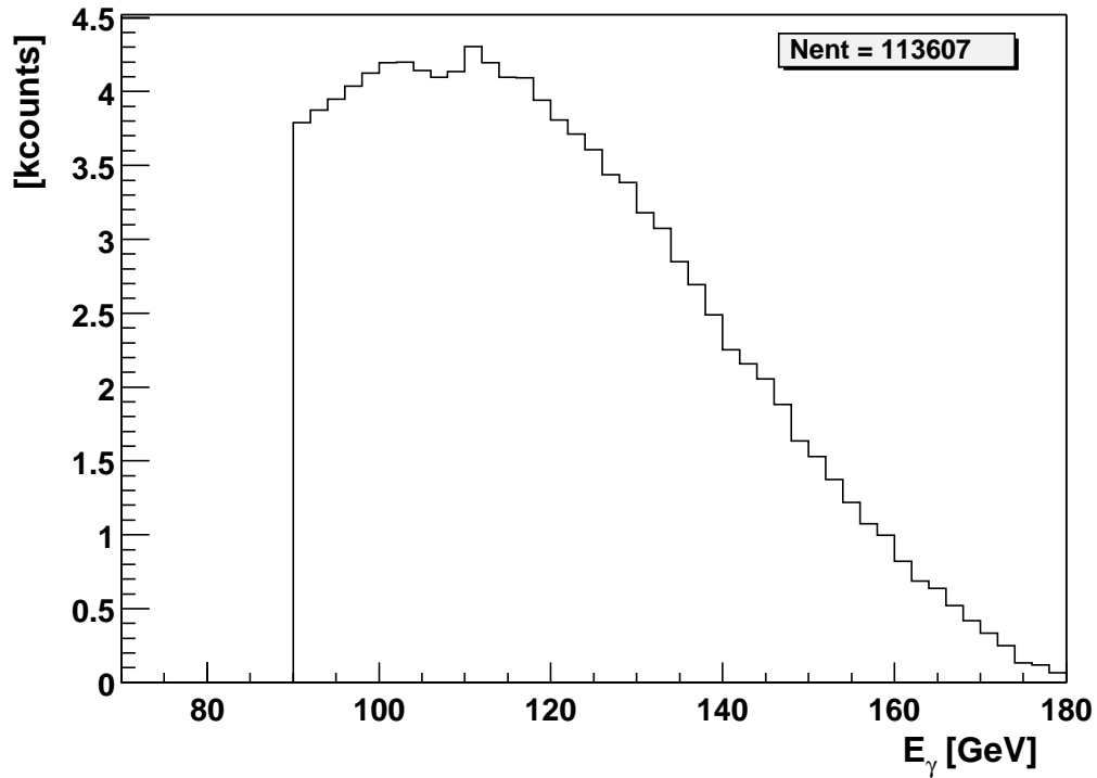
Figure 4.28: Gamma energy distribution [70].
