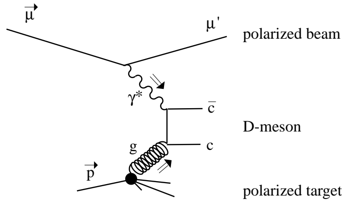
Figure 2.1: The photon-gluon fusion diagram for c\bar{c} production.
