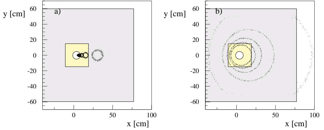
Figure 4.11: Spatial distributions at 1987 cm from the target for a) Primakoff pions and b) diffractively produced pions. The large coloured box corresponds to the MWPCA detector and the small coloured box corresponds to the GEM detector. The insensitive region of the GEM detector is also indicated in its centre, but the insensitive region of the MWPCA is not indicated since that area is covered by the GEM.
