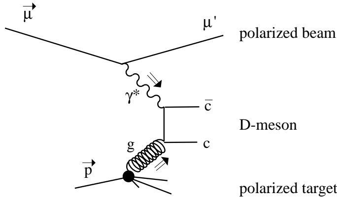
Figure 1.1: The photon-gluon fusion diagram for c\bar{c} production.
