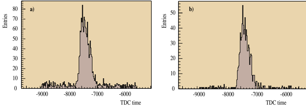
Figure 3.40: TDC spectra for 2 channels a) for a noisy channel and b) for a working channel without problems.
