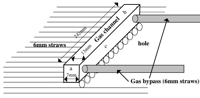
Figure 3.45: Sketch of the physical hole.
