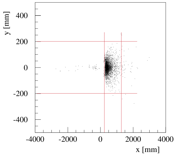
Figure 4.32: Simulated hit distribution of the scattered pion at 30 m from the target. The lines indicate the possible size of the trigger hodoscope.
