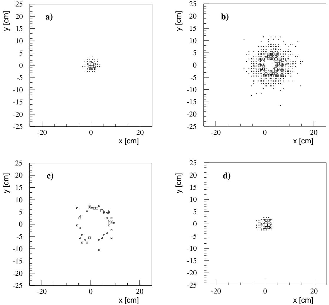
Figure 4.15: Hit positions of the pion at different places in the detector between SM1 and SM2. These pions belong to the events where the \eta decays into two gammas. a) Pions at the silicon station 4, 4.5 m away from the target b) Pions at 15.21 m from the target, (old position of the GEM station 3) c) Pions at 9.25 m from the target, at a MWPCA detector and d) Pions at 13.08 m at the scintillating fibre station 6.
