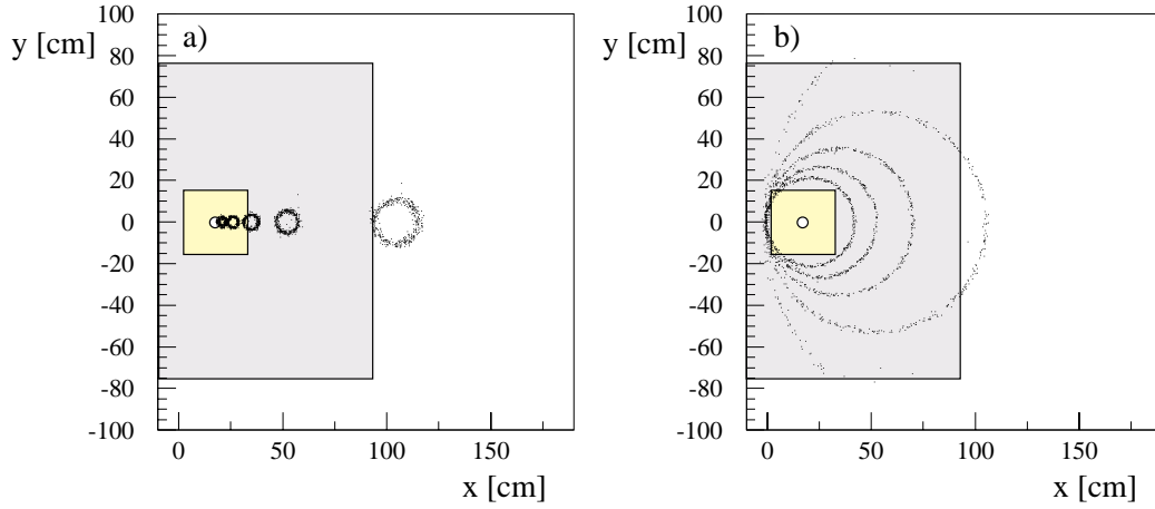
Figure 4.12: Spatial distributions at 3200 cm from the target for a) Primakoff pions and b) diffractively produced pions. The big coloured box corresponds to the MWPCA detector and the small coloured box corresponds to the GEM detector. The insensitive region of the GEM detector is also indicated in its centre, but the insensitive region of the MWPCA is not indicated since that area is covered by the GEM.
