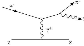
Figure 4.5: Pion radiative scattering in the Coulomb field of a nucleus.
