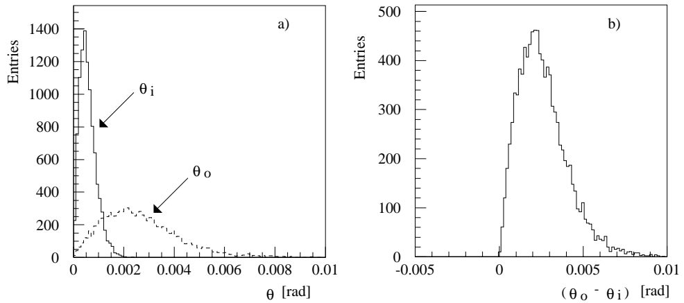
Figure 4.4: Diffractive dissociation: a) polar angles \theta_i of the incoming \pi^- and \theta_0 of the outgoing \pi^- . b) scattering angle \theta_0 - \theta_i of the outgoing \pi^- .
