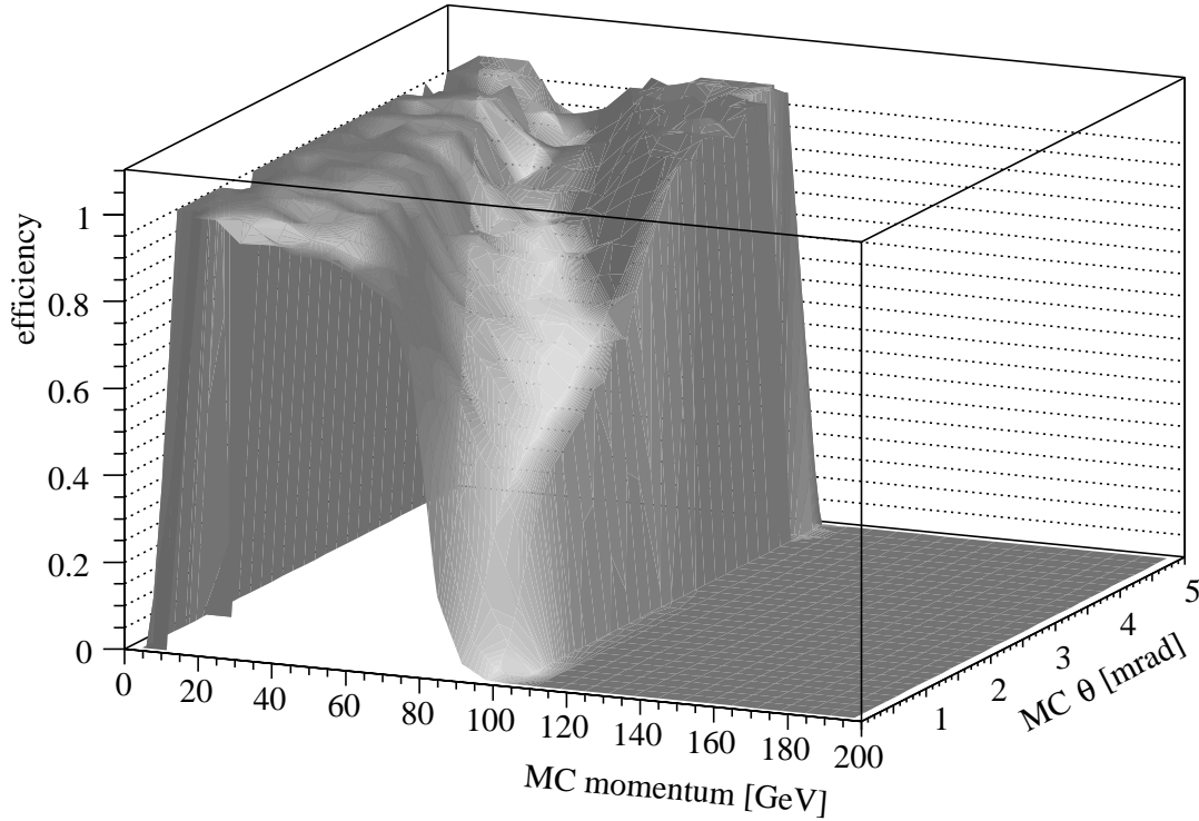
Figure 4.18: Reconstruction efficiency for the pions for different pion momenta and theta angles [70]. The efficiency is computed as the number of reconstructed pion tracks divided by the number of generated pion tracks. A hole in the acceptance of the detector is visible for small \theta angles and large longitudinal momenta and for large \theta angles and small longitudinal momenta.
