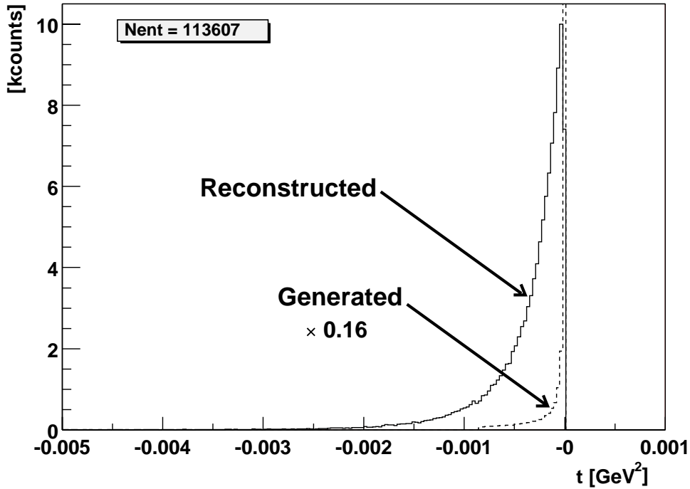
Figure 4.26: t distribution of generated events and of the reconstructed events in the COMPASS detector [70].
