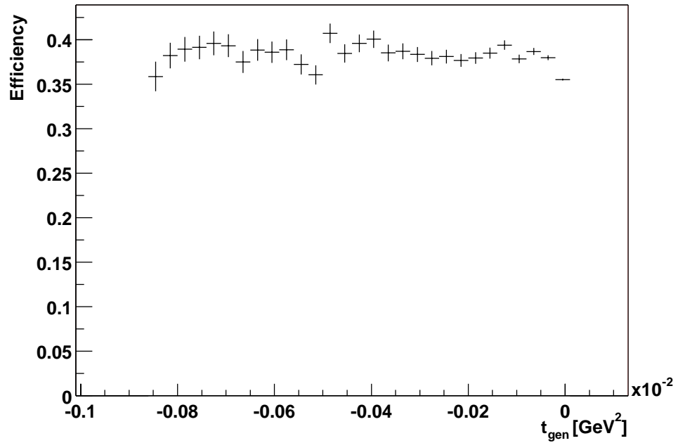
Figure 4.30: Efficiency versus the four momentum transfer squared t [70].
