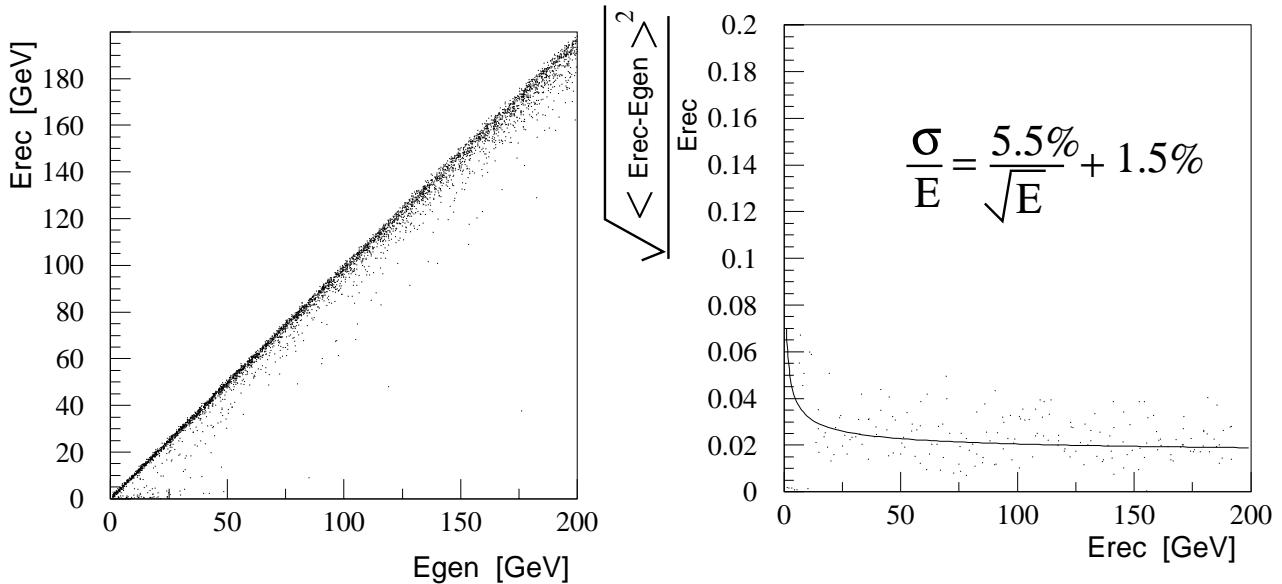
Figure 4.19: The left plot shows the energy of the reconstructed gamma versus the energy of the generated gamma. The right plot shows sigma versus the reconstructed energy. The curve running through the points indicates the predicted behaviour.
