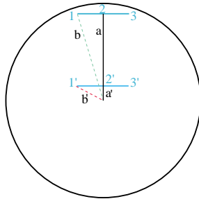
Figure 3.32: Ionisation path needed to produce enough electron ion pairs for the signal development, close the wire (from point 1 to point 3) or close to the wall (from point 1' to point 3') (see text).
