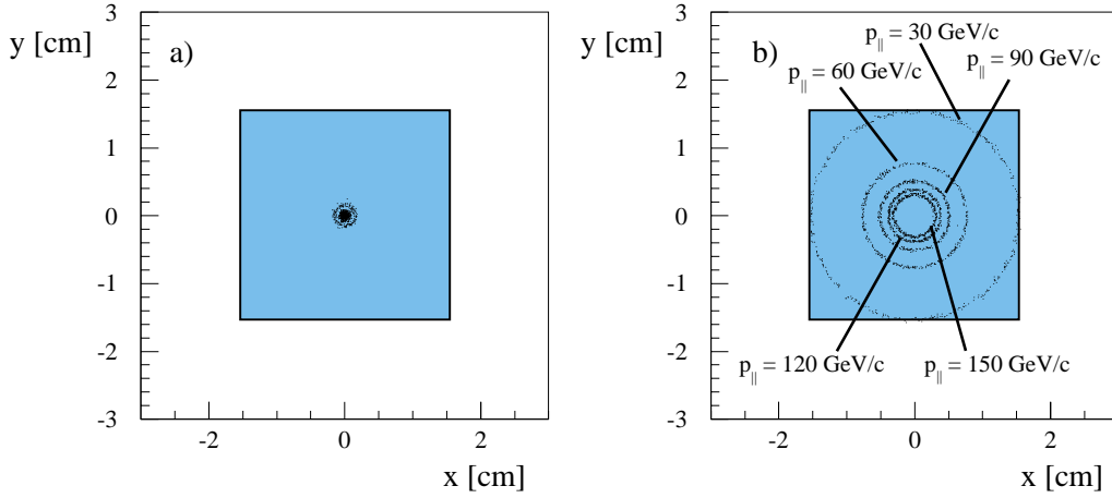
Figure 4.9: Hit distributions at 46 cm from the target for a) Primakoff pions and b) diffractively produced pions. In b) the different longitudinal momenta are indicated. The coloured box refers to the size of the silicon detector.
