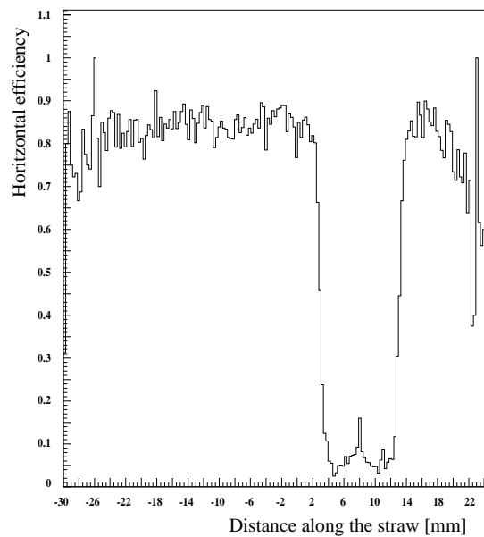
Figure 3.37: Efficiency in the region of the spacer as a function of the hit position along the wire for a 10 mm straw.
