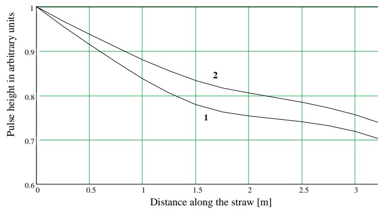
Figure 3.15: Pulse height simulation as a function of the source position along the straw. Diameter of the straw: 6 mm. Number 1 is the straw with carbon coated Kapton, as those used in the prototypes built in JINR and MSU. Number 2 is the straw with Kapton XC with aluminized mylar.
