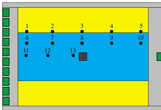
Figure 3.41: Measuring points in the chamber. These points were chosen to study the homogeneity of calibration.
