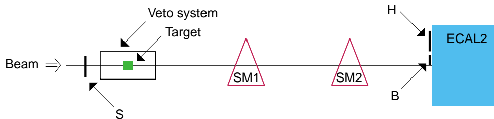
Figure 4.31: Trigger setup for the Primakoff measurement in COMPASS. It consists of a beam counter ( S ), beam veto counter ( B ), a hodoscope ( H ), a veto system around the target and the electromagnetic calorimeter ( ECAL2 ).
