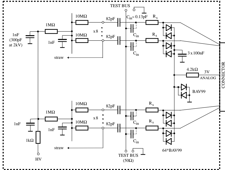
Figure 3.11: Circuit diagram of the motherboard that will be used in the straw chambers of TS2 [55].
