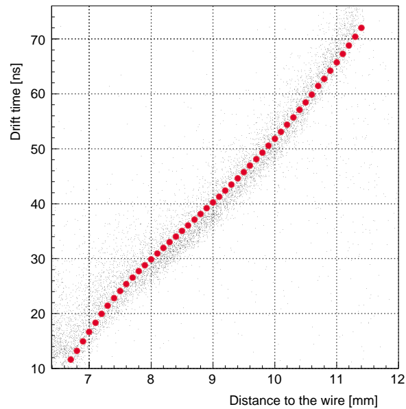
Figure 3.29: One of the V-legs for a 10 mm straw. The dots in gray correspond to the simulated r(t) relation using the GARFIELD simulation package.
