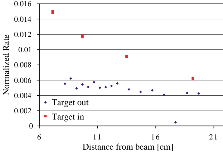
Figure 3.22: The figure shows the measurement of the normalized rate for the hadron beam for two different conditions, when the target is in or out (the SM1 magnet is switched off).
