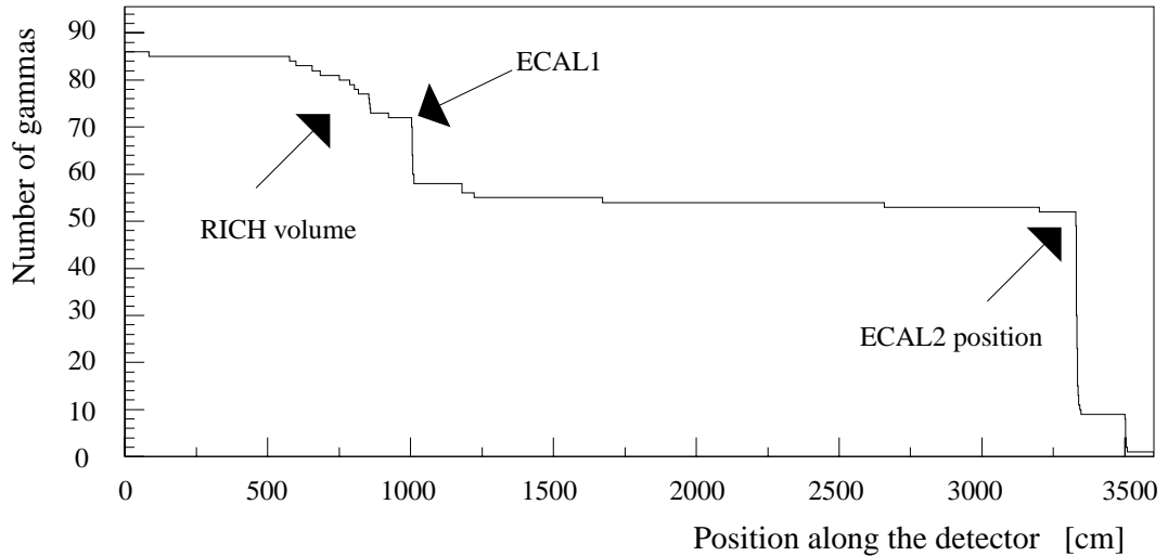
Figure 4.8: Number of gammas at different positions along the detector. In the region of the RICH as well as in the position of the ECAL1, a large amount of gammas is converted. ECAL1 has a large hole, thus only gammas with large angles will be converted there. At the ECAL2 position almost all remaining gammas are converted except for those that escape through the hole of the ECAL2 and those with angles larger than the acceptance of the ECAL2.
