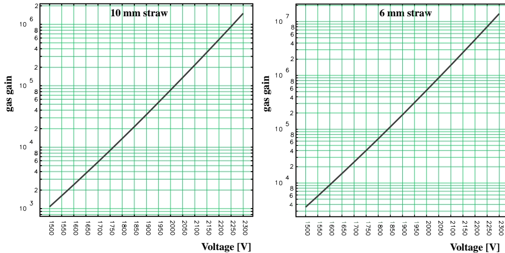
Figure 3.7: Simulated gas gain versus wire voltage for 10 mm and 6 mm straws using the gas mixture \text{Ar}/\text{CF}_4/\text{CO}_2 (74:20:6).
