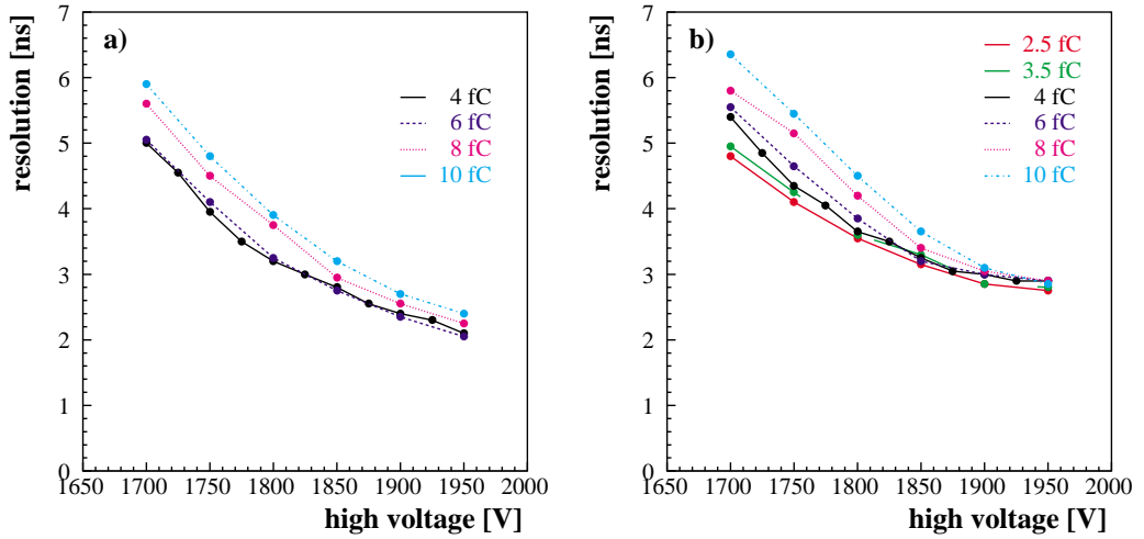
Figure 3.12: Convoluted time resolution of two straws as a function of the high voltage settings and of the different thresholds of the discriminators for the a) ASD8b and b) MADIV.
