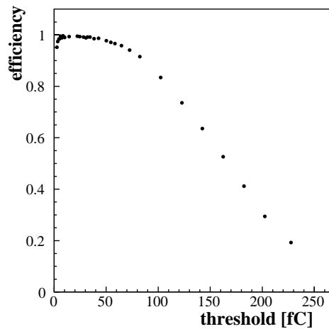
Figure 3.14: Efficiency at a drift distance of 1 \text{ mm} \leq r \leq 2 \text{ mm} measured with the ASD8b at 1950 V.
