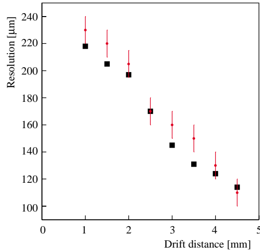
Figure 3.34: Comparison of simulated (squares) and measured resolution (dots) for a 10 mm straw at various drift distances to the wire.
