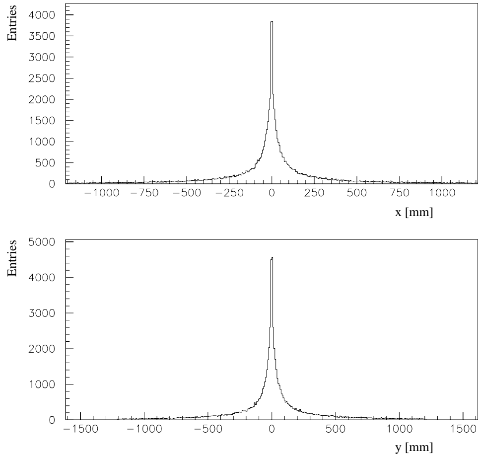
Figure 3.23: Simulated particle distributions in a chamber plane in the x -direction and in the y -direction.
