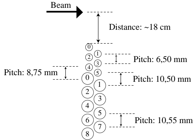
Figure 3.38: Straws layout for the pilot run of COMPASS.
