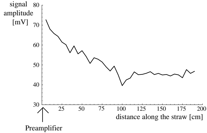
Figure 3.9: Measurement of the attenuation length. At about 100 cm the signal is smaller due to the presence of the spacer.
