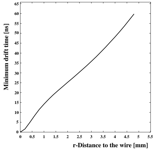
Figure 3.5: r(t) relation for a 10 mm straw with no magnetic field using Ar/CO 2 /CF 4 74:6:20 as gas mixture.
