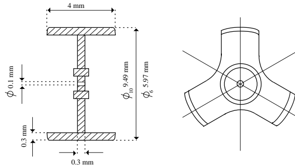
Figure 3.43: Side and front view of a spacer. The dimensions are equal for the 6 mm and the 10 mm straws, except for the dimensions which have a subindex indicating to which straw diameter they belong to.
