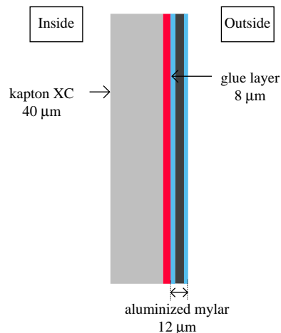
Figure 3.42: Schematic layout of the straw wall.
