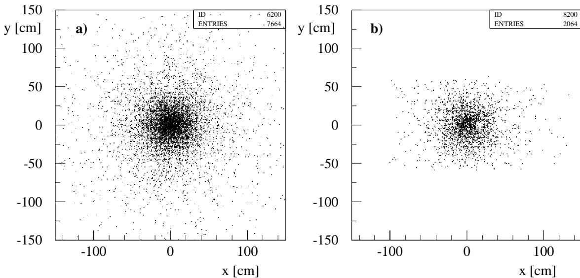
Figure 4.13: a) Spatial distribution of the gammas generated from the \eta decay extrapolated to the position of ECAL2 and b) Hits generated by the conversion of \eta decay.
