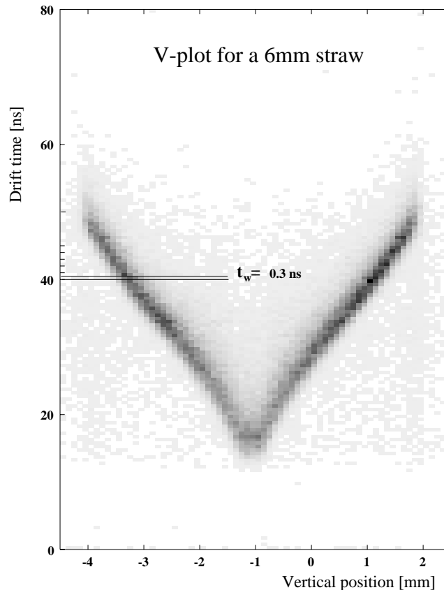
Figure 3.30: V-plot for a 6 mm straw.
