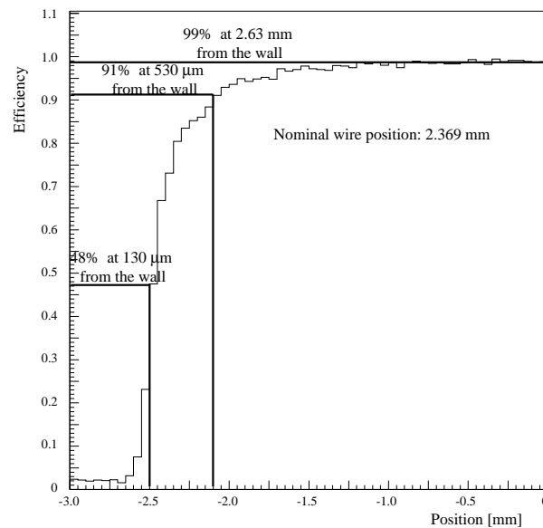
Figure 3.36: Efficiency for a 10 mm straw near the wall.
