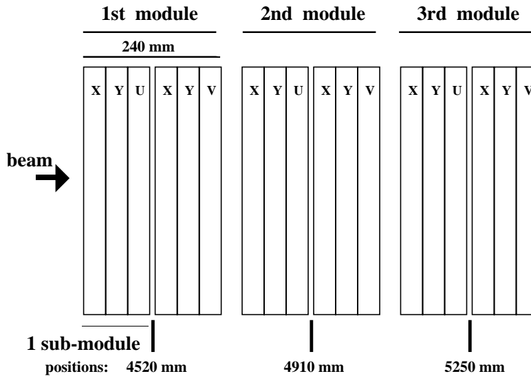
Figure 3.3: Schematic layout of the tracking station 2. The positions of the different modules along the COMPASS detector are indicated.
