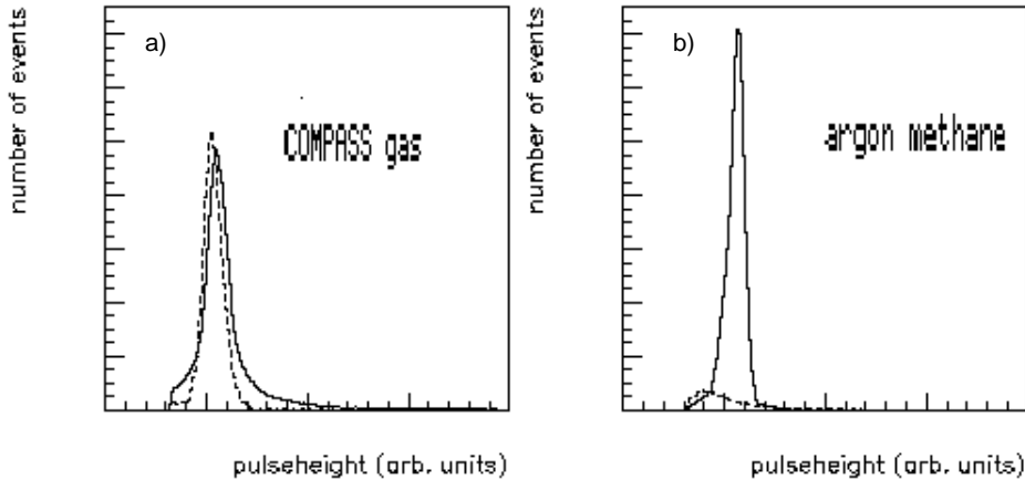
Figure 3.17: Pulseheight spectra before (solid lines) and after (1.1 C/cm, dotted lines) proton irradiation for two different gases a) the COMPASS gas and b) argon methane. The spectra was taken using an 55 Fe source.
