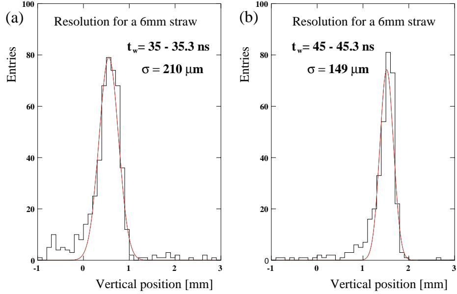
Figure 3.33: Resolution for a 6 mm straw for a time window of (a) 35-35.3 ns (b) 45-45.3 ns.
