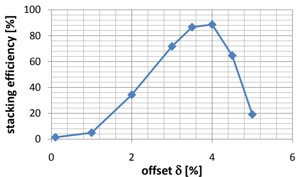
Figure 3: Simulated stacking efficiency for the CLIC-PDR vs. the momentum offset at injection, \delta_{\text{off}} , for z_{\text{off}} = 10 mm. Each bunchlet is represented by 5 macroparticles.
