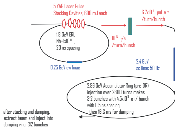
Figure 1: Schematic of CLIC CERL Compton source including typical yields at various steps of the e^+ generation.
