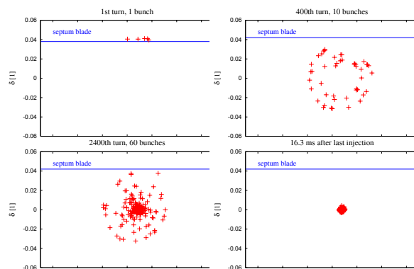
Figure 4: Phase-space snapshots for CLIC-PDR stacking process: first bunchlet on first turn (top left), 10 bunchlets on turn 400 (top right), 60 bunches on turn 2400 (bottom left), and 16.3 ms after last injection (bottom right). The blue line indicates the location of the septum blade.
