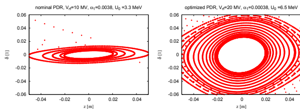
Figure 2: Longitudinal phase space of the CLIC PDR design (left) and stacking-optimized version (right).
